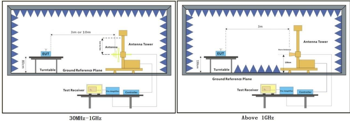
30MHz-1GHz
