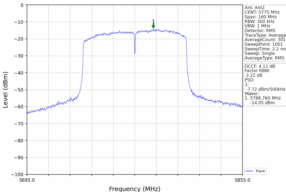
802.11ac(VHT80)_MCH_5775MHz_MIMO_NTNV
