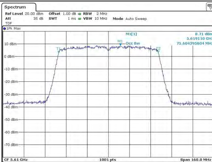
11AC80SISO_Ant2_5610
