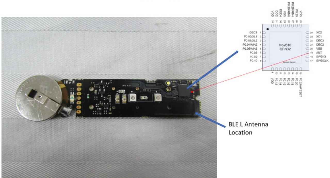
Antenna Location
