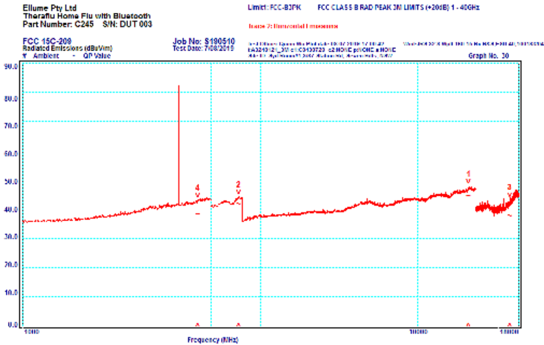
Graph 30 Horizontal Polarisation 1000 to 18000 MHz
