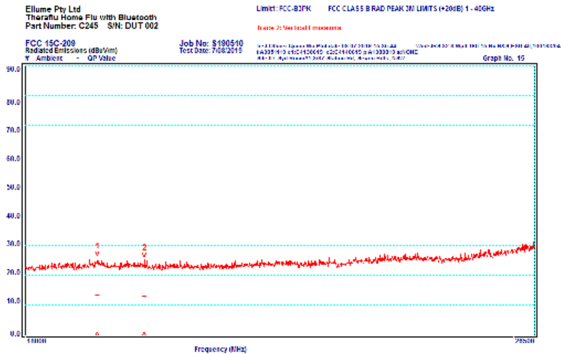
Graph 15 Vertical Polarisation 18000 to 26500 MHz
