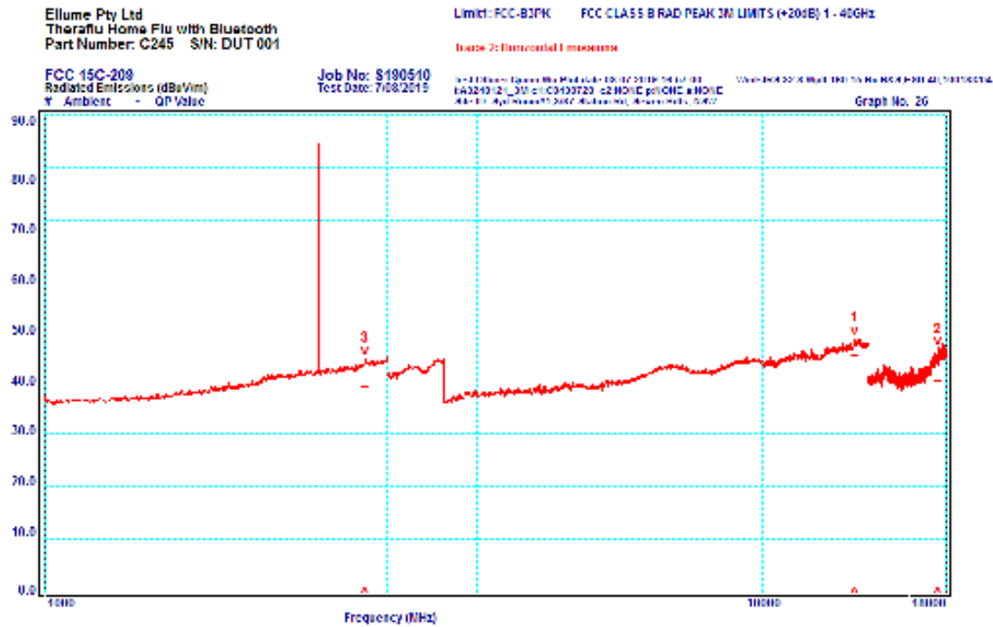
Graph 26 Horizontal Polarisation 1000 to 18000 MHz
