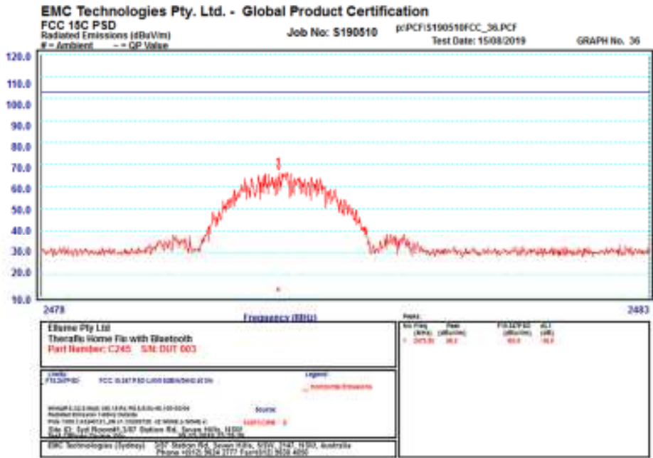
Graph 36 High Channel Horizontal Polarisation 2478 to 2483MHz
