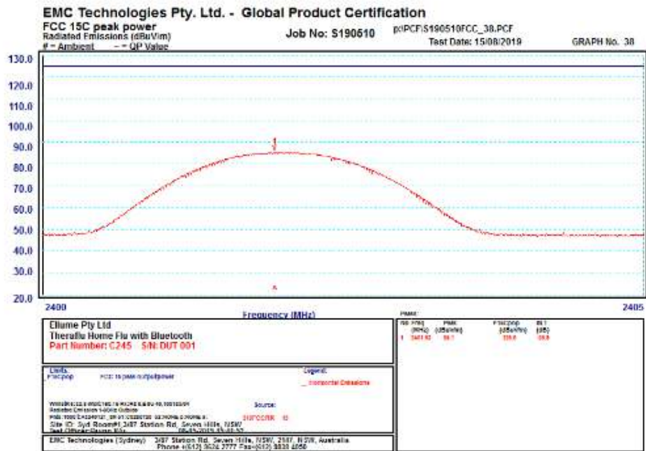
Graph 38 Low Channel Horizontal Polarisation 2400 to 2405MHz
