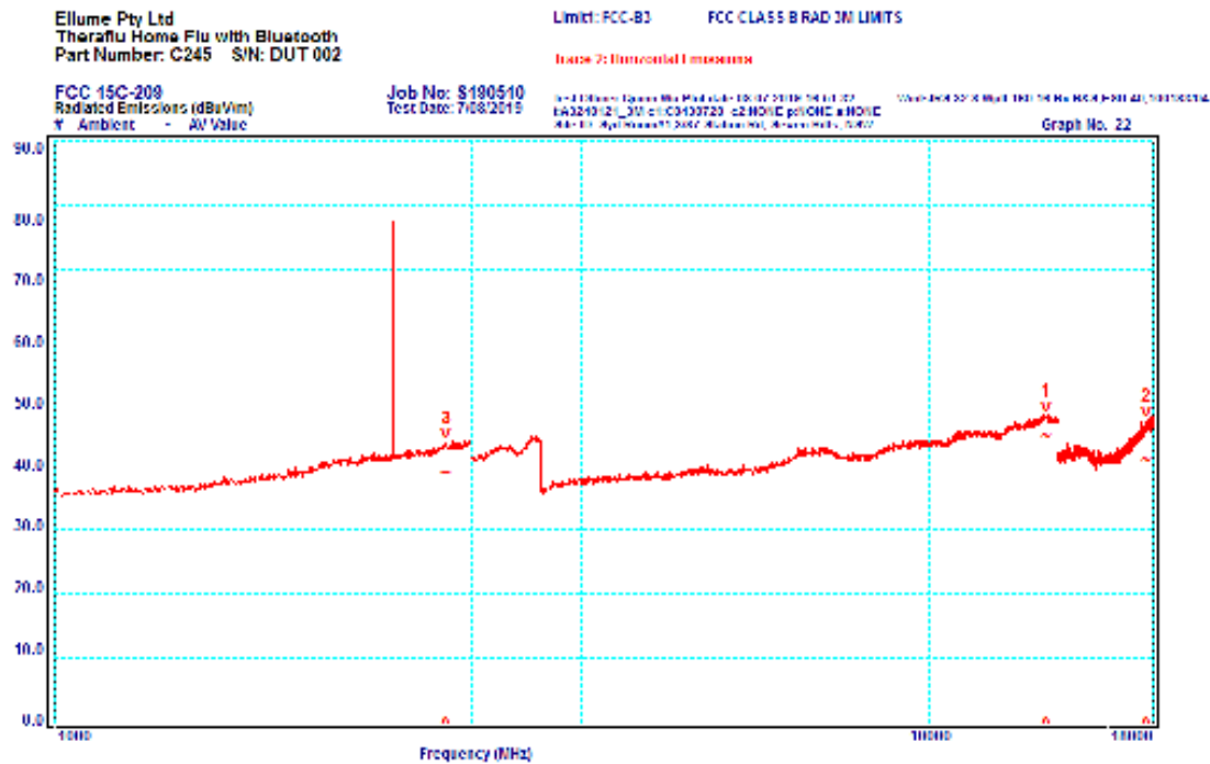
Graph 22 Horizontal Polarisation 1000 to 18000 MHz
