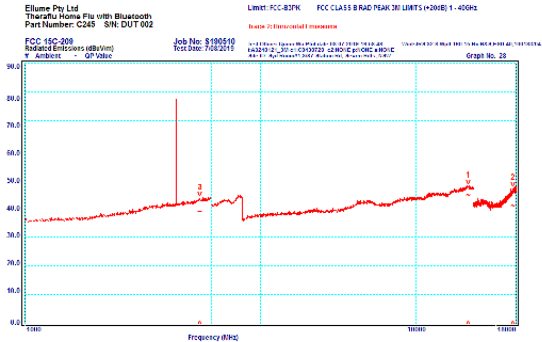
Graph 28 Horizontal Polarisation 1000 to 18000 MHz
