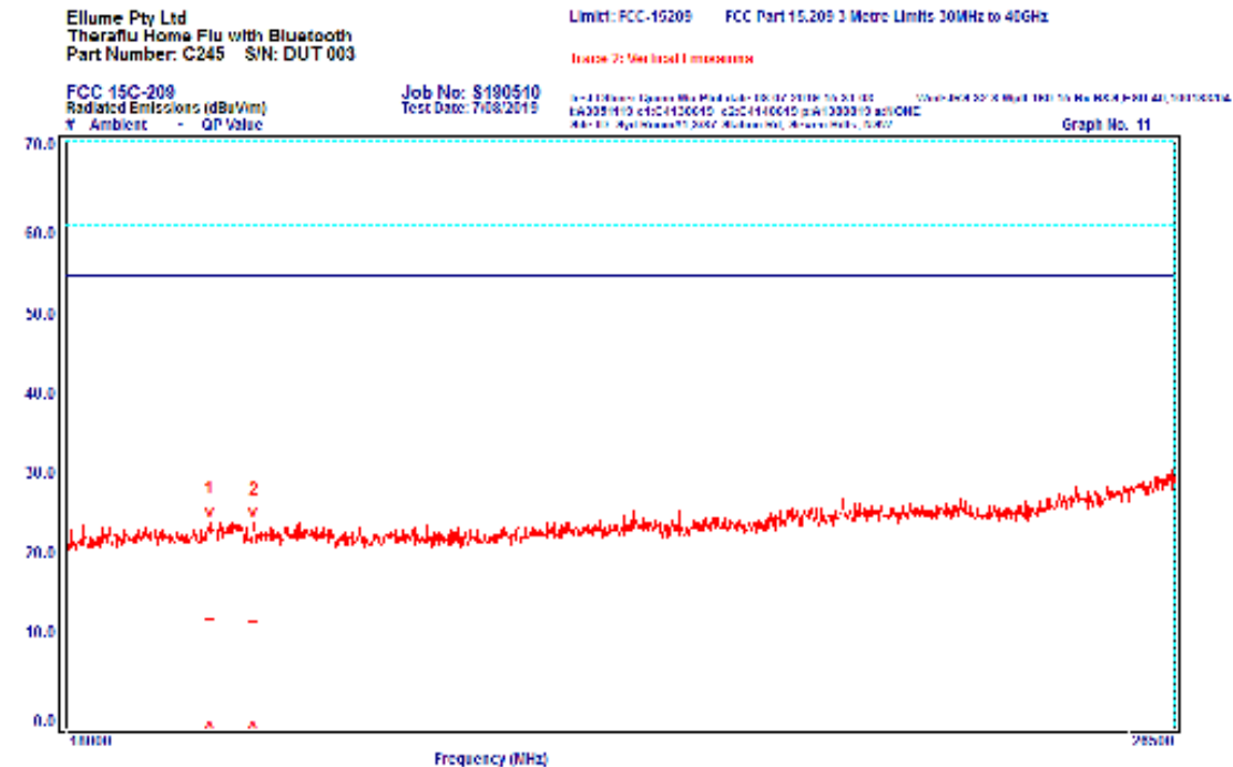
Graph 11 Vertical Polarisation 18000 to 26500 MHz
