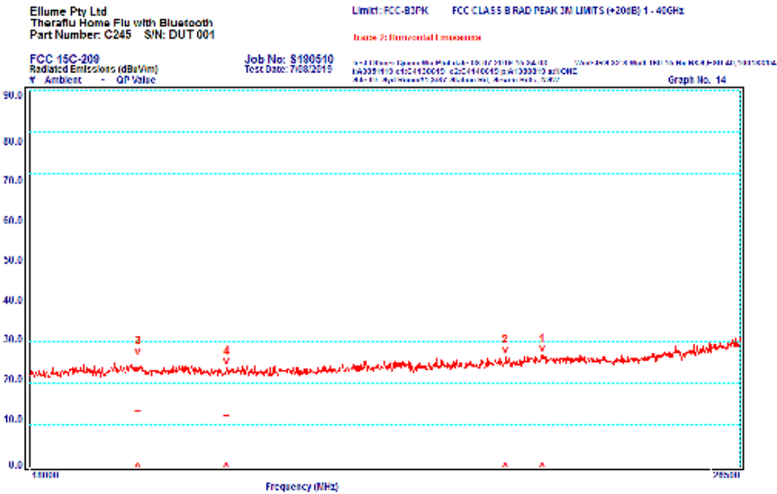
Graph 14 Horizontal Polarisation 18000 to 26500 MHz
