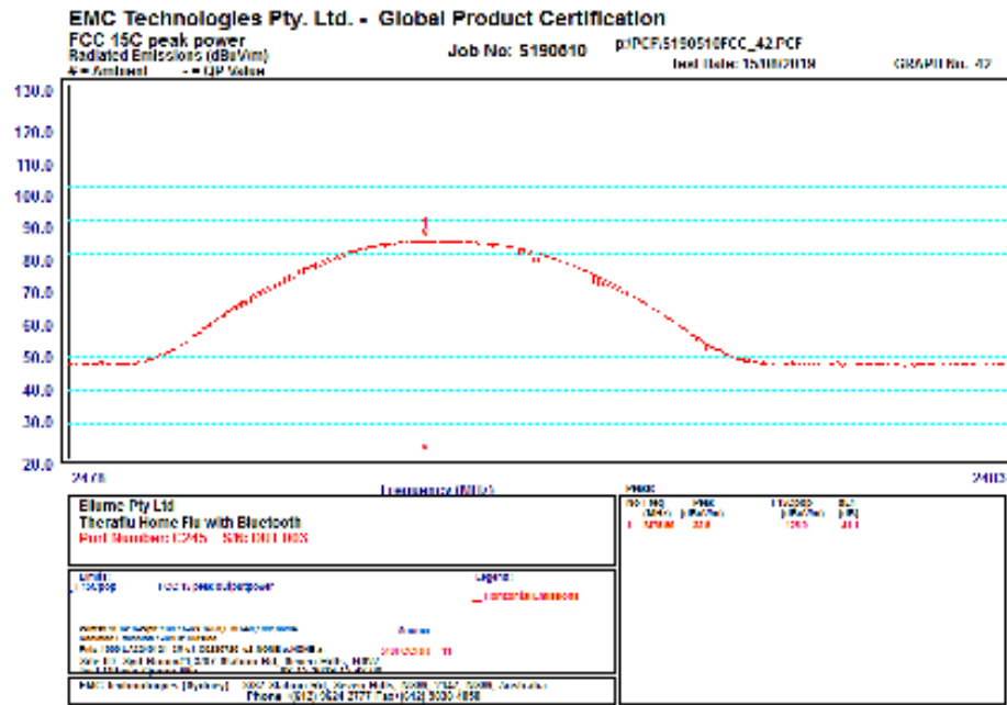
Graph 42 High Channel Horizontal Polarisation 2478 to 2483MHz
