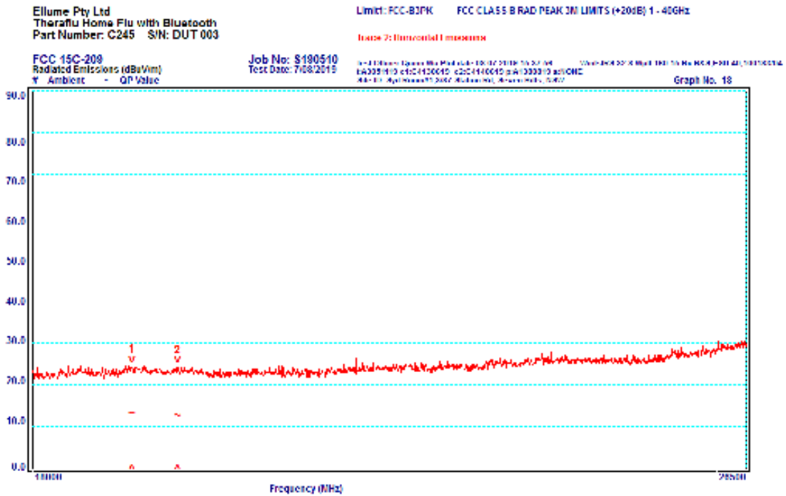
Graph 18 Horizontal Polarisation 18000 to 26500 MHz
