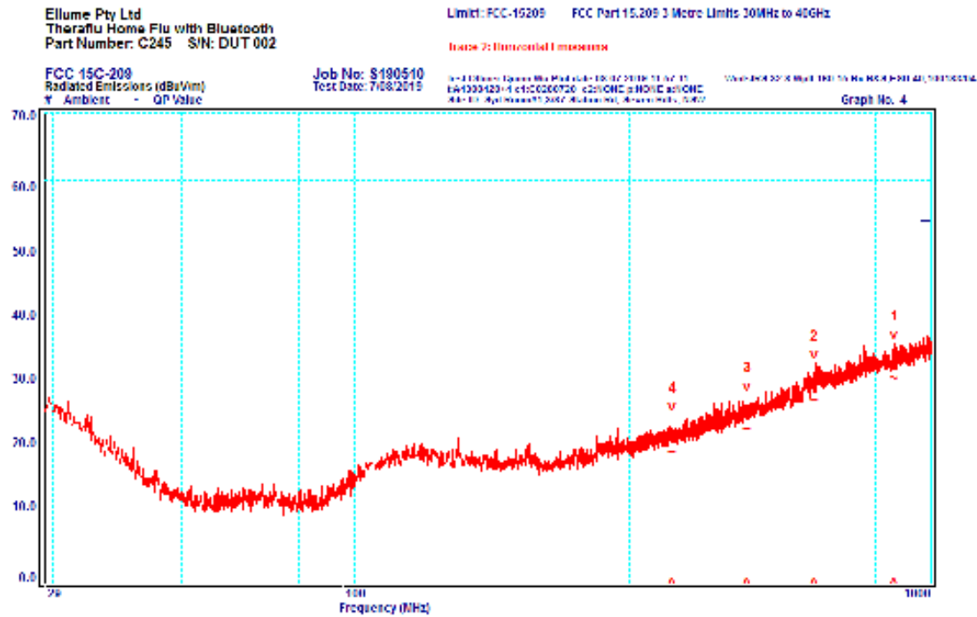
Graph 4 Horizontal Polarisation 29 to 1000MHz
