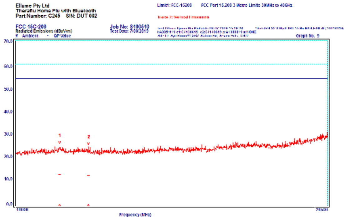
Graph 9 Vertical Polarisation 18000 to 26500 MHz
