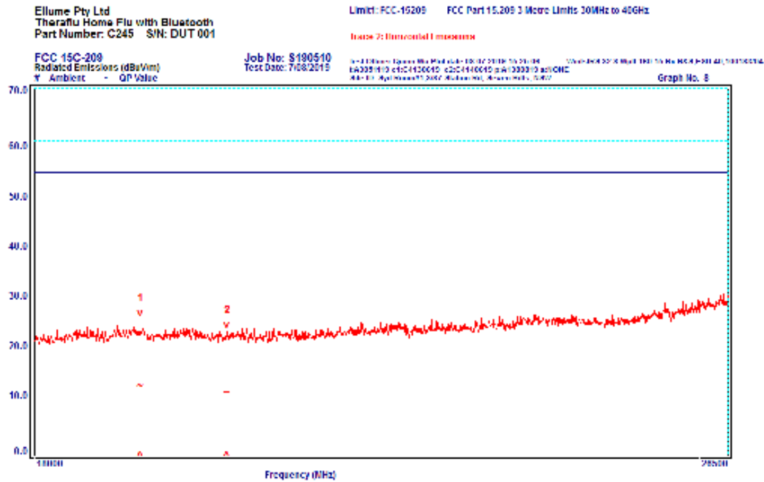
Graph 8 Horizontal Polarisation 18000 to 26500 MHz
