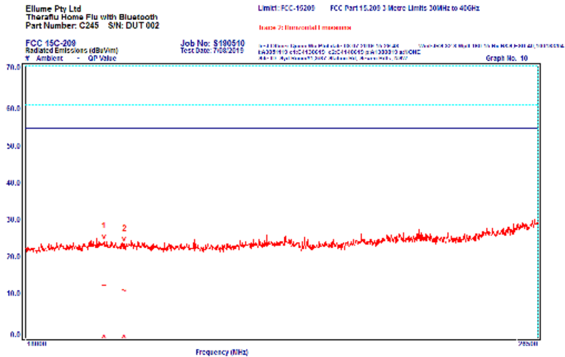
Graph 10 Horizontal Polarisation 18000 to 26500 MHz
