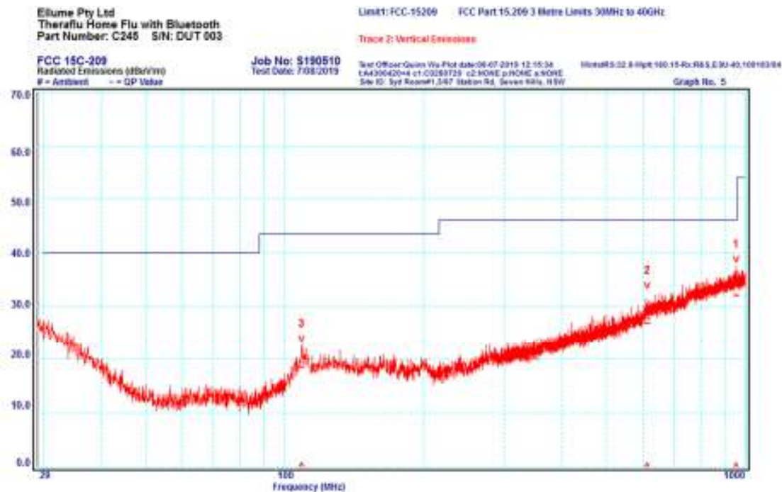
Graph 5 Vertical Polarisation 29 to 1000MHz
