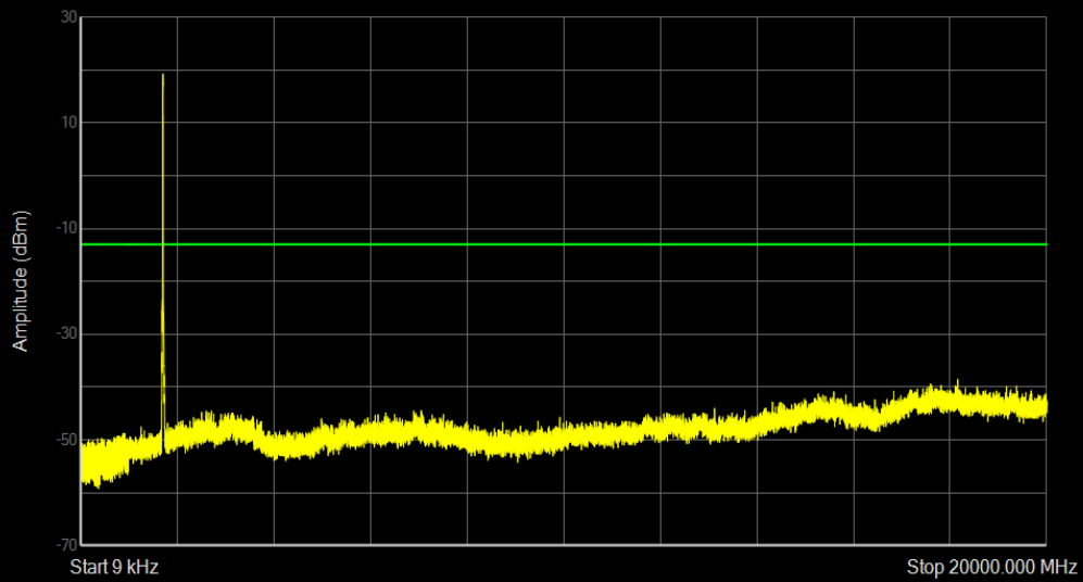
Band66 16QAM BW=10MHz Channel=132022 RB Size=50 Position=#0
