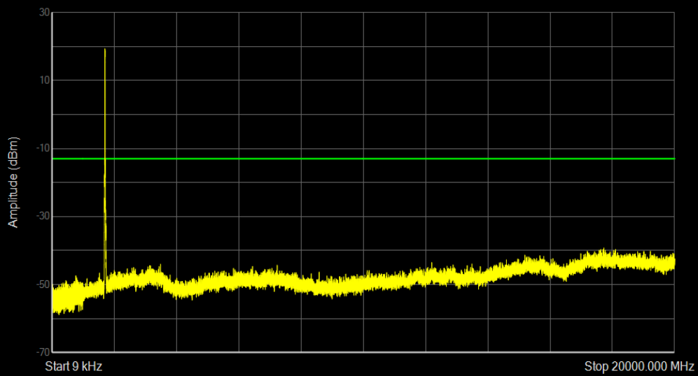
Band66 16QAM BW=10MHz Channel=132022 RB Size=50 Position=#0
