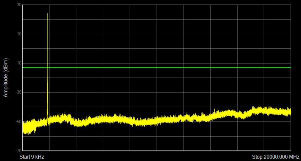
Band25 16QAM BW=15MHz Channel=26365 RB Size=1 Position=#0
