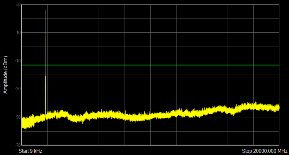
Band25 16QAM BW=15MHz Channel=26115 RB Size=1 Position=#0
