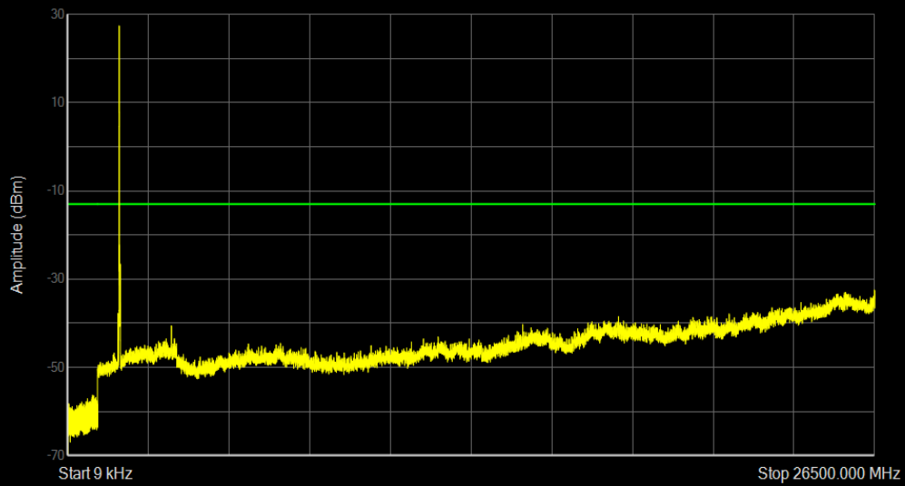
Band66 16QAM BW=20MHz Channel=132072 RB Size=1 Position=#0
