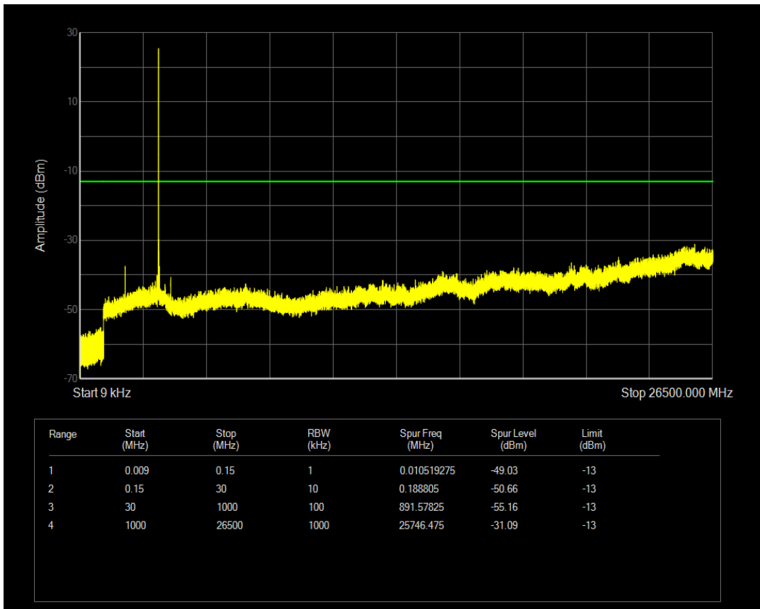
n78 SCS=30kHz CP_QPSK BW=20MHz Channel=620668 RB=1@50
