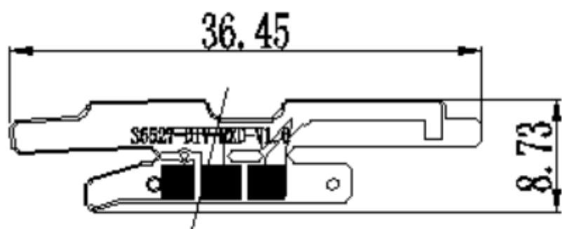
Diversity Antenna
