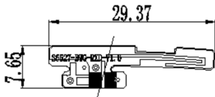
Diversity Antenna
