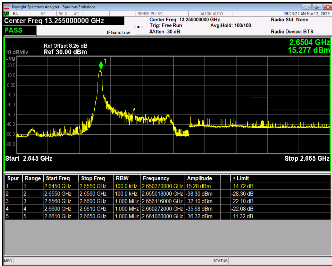
Band41(2545-2655) 16QAM BW=5MHz Channel=41215 RB Size=1 Position=#Max
