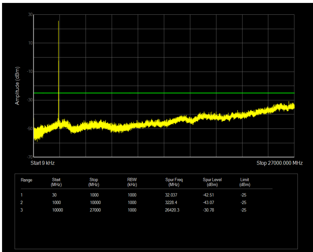
Band41(2545-2655) 16QAM BW=15MHz Channel=40690 RB Size=75 Position=#0
