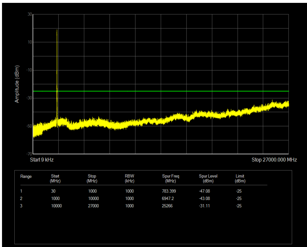
Band41(2545-2655) QPSK BW=15MHz Channel=40690 RB Size=1 Position=#0
