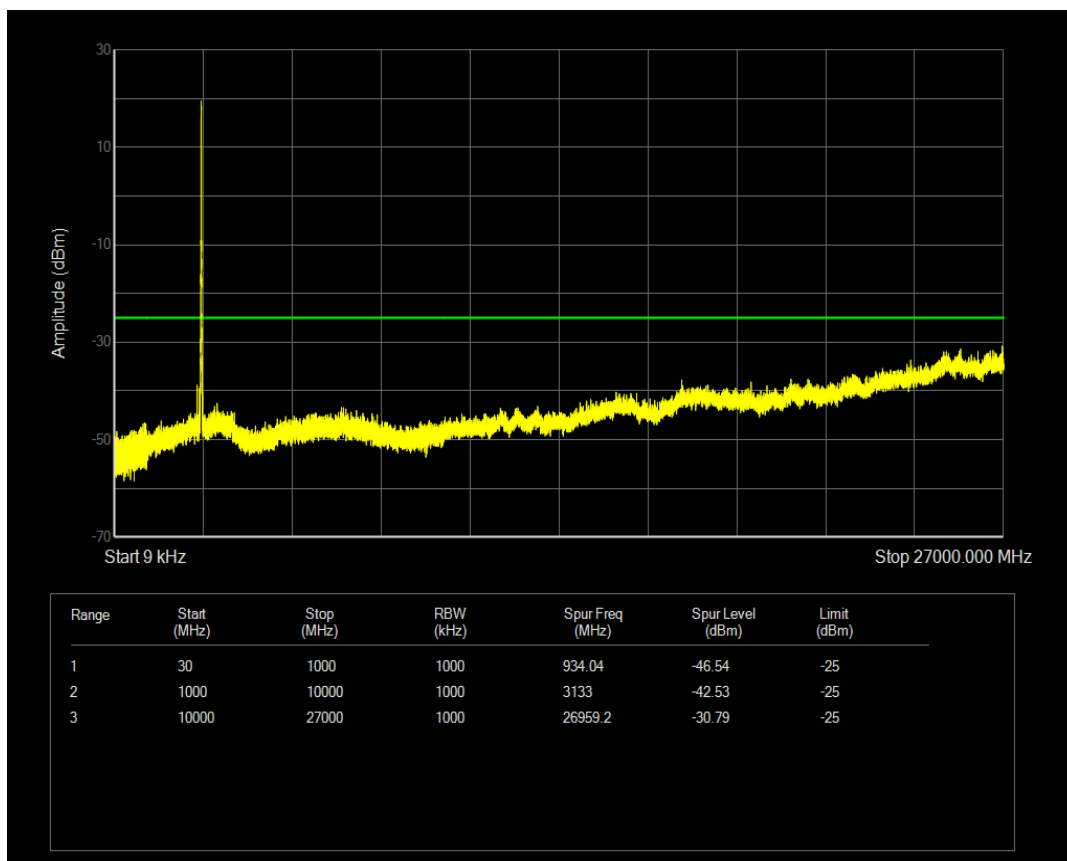
Band41(2545-2655) 16QAM BW=10MHz Channel=41190 RB Size=1 Position=#0
