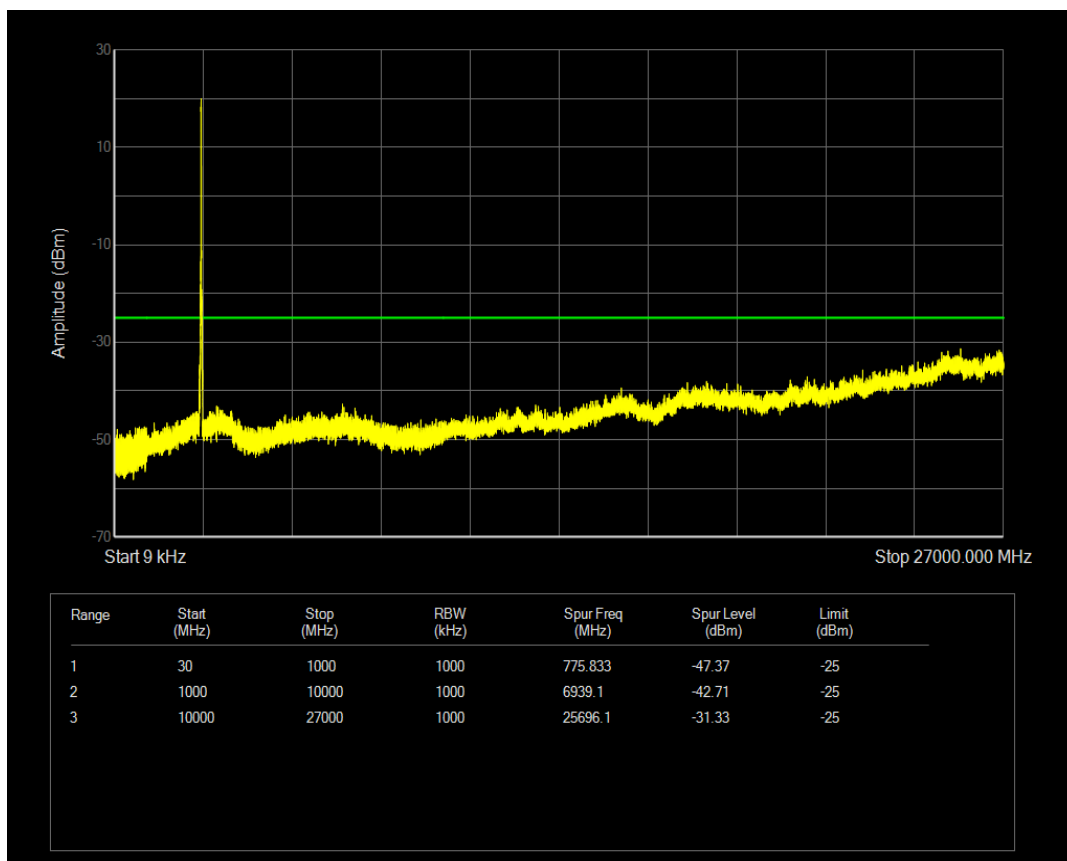
Band41(2545-2655) 16QAM BW=15MHz Channel=41165 RB Size=1 Position=#0
