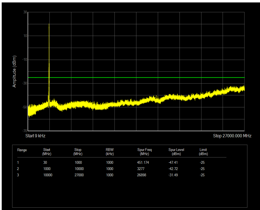
Band41(2545-2655) QPSK BW=20MHz Channel=40240 RB Size=1 Position=#0
