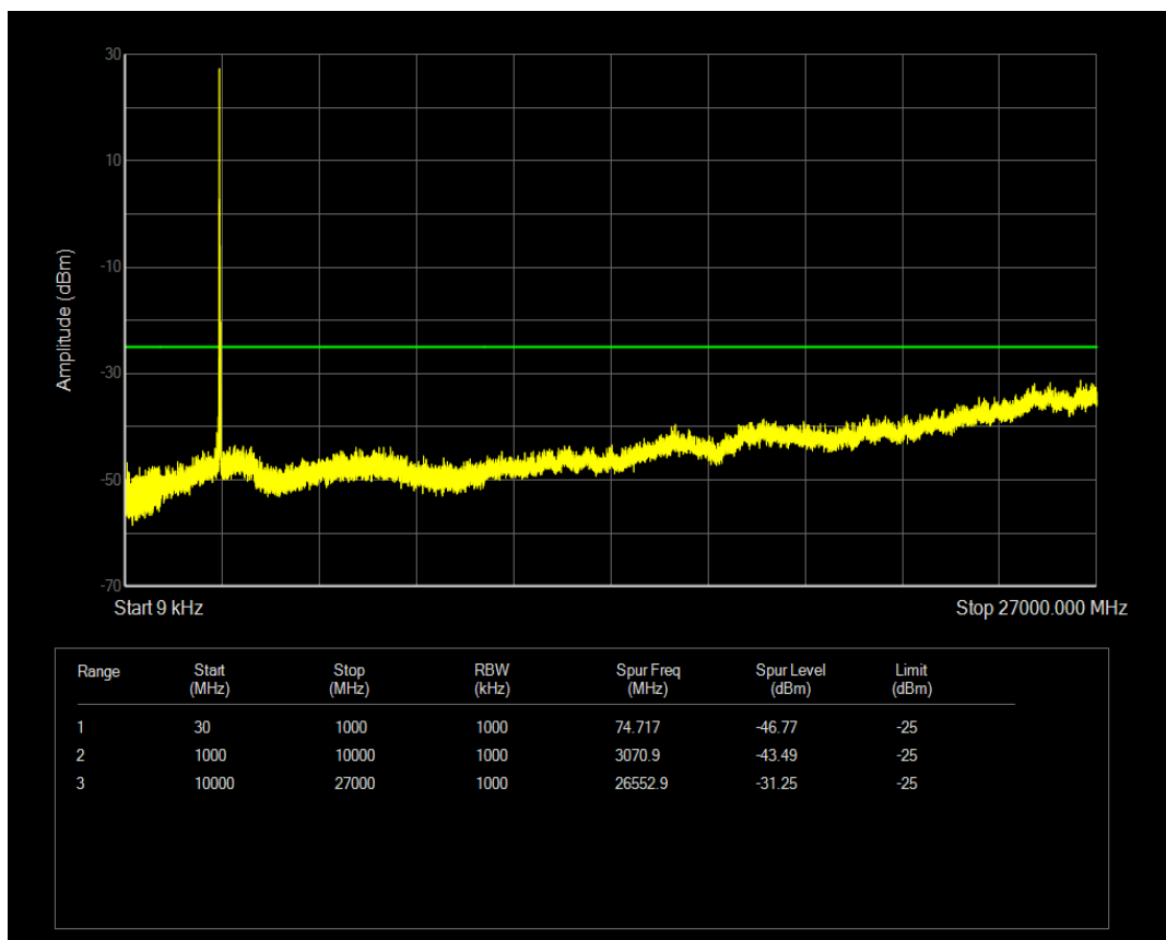
Band41(2545-2655) 16QAM BW=20MHz Channel=41140 RB Size=1 Position=#0
