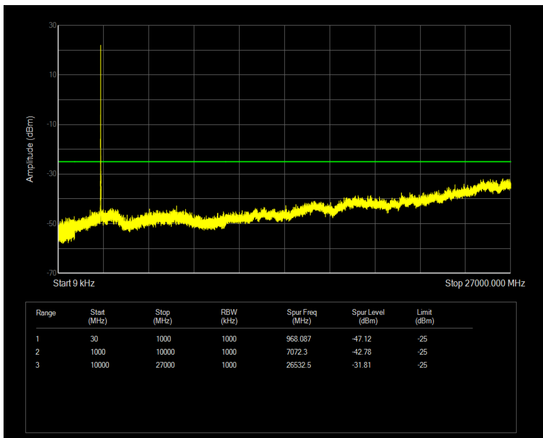
Band41(2545-2655) 16QAM BW=5MHz Channel=40165 RB Size=1 Position=#0
