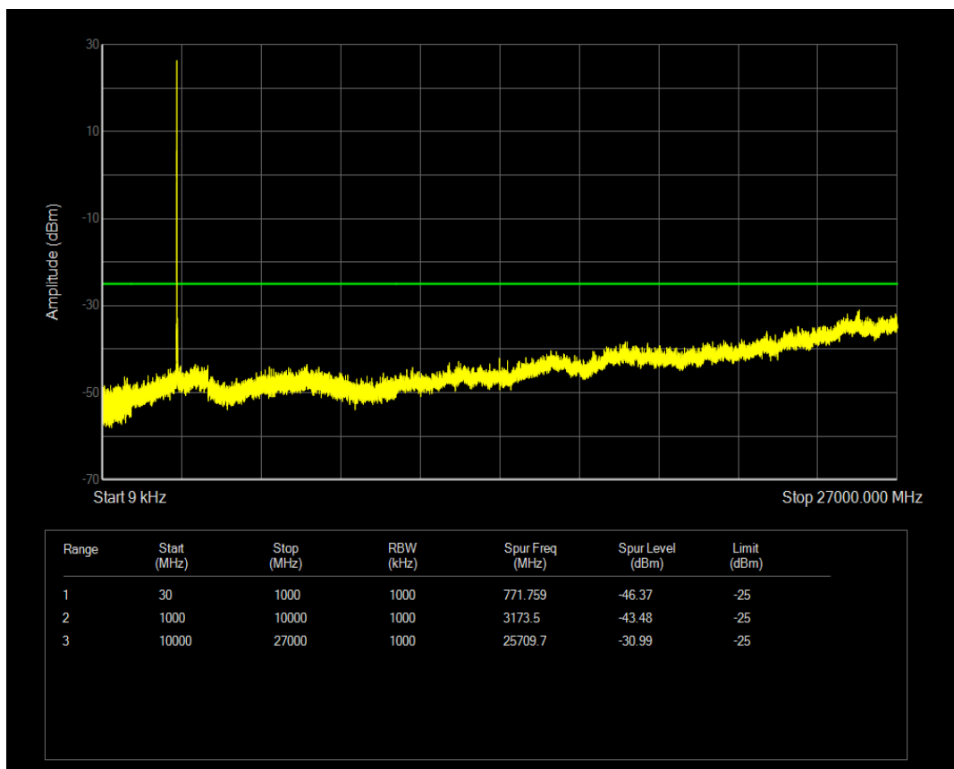
Band41(2545-2655) 16QAM BW=10MHz Channel=40190 RB Size=50 Position=#0
