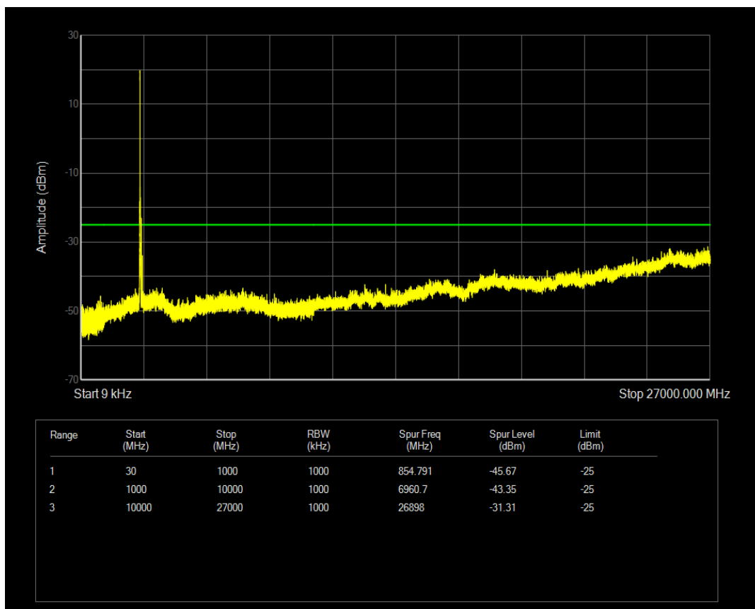
Band41(2545-2655) 16QAM BW=10MHz Channel=40190 RB Size=1 Position=#0
