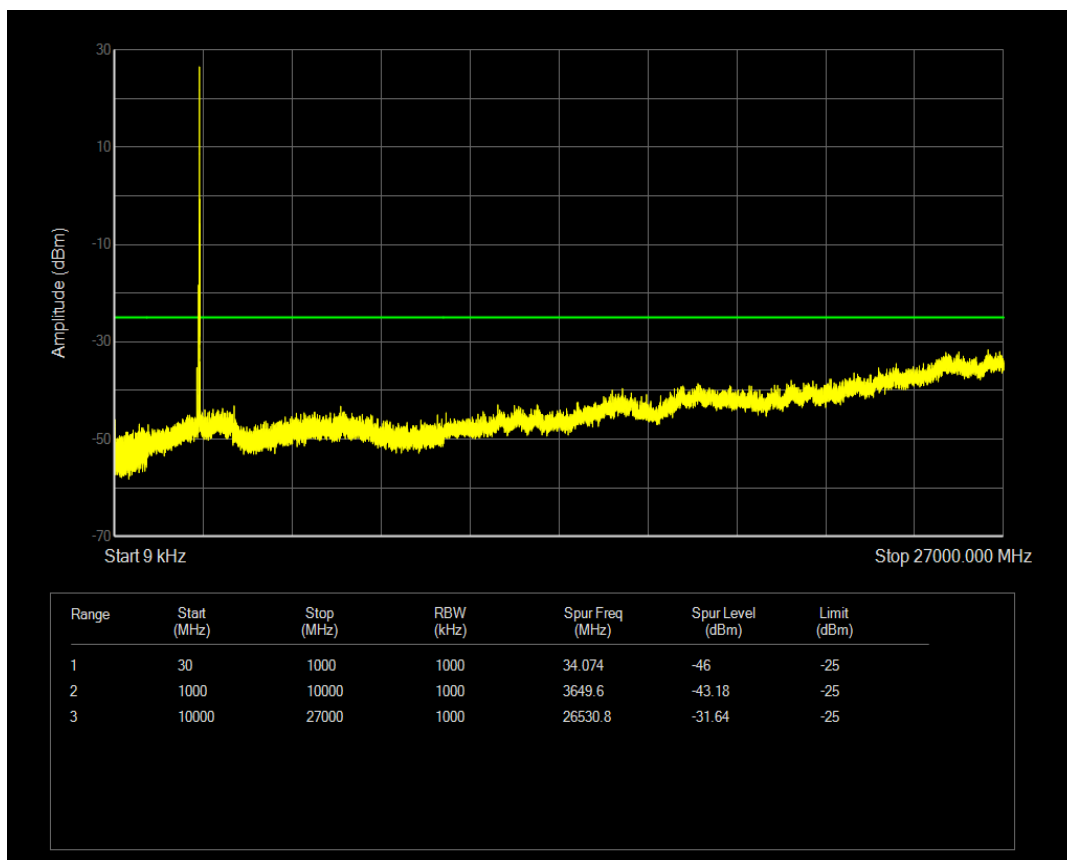
Band41(2545-2655) QPSK BW=10MHz Channel=40690 RB Size=50 Position=#0
