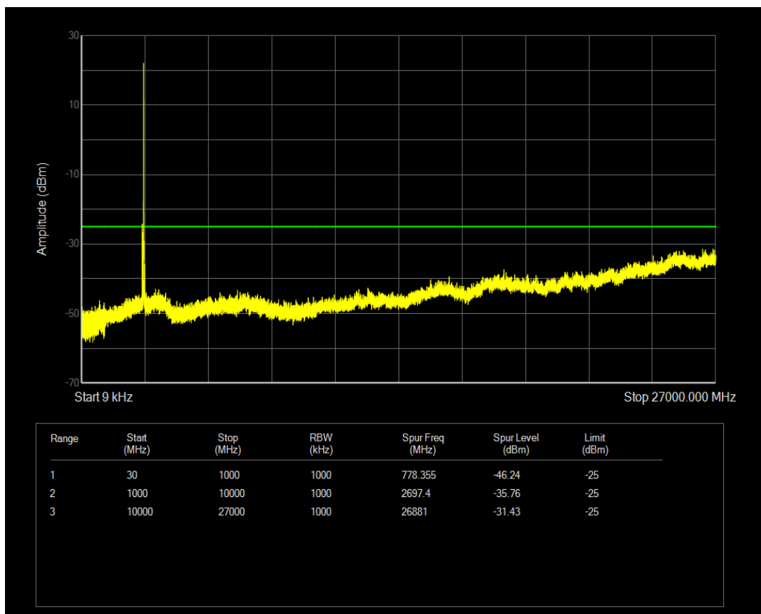
Band41(2545-2655) QPSK BW=10MHz Channel=40190 RB Size=1 Position=#0
