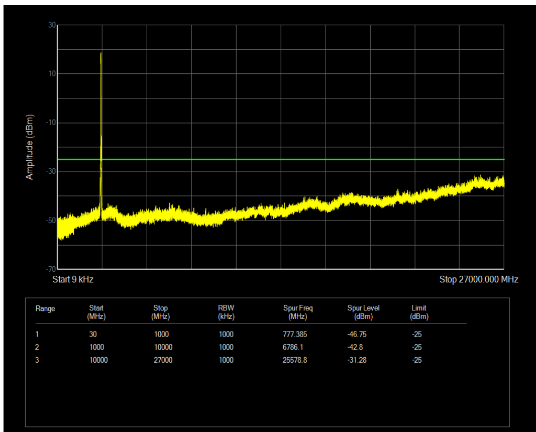
Band41(2545-2655) 16QAM BW=20MHz Channel=41140 RB Size=100 Position=#0
