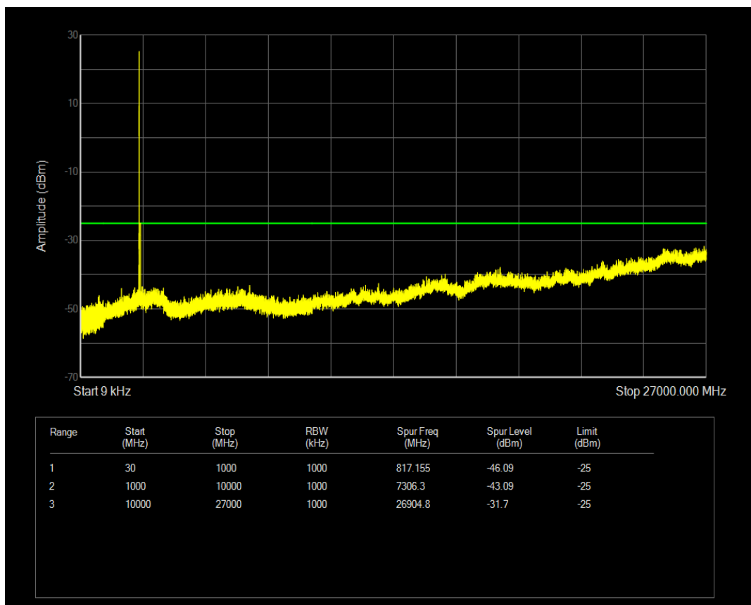
Band41(2545-2655) 16QAM BW=5MHz Channel=40165 RB Size=25 Position=#0
