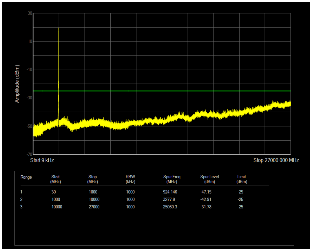
Band41(2545-2655) QPSK BW=15MHz Channel=40215 RB Size=1 Position=#0
