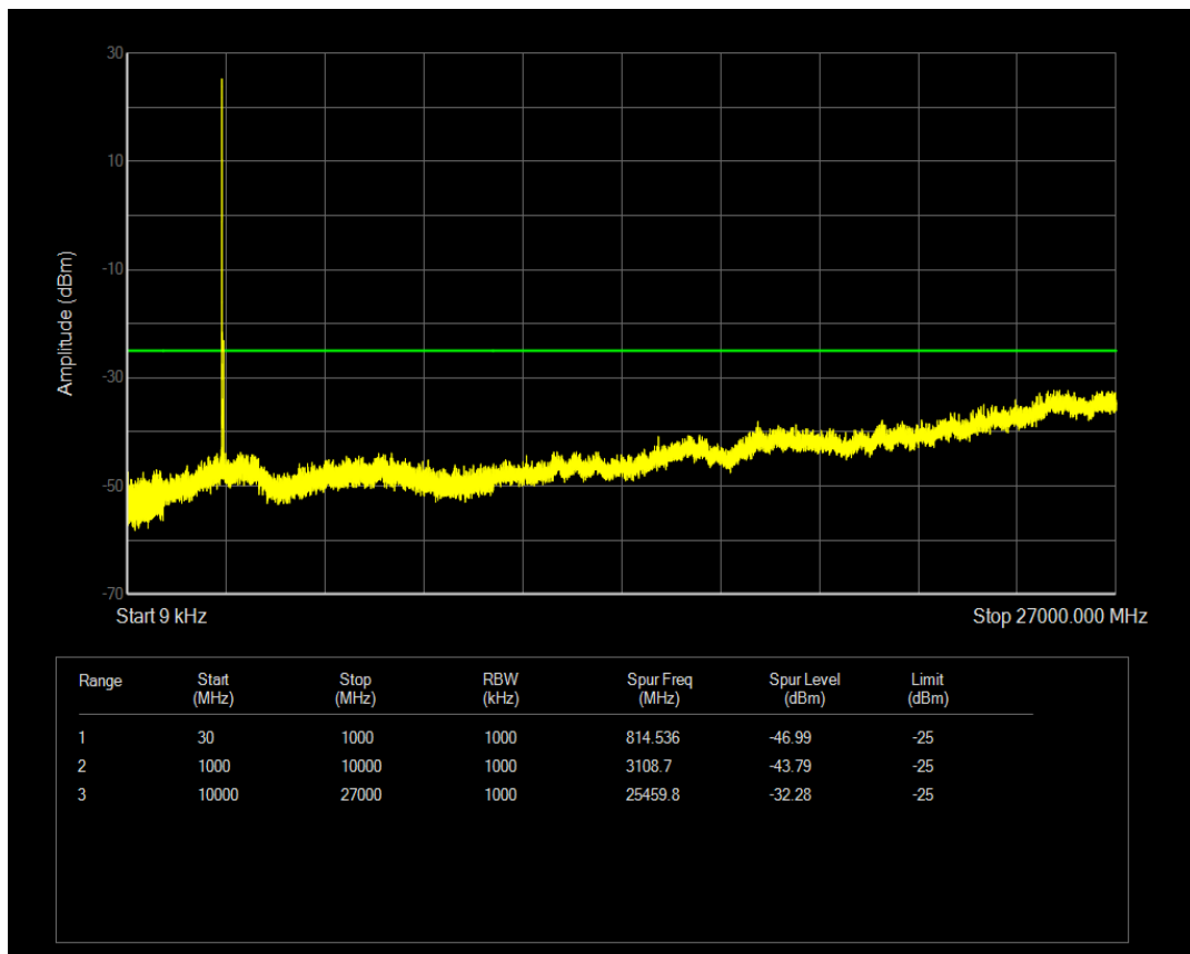
Band41(2545-2655) 16QAM BW=5MHz Channel=40690 RB Size=25 Position=#0
