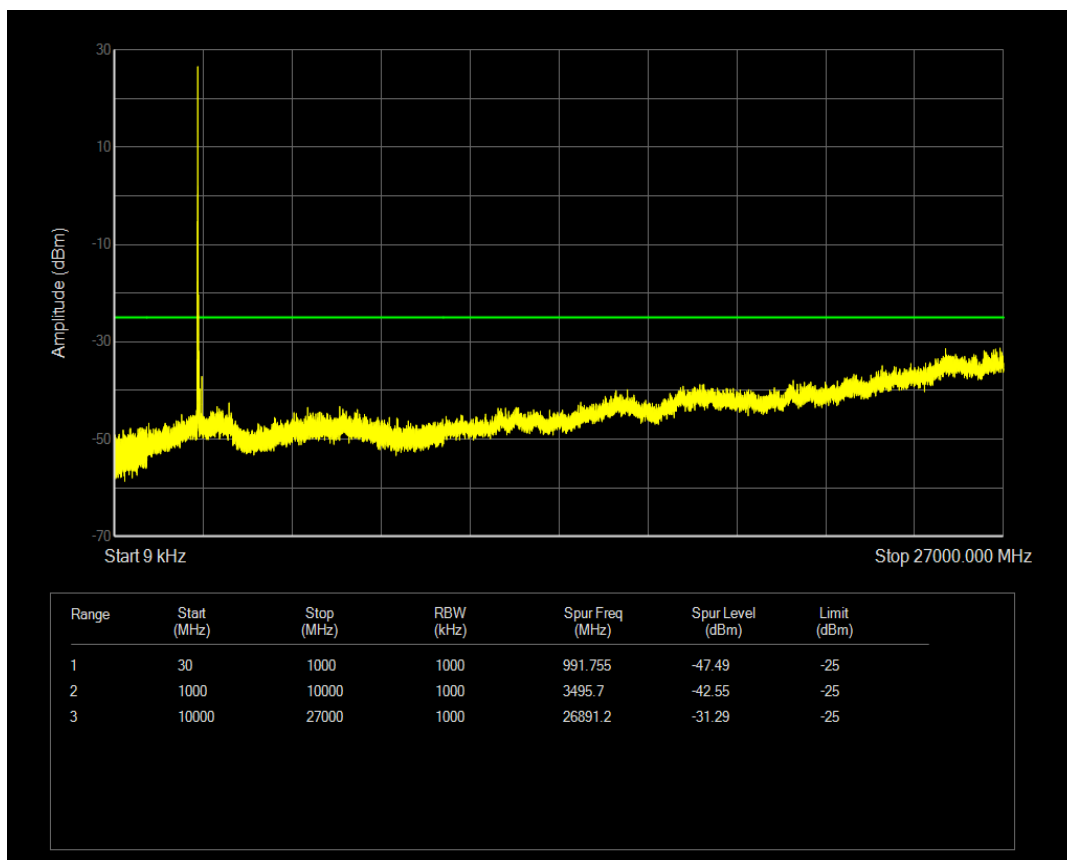
Band41(2545-2655) 16QAM BW=20MHz Channel=40240 RB Size=100 Position=#0
