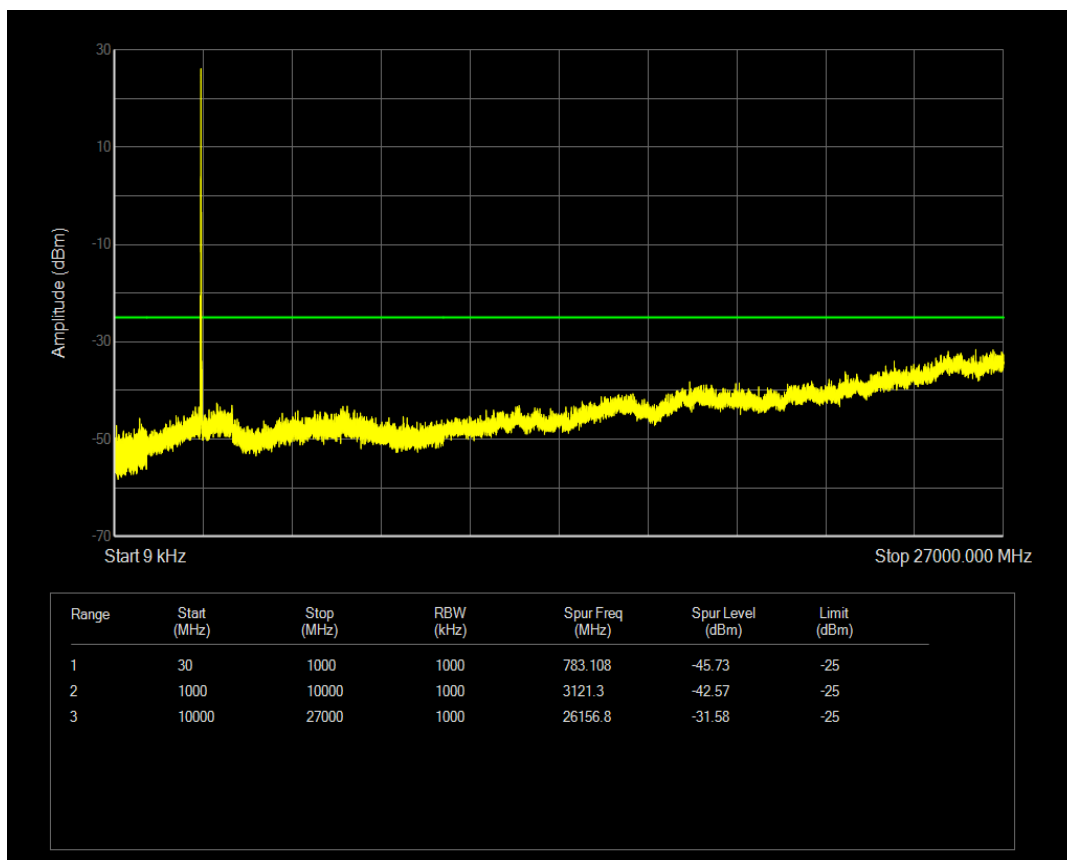
Band41(2545-2655) 16QAM BW=15MHz Channel=41165 RB Size=75 Position=#0
