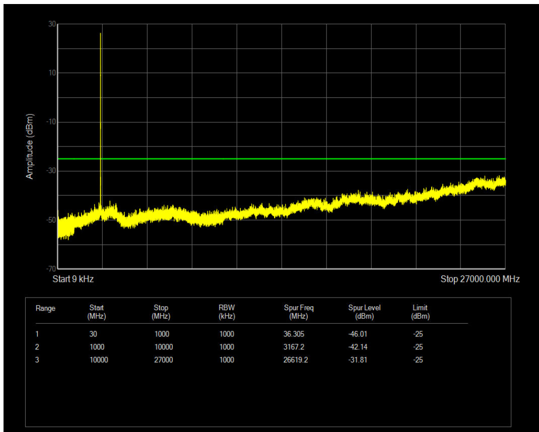
Band41(2545-2655) QPSK BW=5MHz Channel=40690 RB Size=25 Position=#0
