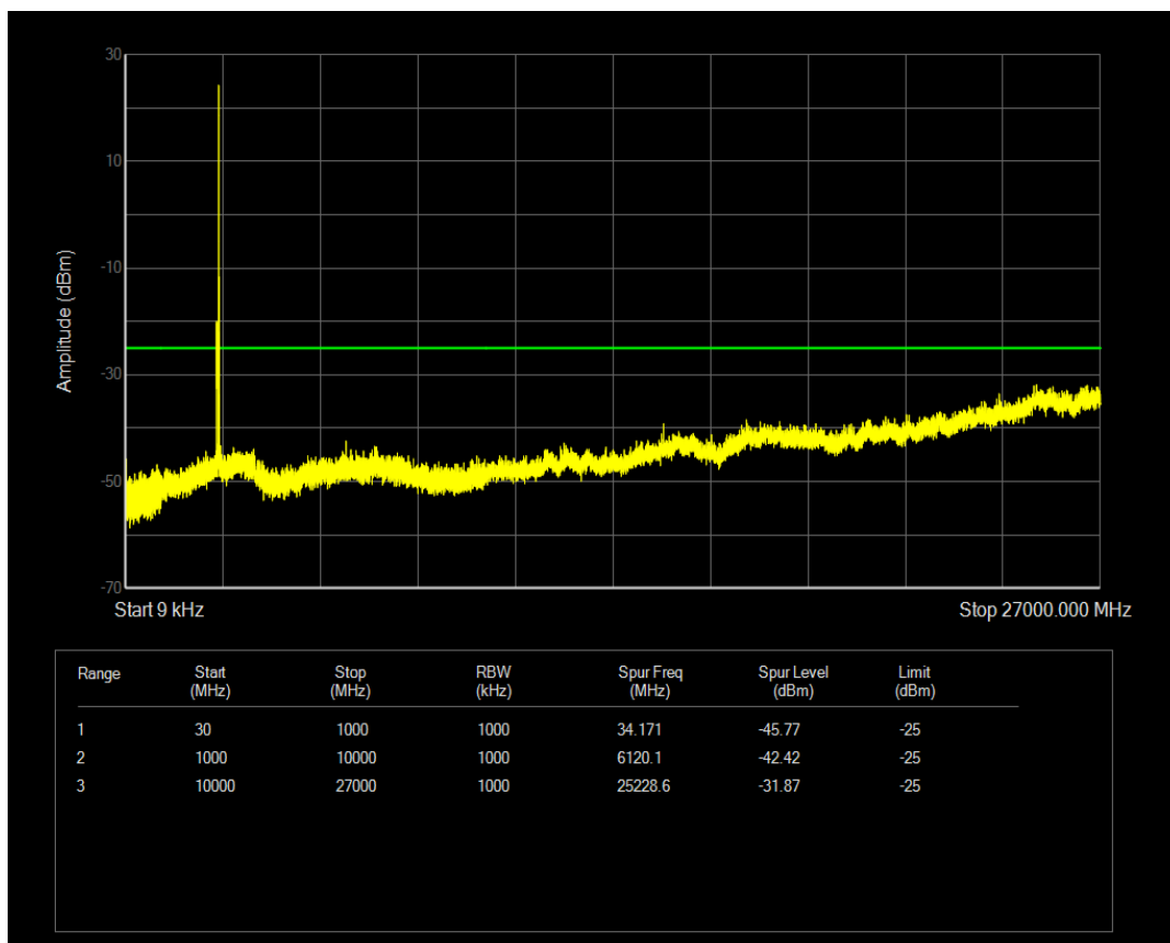
Band41(2545-2655) 16QAM BW=10MHz Channel=40690 RB Size=50 Position=#0
