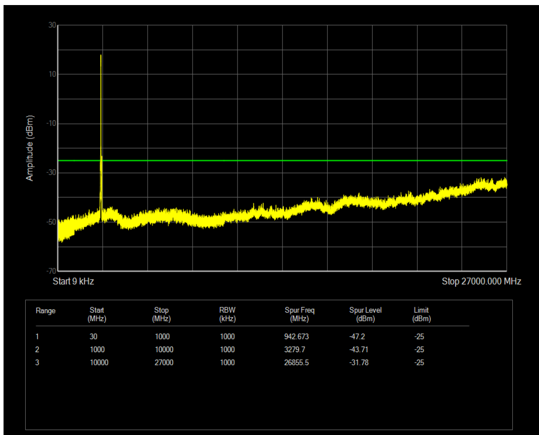
Band41(2545-2655) QPSK BW=15MHz Channel=41165 RB Size=1 Position=#0
