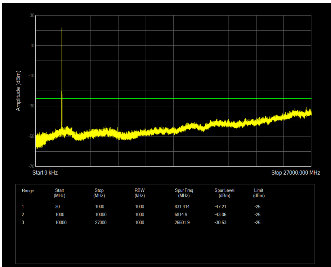
Band41(2545-2655) QPSK BW=5MHz Channel=41215 RB Size=1 Position=#0
