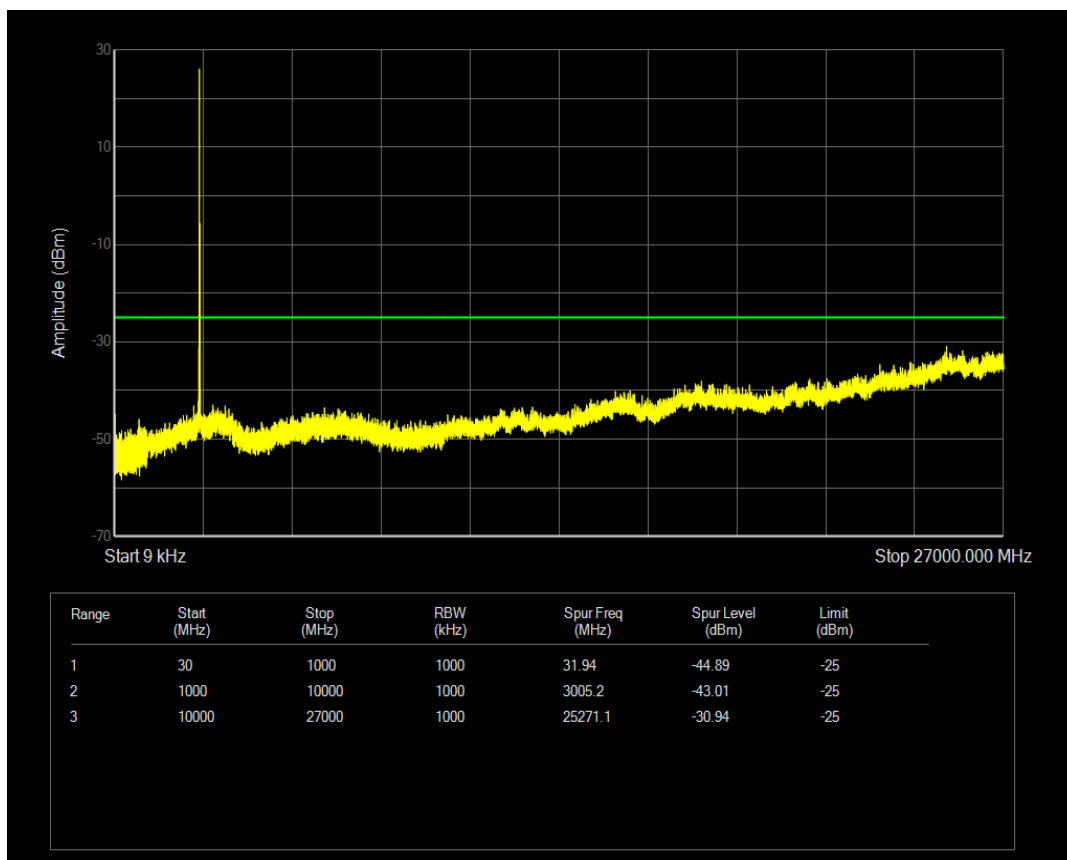
Band41(2545-2655) QPSK BW=15MHz Channel=40690 RB Size=75 Position=#0
