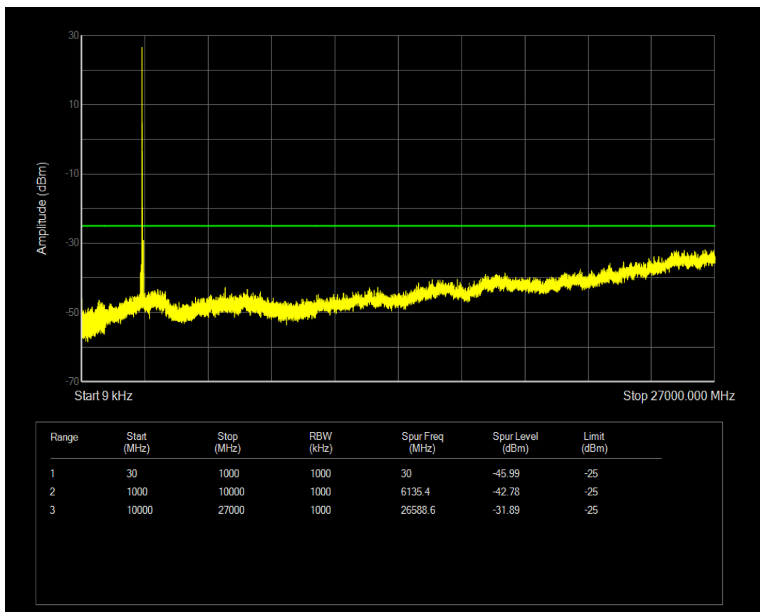
Band41(2545-2655) QPSK BW=20MHz Channel=40690 RB Size=100 Position=#0
