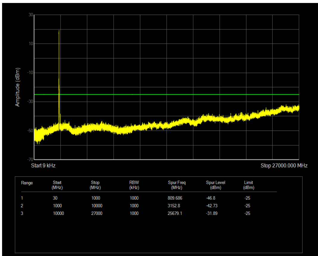
Band41(2545-2655) QPSK BW=10MHz Channel=40690 RB Size=1 Position=#0
