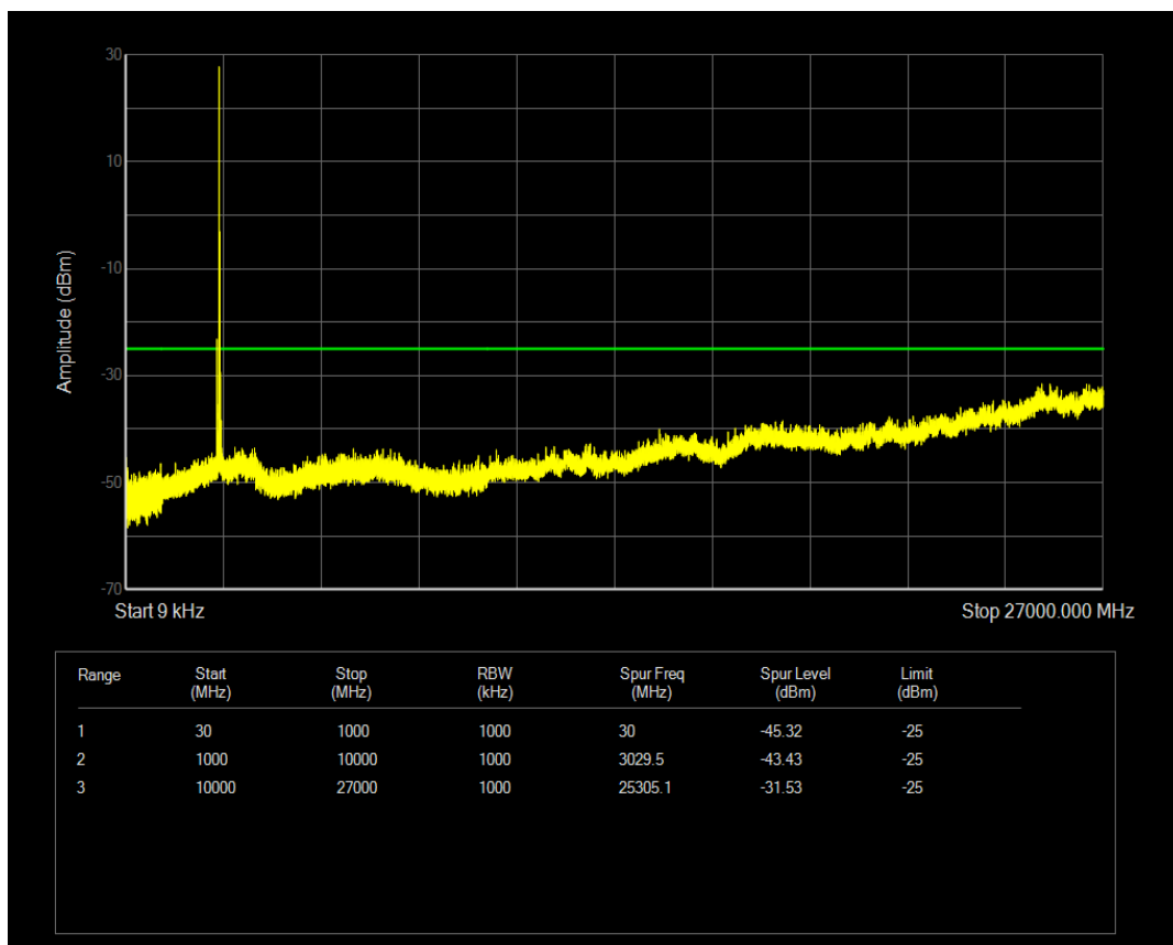
Band41(2545-2655) 16QAM BW=20MHz Channel=40690 RB Size=100 Position=#0
