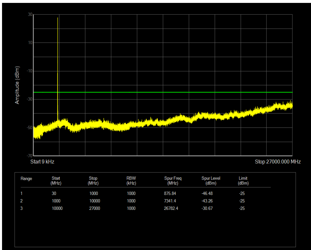
Band41(2545-2655) QPSK BW=10MHz Channel=40190 RB Size=50 Position=#0
