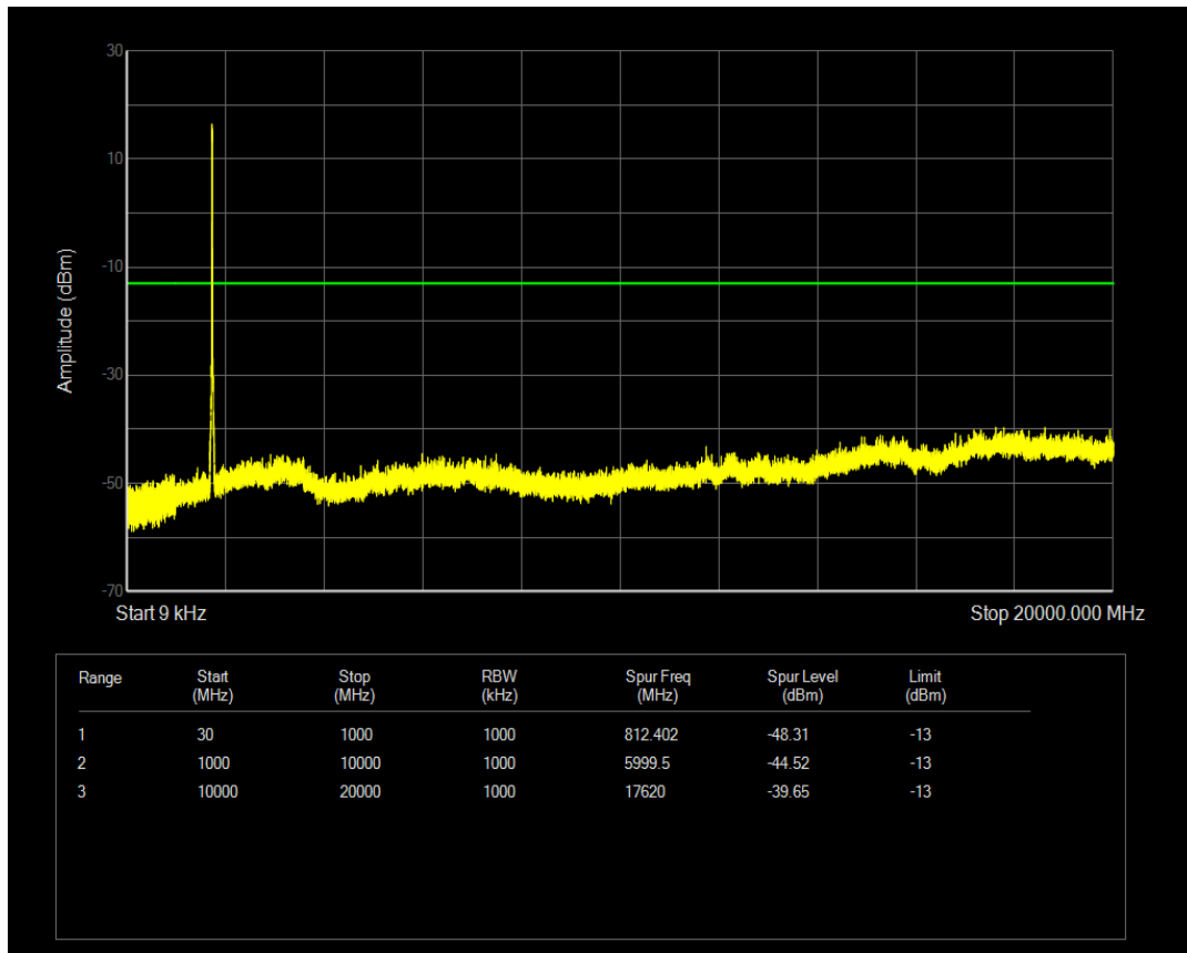
Band41(2545-2655) QPSK BW=5MHz Channel=40165 RB Size=1 Position=#0
