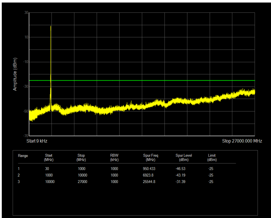
Band41(2545-2655) 16QAM BW=15MHz Channel=40690 RB Size=1 Position=#0
