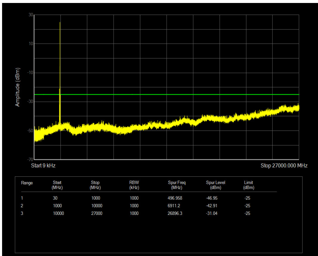
Band41(2545-2655) 16QAM BW=10MHz Channel=41190 RB Size=50 Position=#0
