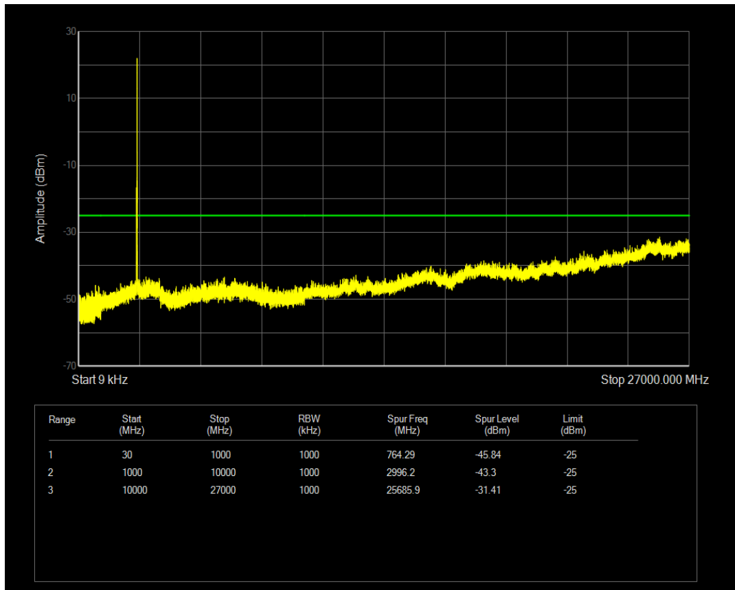
Band41(2545-2655) 16QAM BW=5MHz Channel=40690 RB Size=1 Position=#0
