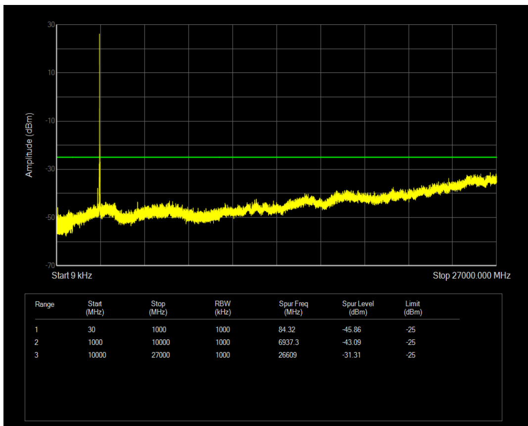
Band41(2545-2655) QPSK BW=10MHz Channel=41190 RB Size=50 Position=#0
