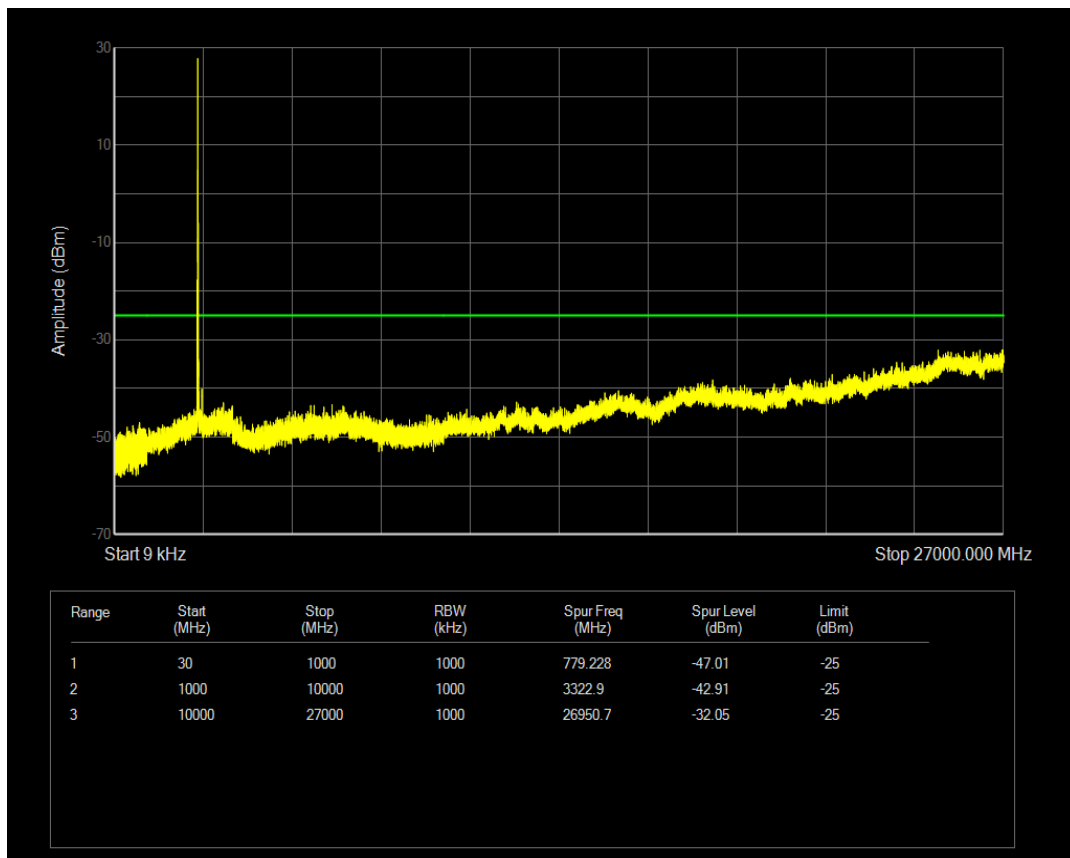
Band41(2545-2655) QPSK BW=15MHz Channel=40215 RB Size=75 Position=#0
