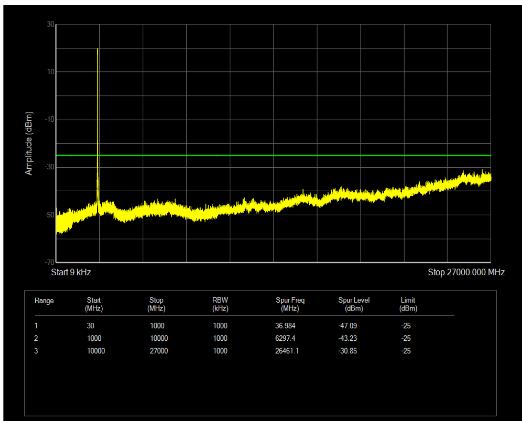
Band41(2545-2655) QPSK BW=10MHz Channel=41190 RB Size=1 Position=#0
