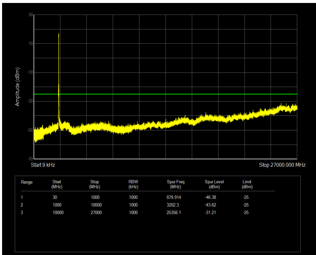
Band41(2545-2655) 16QAM BW=20MHz Channel=40240 RB Size=1 Position=#0
