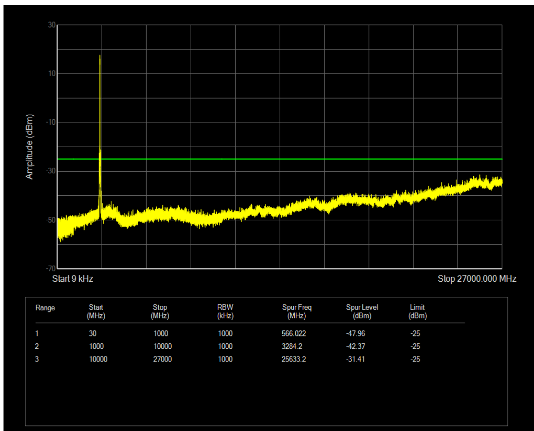
Band41(2545-2655) QPSK BW=20MHz Channel=41140 RB Size=1 Position=#0
