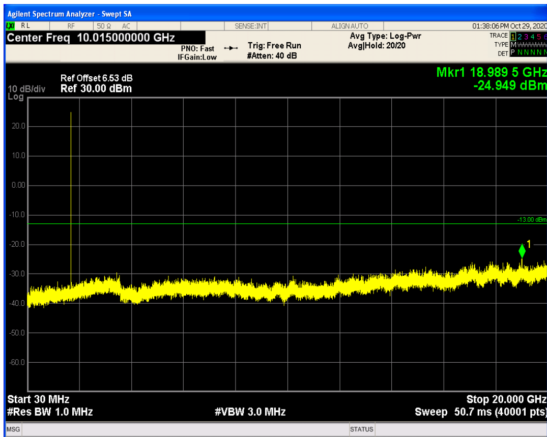
LTE Band4 QPSK BW=1.4MHz Channel=19957 RB Size=6 Position=#0
