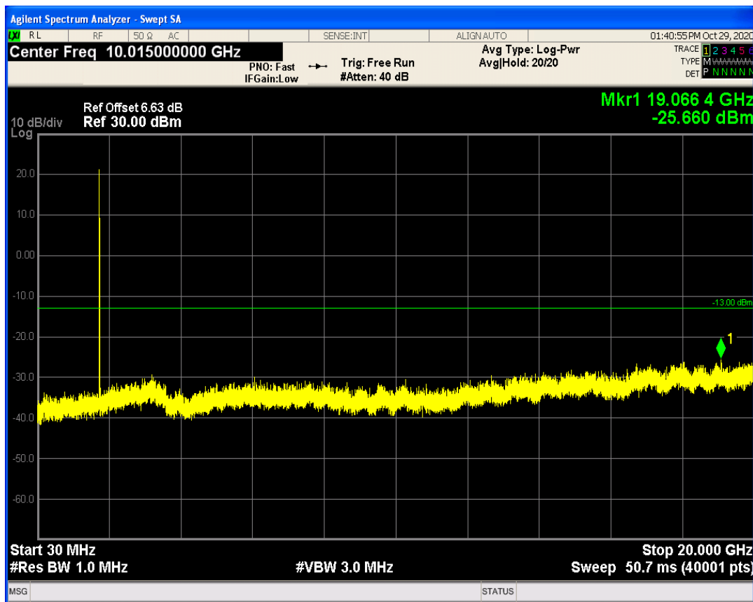
LTE Band4 QPSK BW=3MHz Channel=19965 RB Size=1 Position=#0
