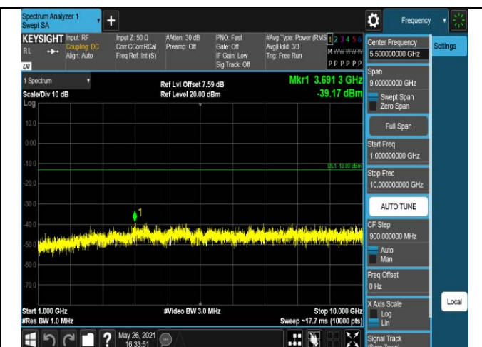
Band17-10MHz-QPSK-23780-1RB#0-Range2:1000~10
