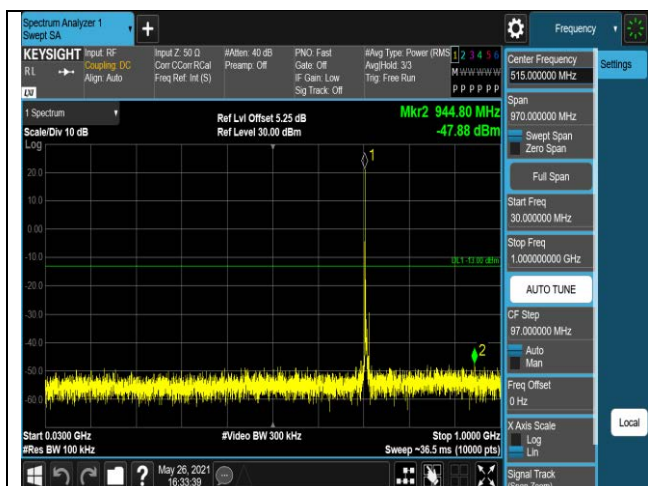
Band17-10MHz-QPSK-23780-1RB#0-Range1:30~1
