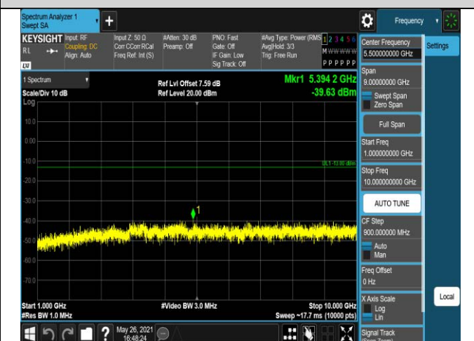
Band17-10MHz-QPSK-23790-1RB#0-Range2:1000~10
