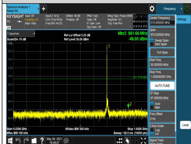
Band17-10MHz-QPSK-23800-1RB#0-Range1:30~1
