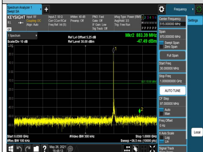
Band17-10MHz-QPSK-23790-1RB#0-Range1:30~1
