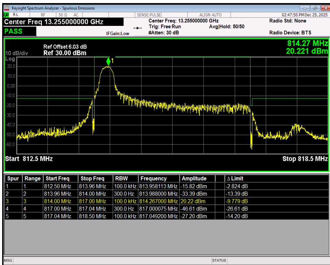
Band26(814-824) QPSK BW=3MHz Channel=26705 RB Size=1 Position=#Max
