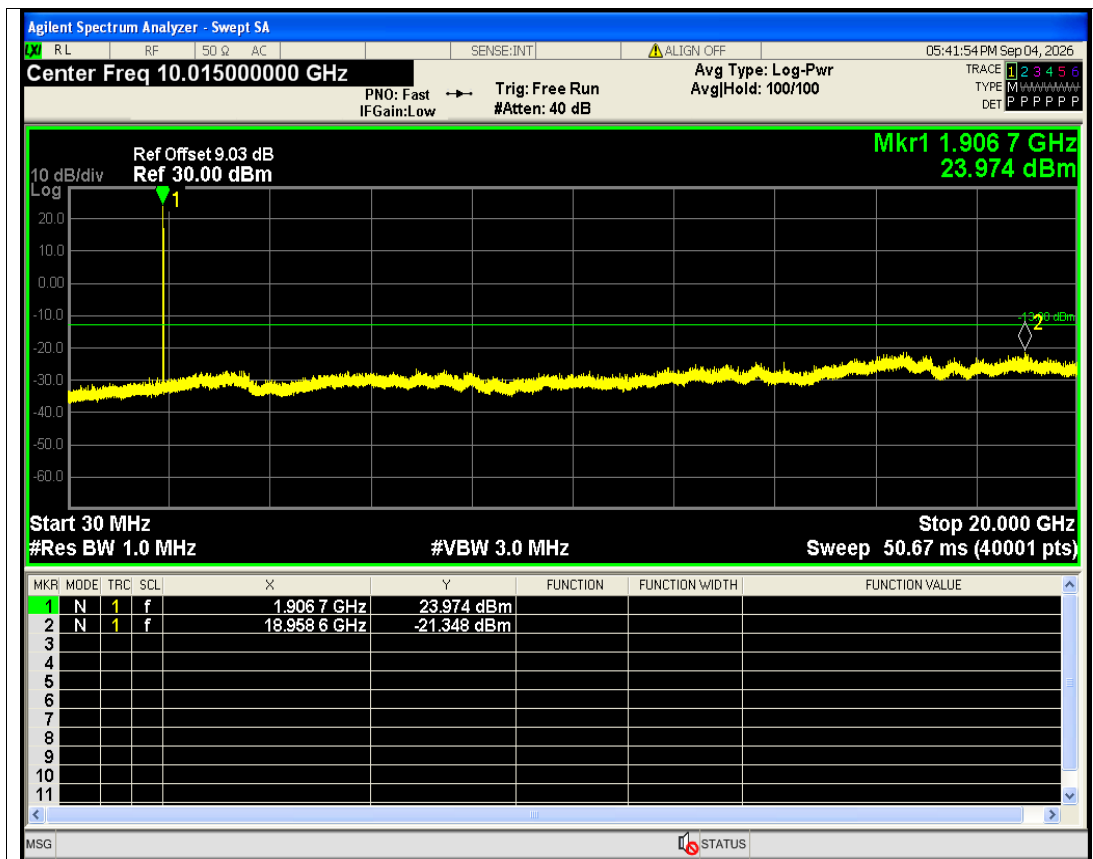
HSUPA Band2 Subtest4 Channel=9538 NVNT
