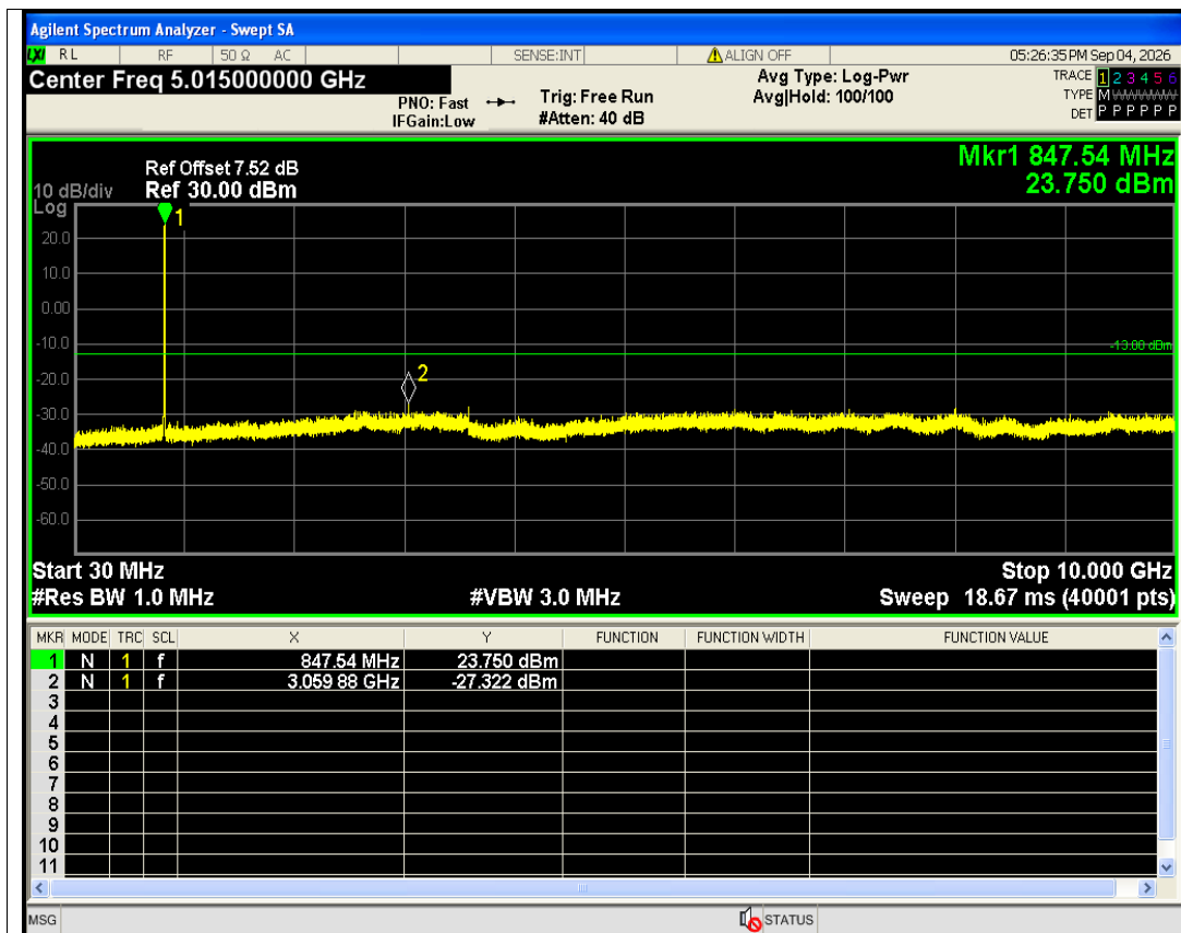
HSDPA Band5 Subtest2 Channel=4233 NVNT
