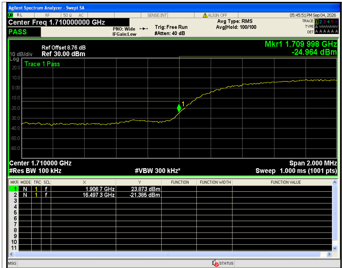
HSUPA Band4 Subtest4 Channel=1312 NVNT
