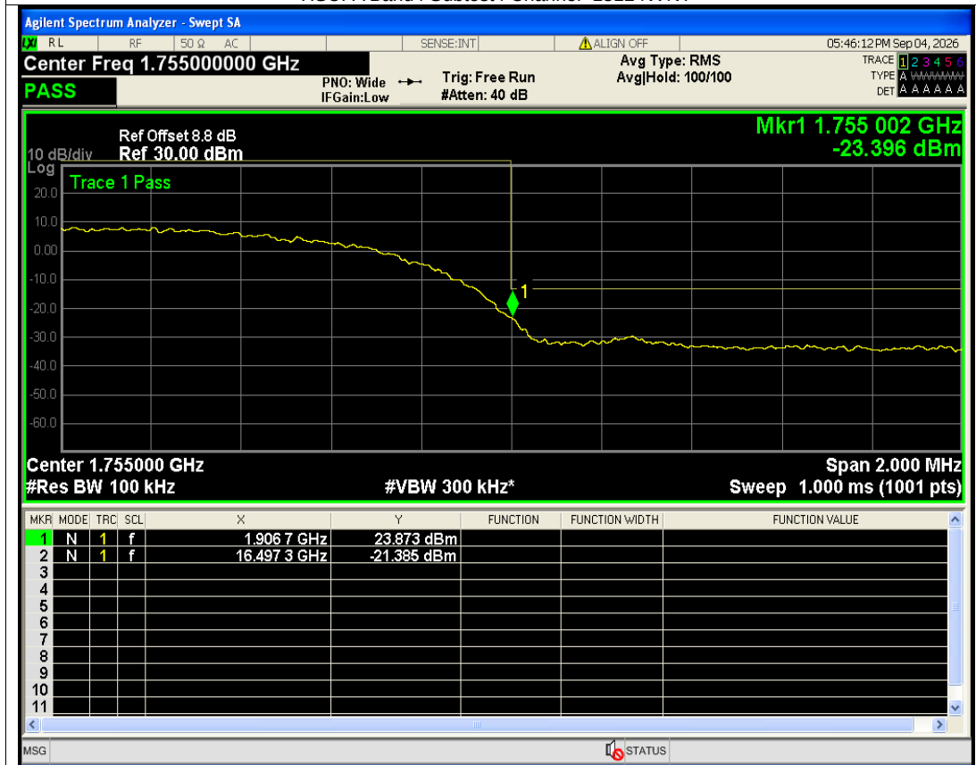
HSUPA Band4 Subtest4 Channel=1513 NVNT
