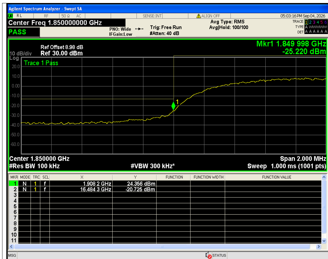
HSDPA Band2 Subtest3 Channel=9262 NVNT
