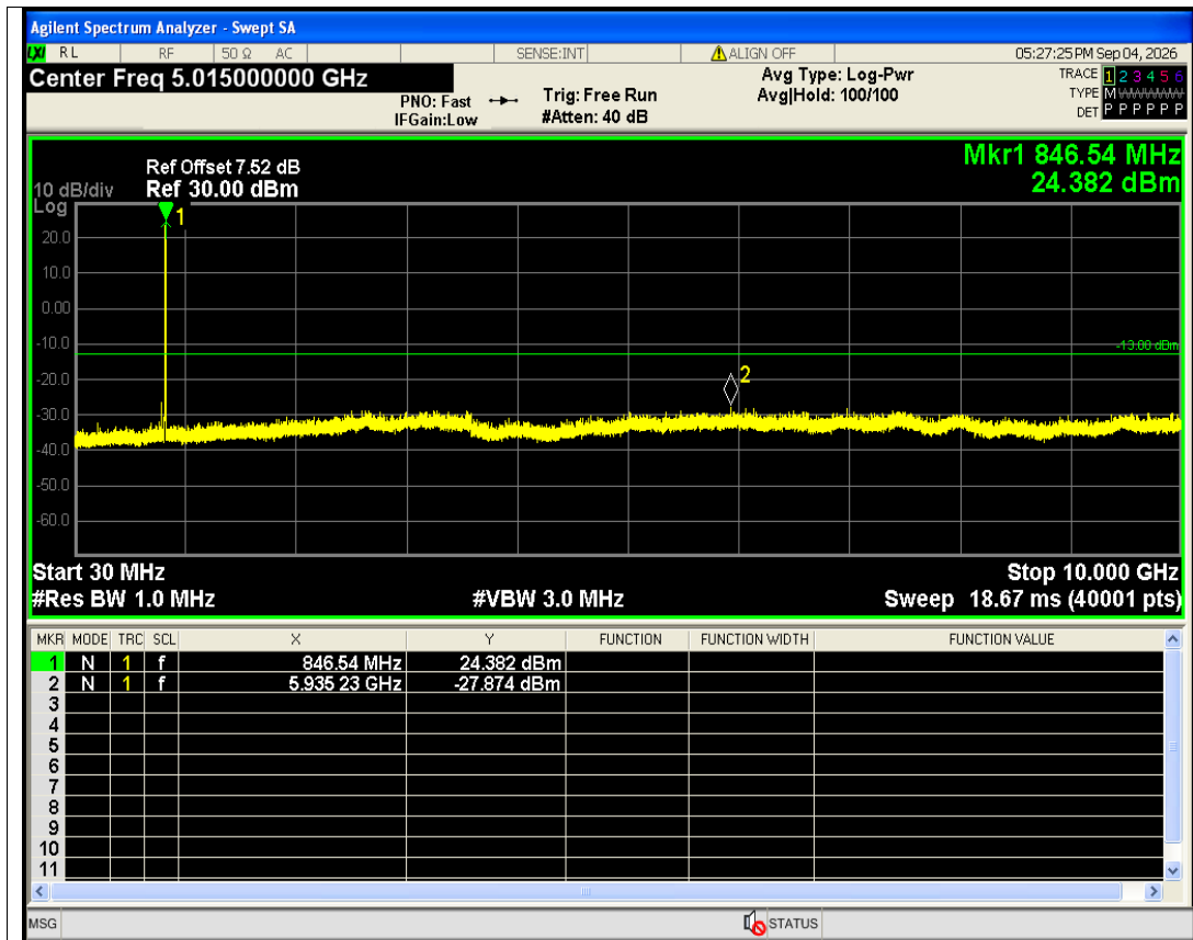
HSDPA Band5 Subtest4 Channel=4233 NVNT
