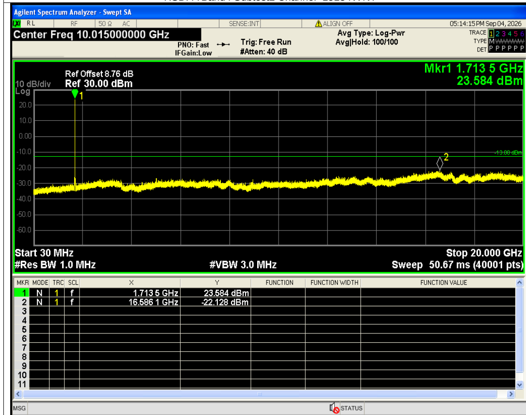
HSDPA Band4 Subtest3 Channel=1312 NVNT
