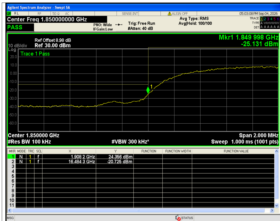
HSDPA Band2 Subtest1 Channel=9262 NVNT
