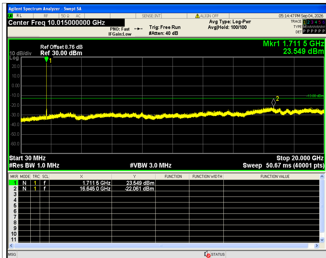
HSDPA Band4 Subtest4 Channel=1312 NVNT
