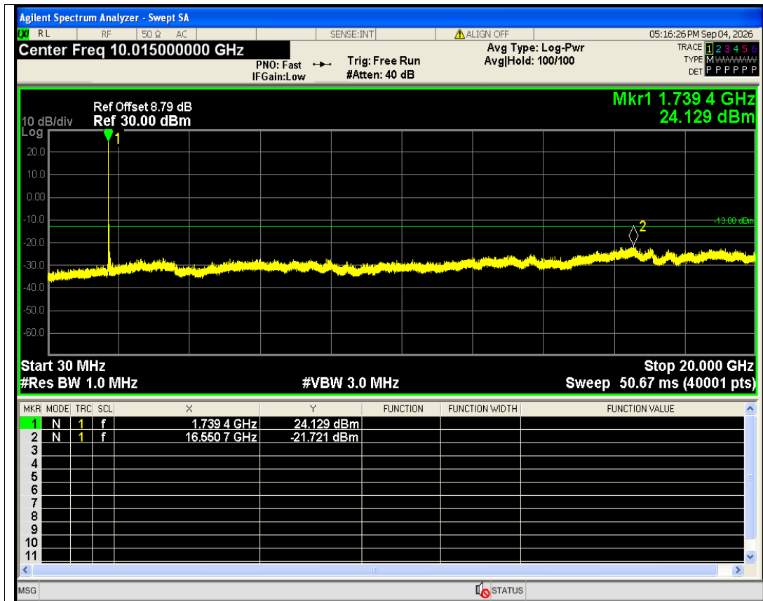
HSDPA Band4 Subtest3 Channel=1450 NVNT
