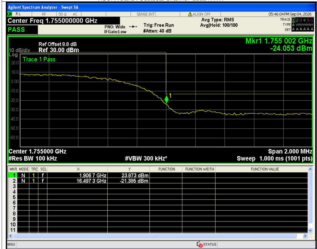
HSUPA Band4 Subtest2 Channel=1513 NVNT
