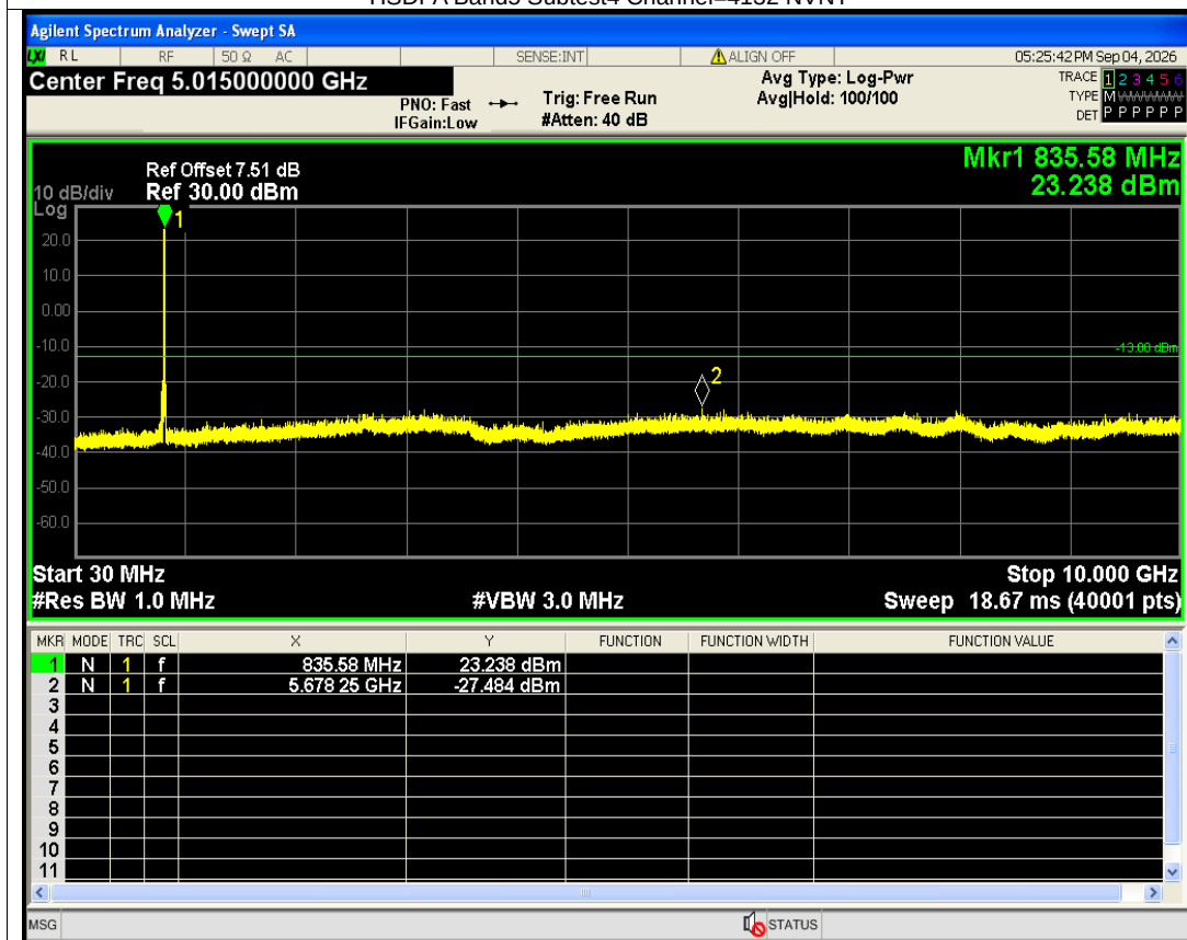
HSDPA Band5 Subtest4 Channel=4182 NVNT
