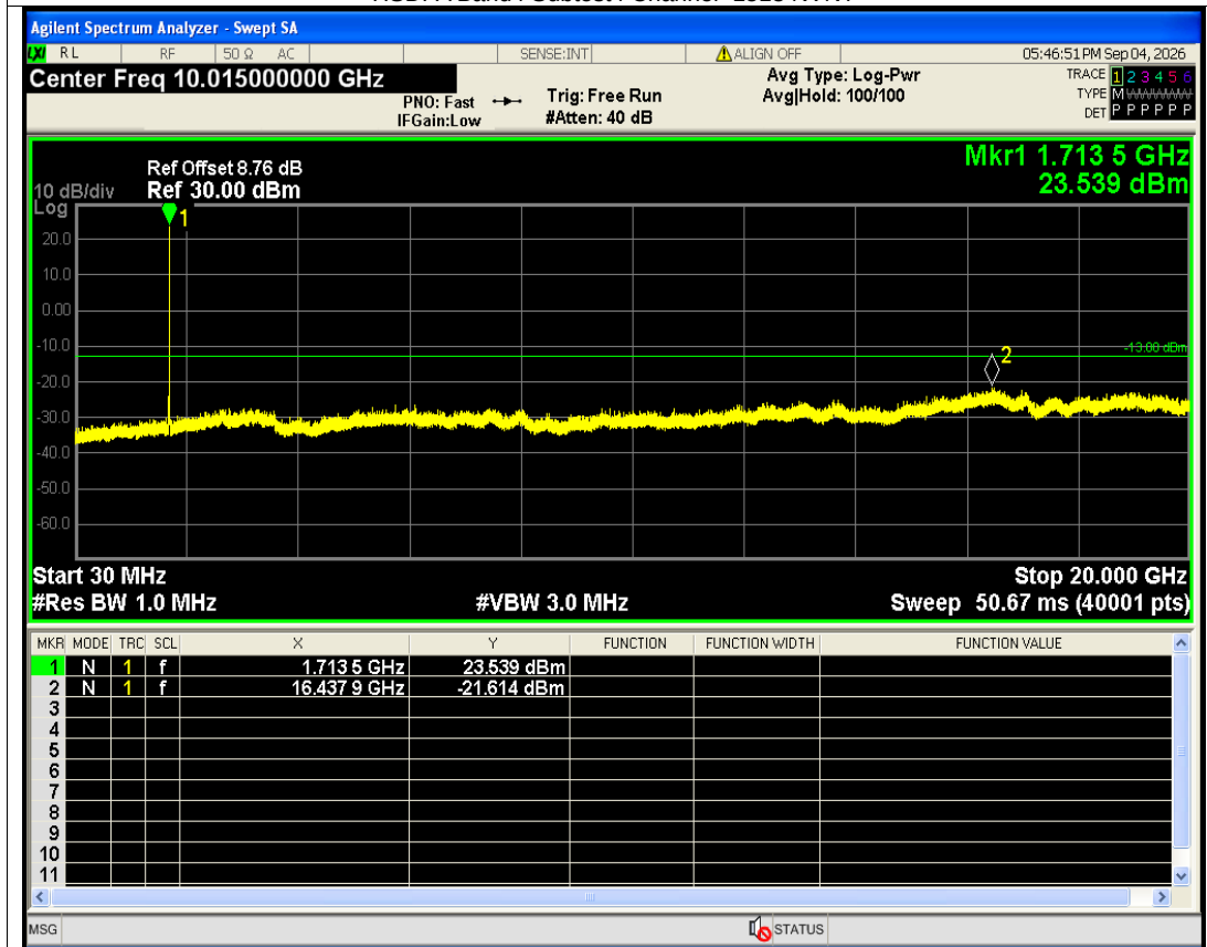
HSUPA Band4 Subtest1 Channel=1312 NVNT
