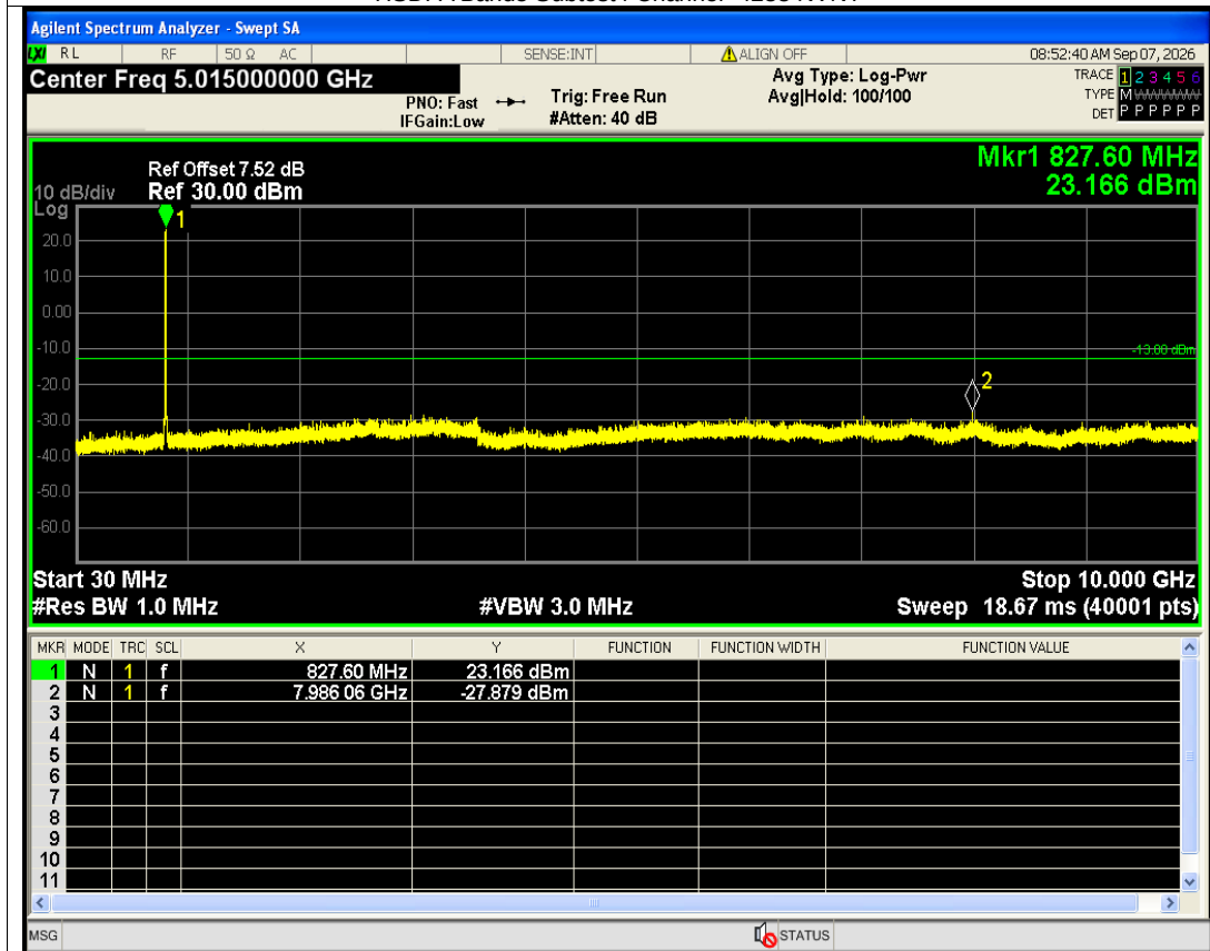
HSUPA Band5 Subtest1 Channel=4132 NVNT
