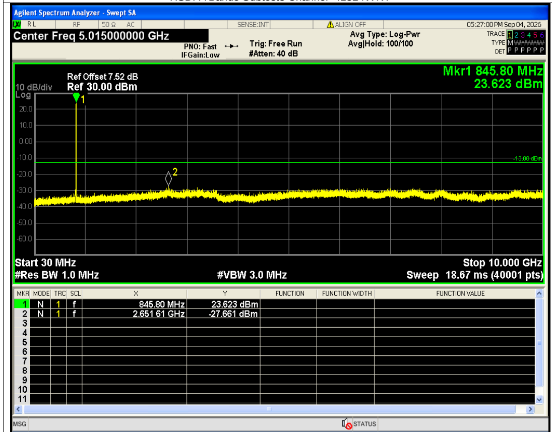
HSDPA Band5 Subtest3 Channel=4233 NVNT
