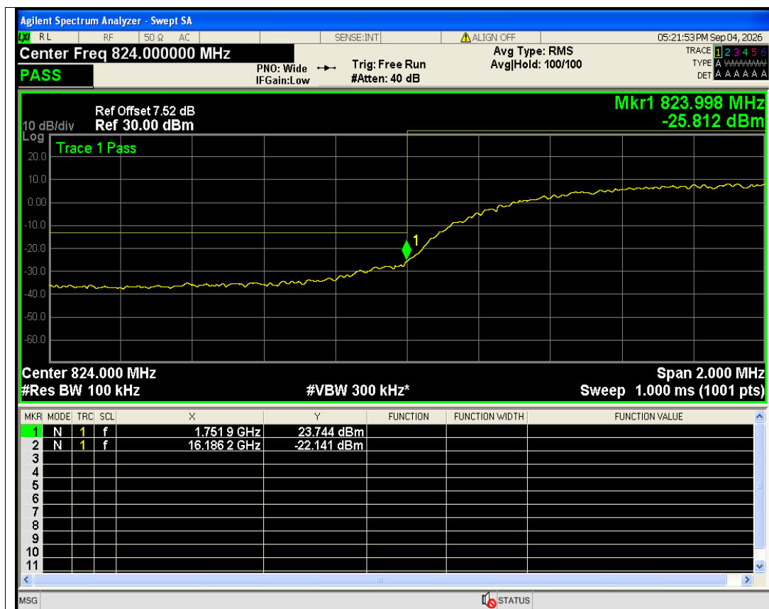
HSDPA Band5 Subtest2 Channel=4132 NVNT
