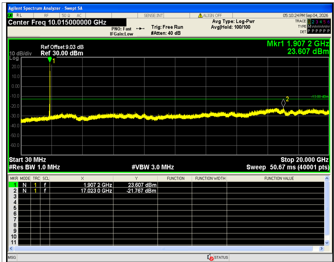
HSDPA Band2 Subtest4 Channel=9538 NVNT
