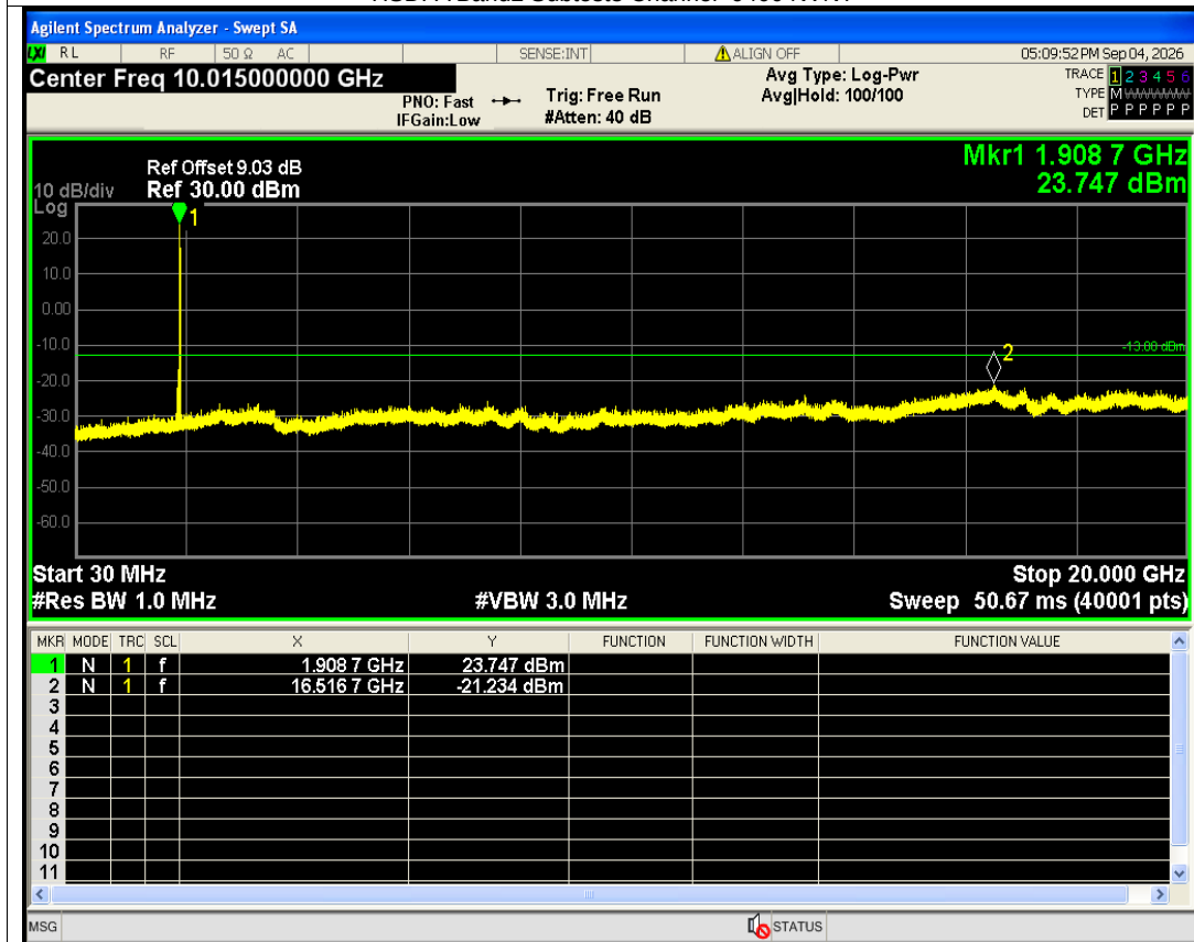
HSDPA Band2 Subtest3 Channel=9538 NVNT
