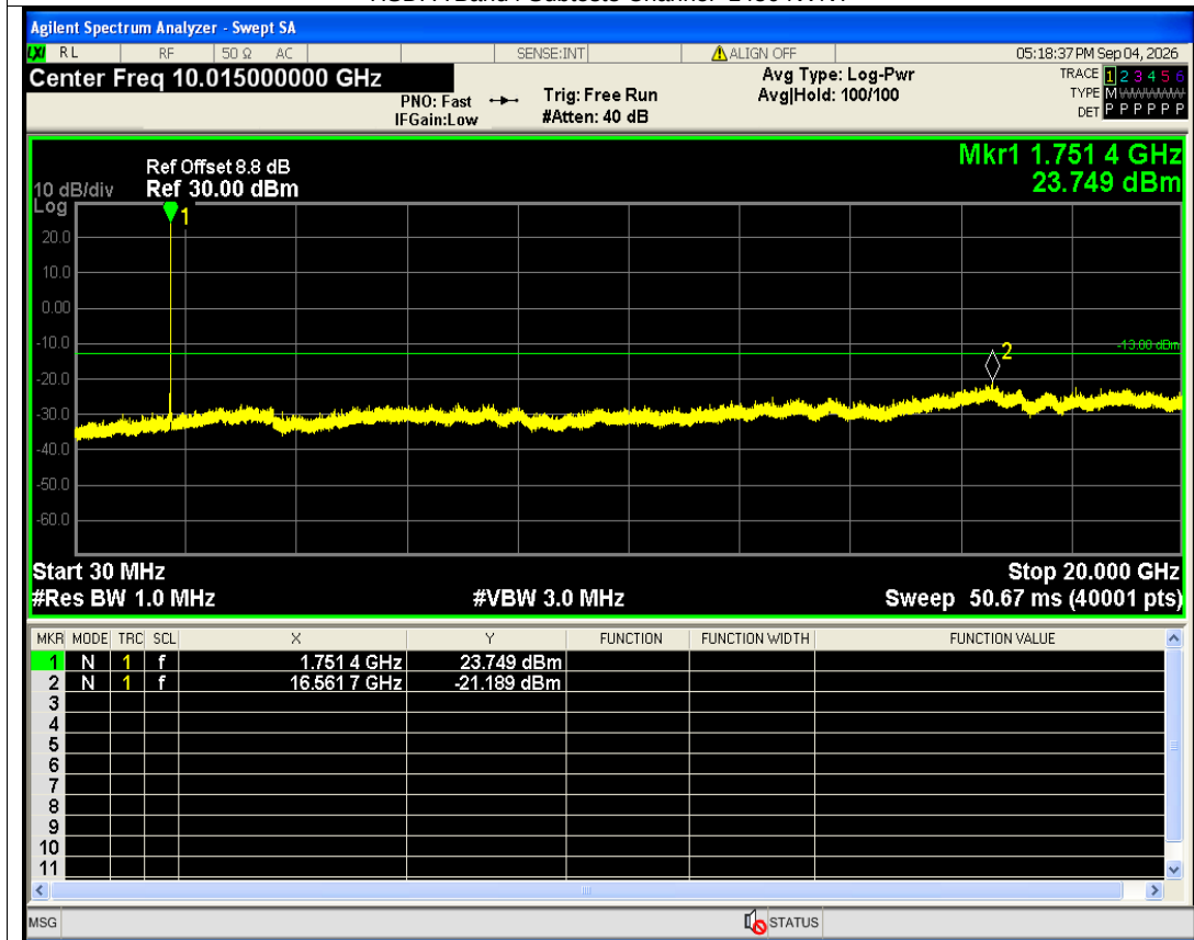
HSDPA Band4 Subtest3 Channel=1513 NVNT
