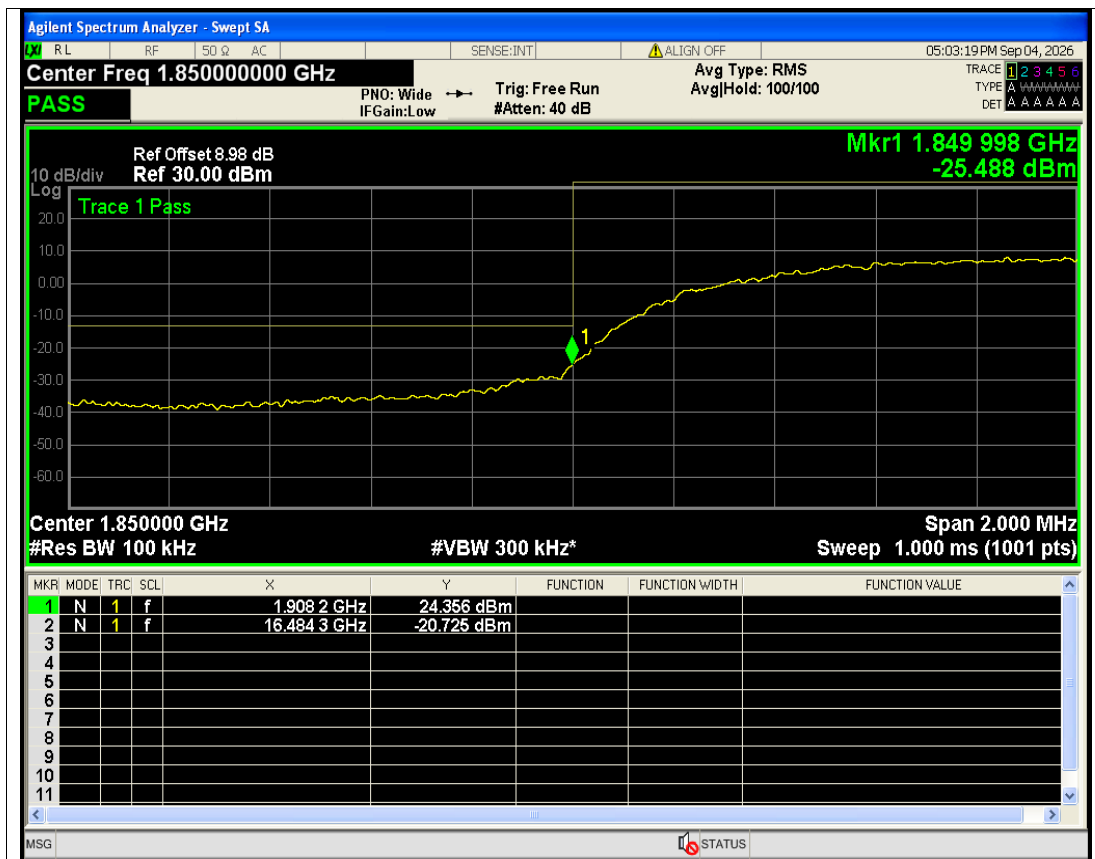
HSDPA Band2 Subtest4 Channel=9262 NVNT
