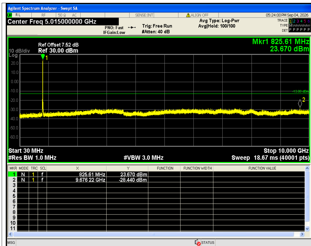
HSDPA Band5 Subtest4 Channel=4132 NVNT
