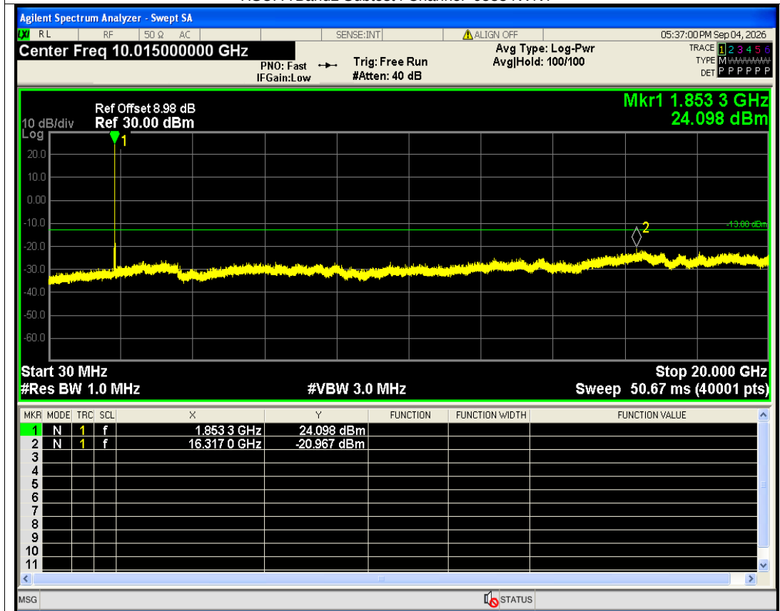
HSUPA Band2 Subtest5 Channel=9262 NVNT
