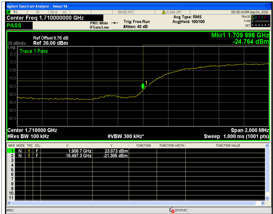
HSUPA Band4 Subtest2 Channel=1312 NVNT
