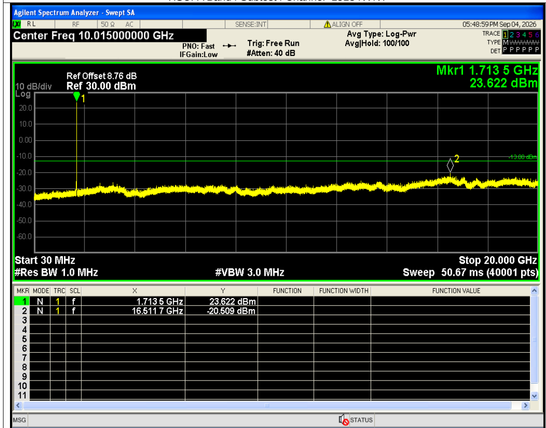
HSUPA Band4 Subtest5 Channel=1312 NVNT
