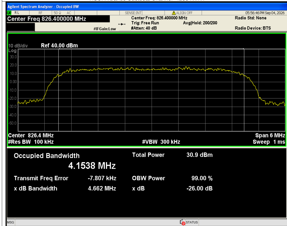
HSUPA Band5 Subtest3 Channel=4132 NVNT
