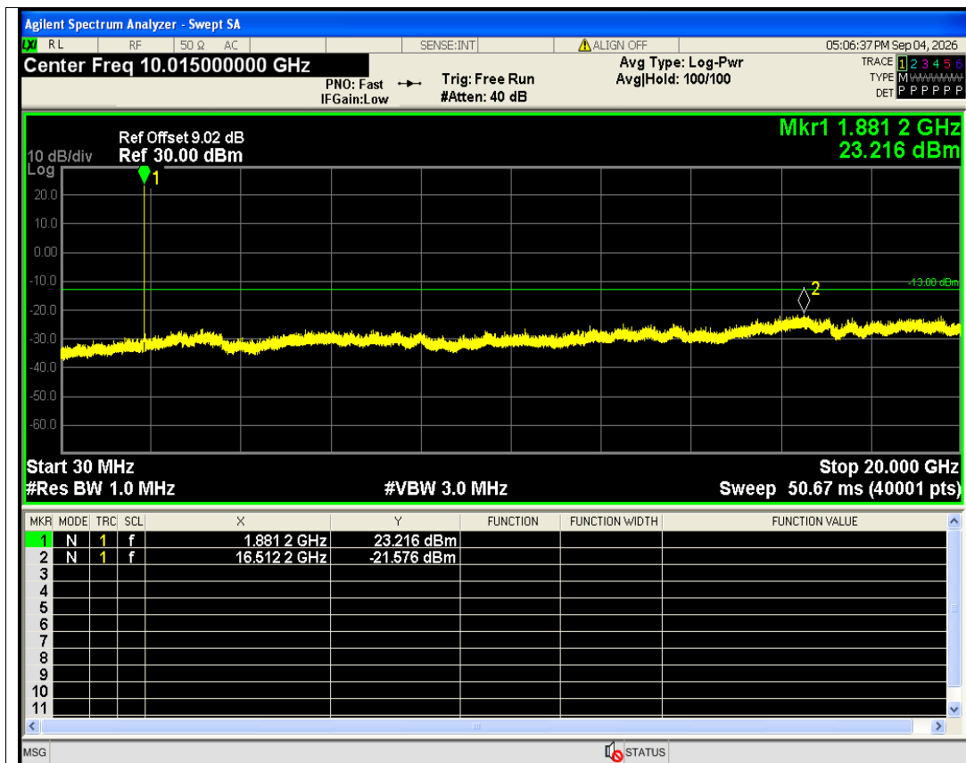
HSDPA Band2 Subtest1 Channel=9400 NVNT
