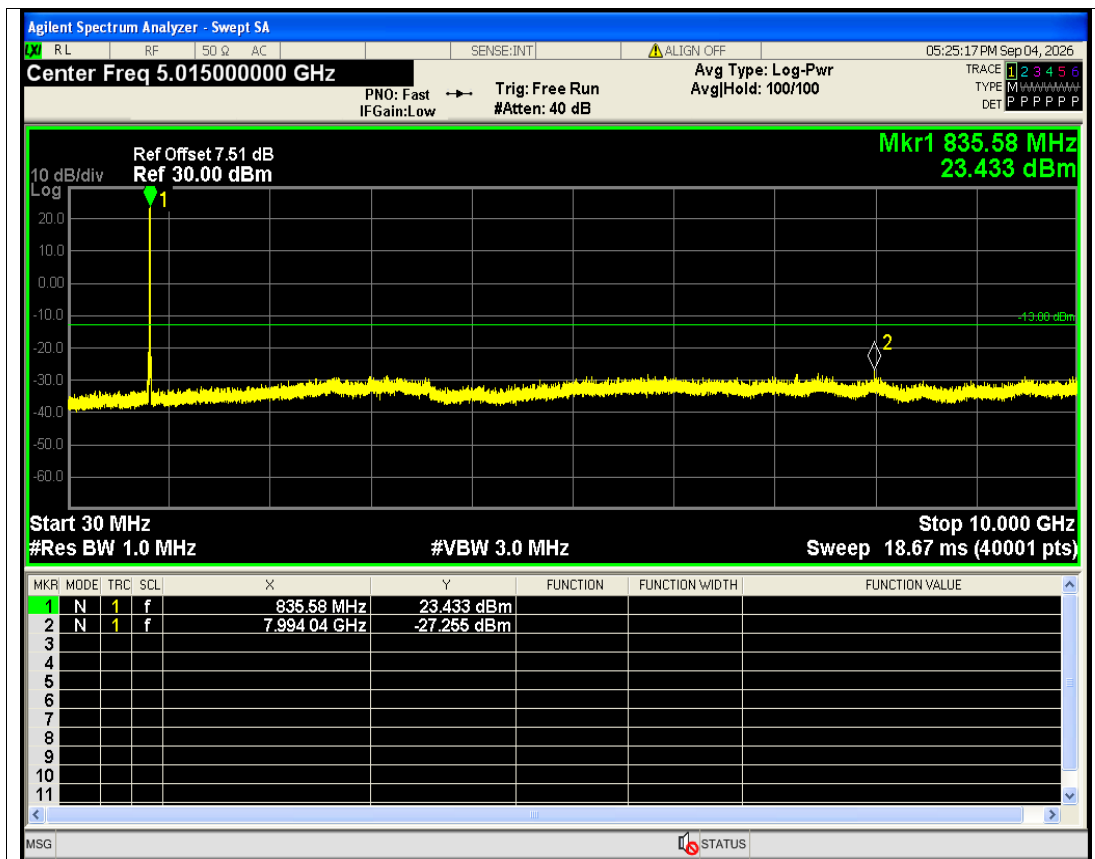
HSDPA Band5 Subtest3 Channel=4182 NVNT
