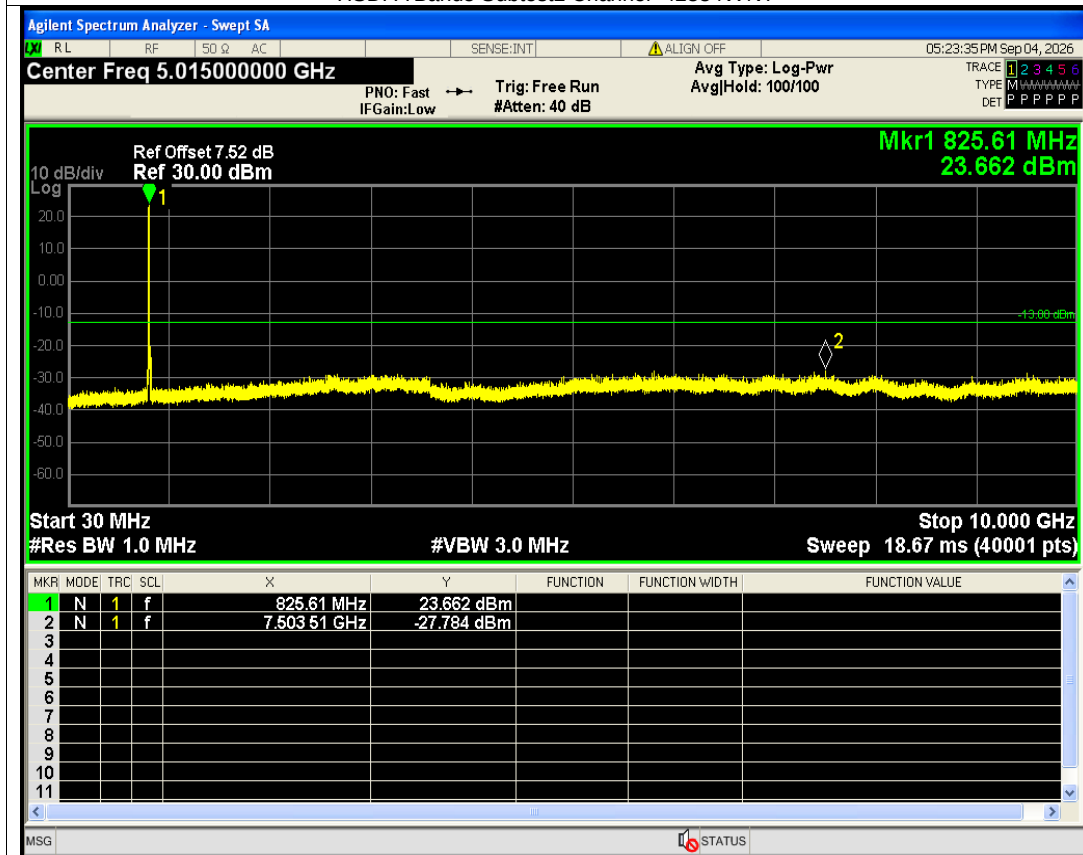
HSDPA Band5 Subtest3 Channel=4132 NVNT
