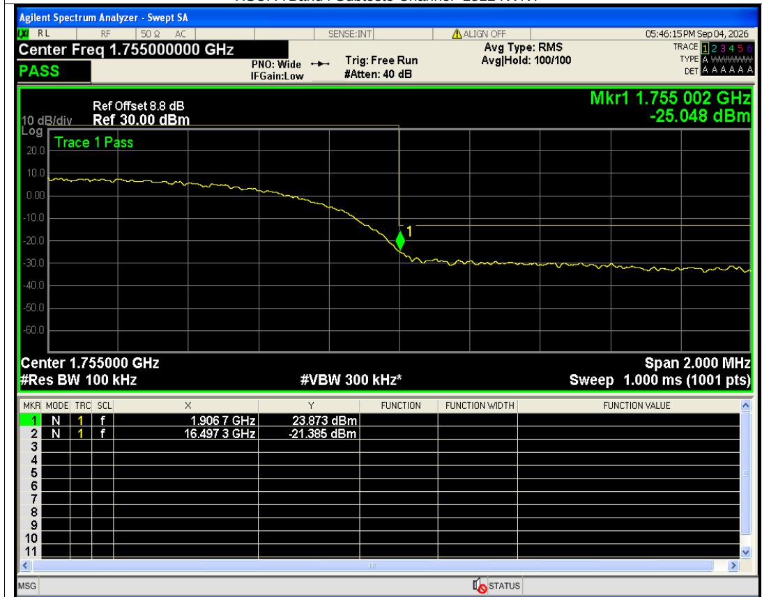
HSUPA Band4 Subtest5 Channel=1513 NVNT
