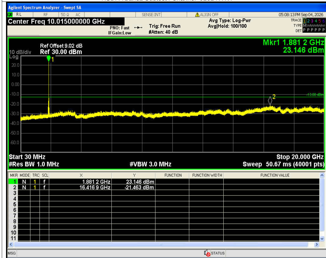
HSDPA Band2 Subtest4 Channel=9400 NVNT
