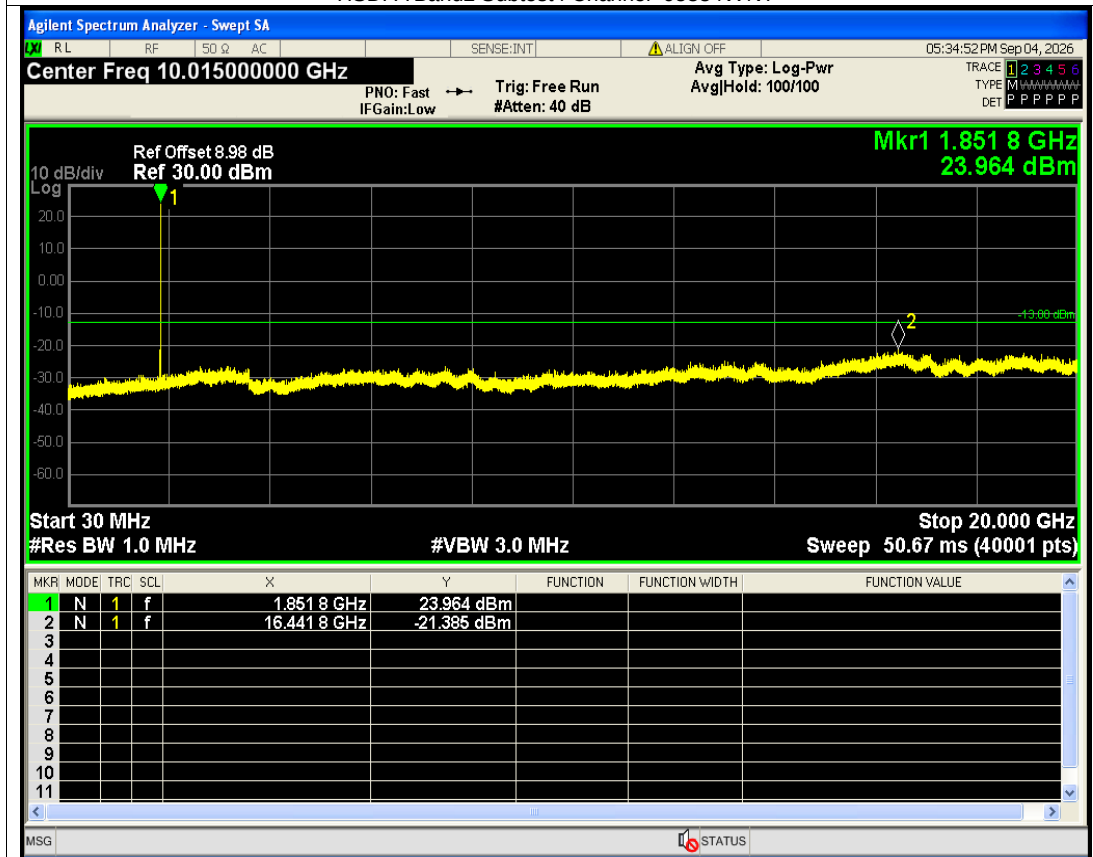
HSUPA Band2 Subtest1 Channel=9262 NVNT
