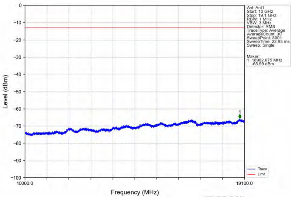
Band2_3MHz_QPSK_LCH_1851.5MHz_RB_15_0_NTNV
