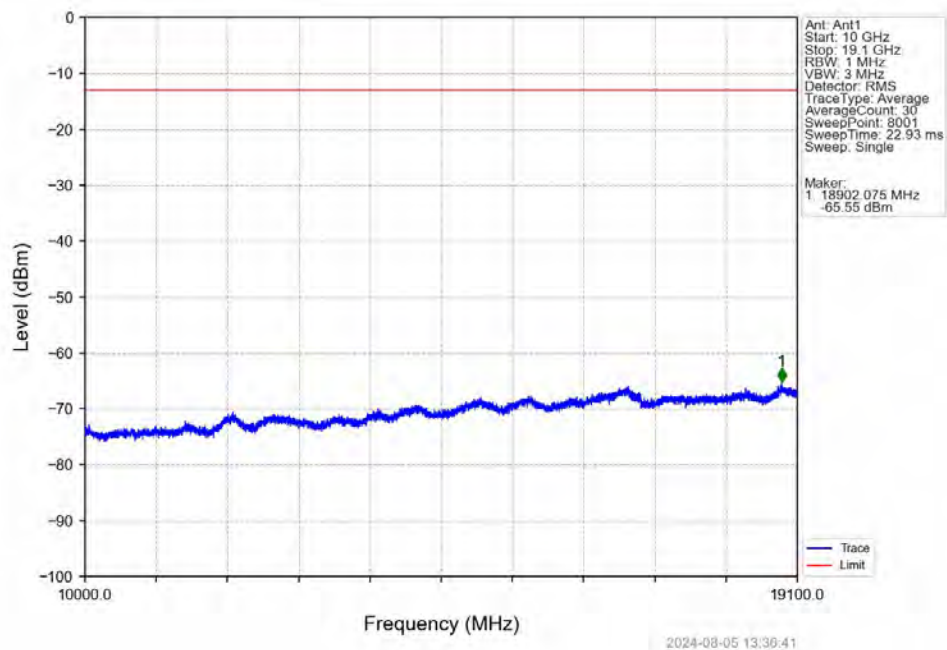
Band2_1.4MHz_16QAM_LCH_1850.7MHz_RB_6_0_NTNV
