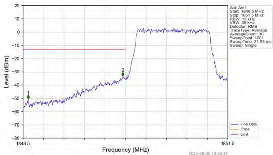
Band2_1.4MHz_16QAM_LCH_1850.7MHz_RB_6_0_NTNV
