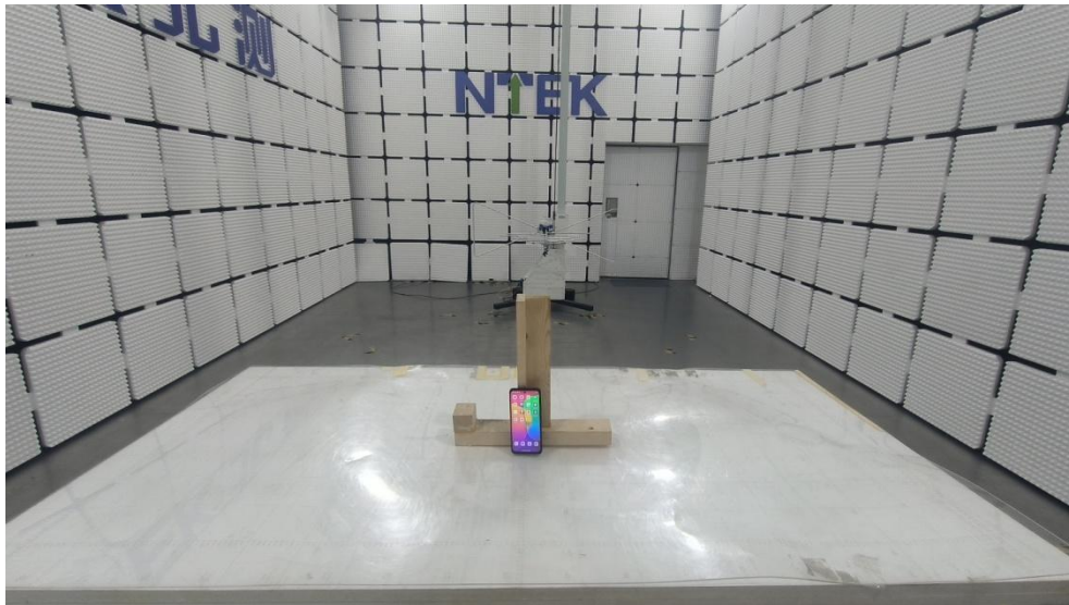
Radiated Measurement Photos(30MHz~1GHz )
