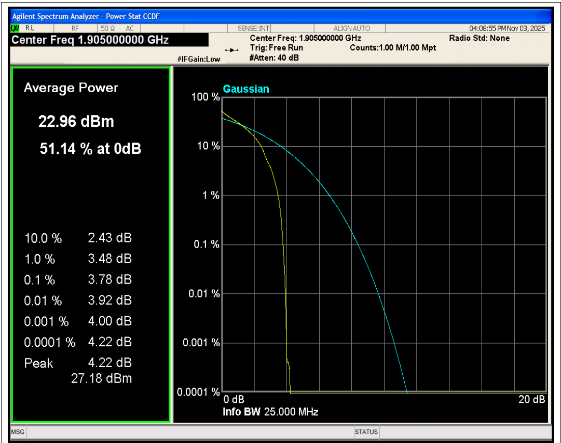
Band2 QPSK BW=10MHz Channel=19150 RB Size=1 Position=#0
