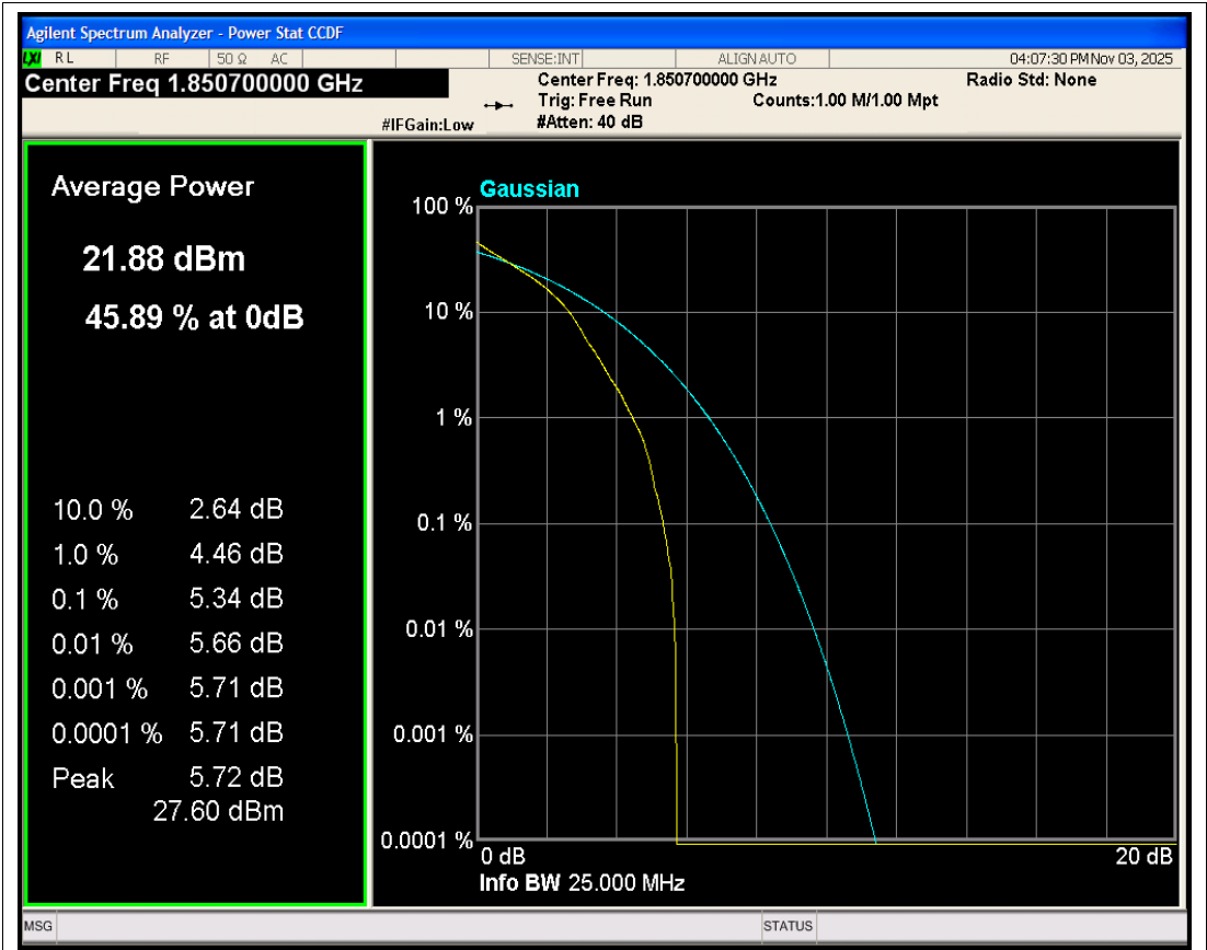
Band2 QPSK BW=1.4MHz Channel=18607 RB Size=1 Position=#0
