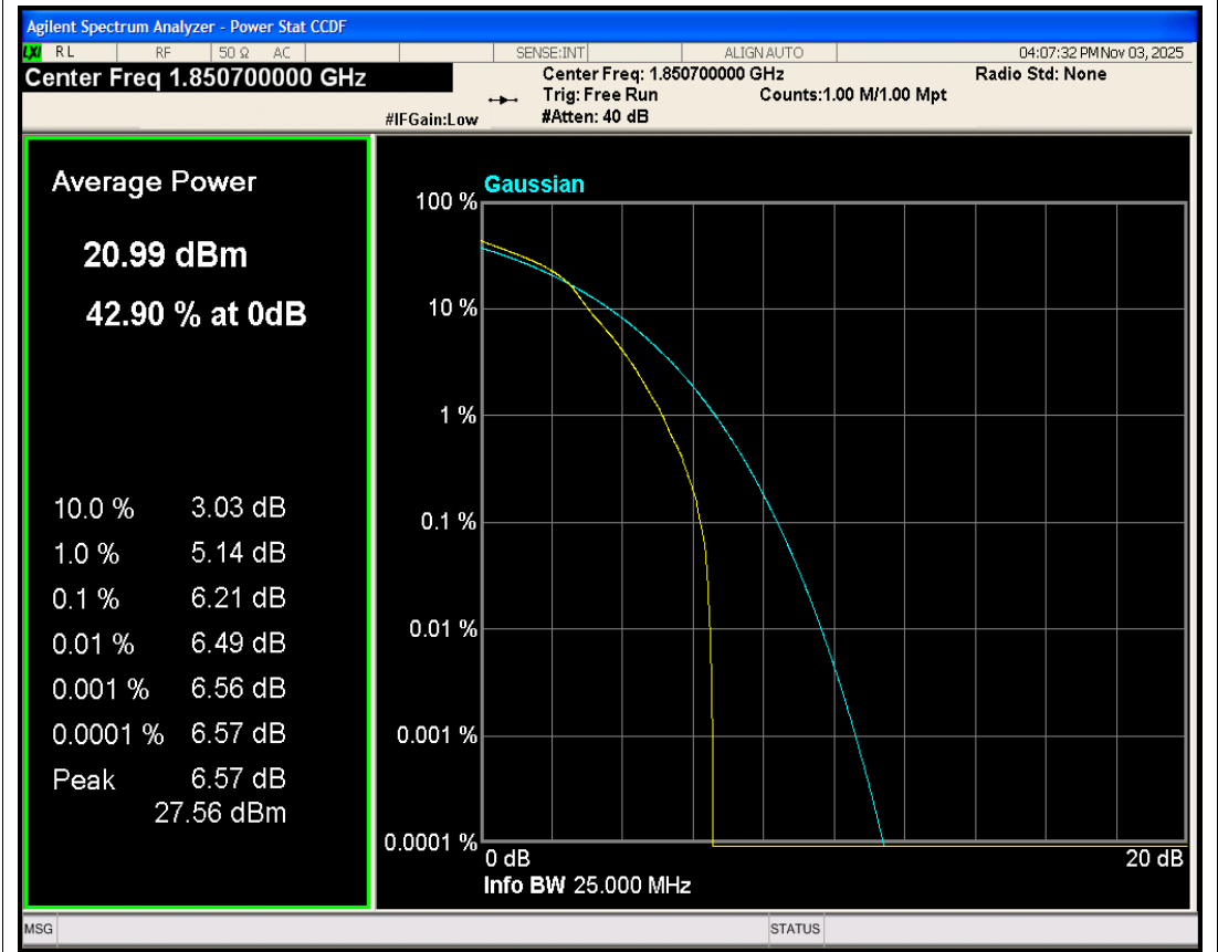
Band2 16QAM BW=1.4MHz Channel=18607 RB Size=1 Position=#0
