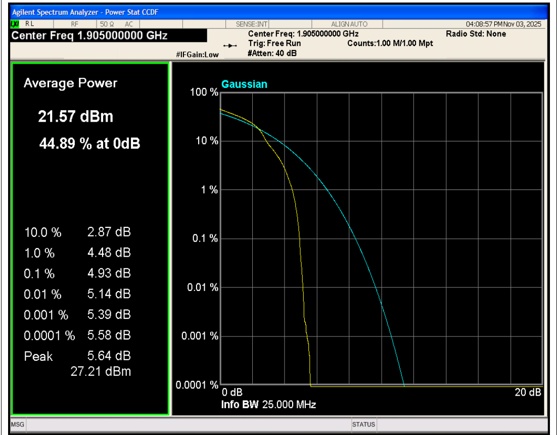
Band2 16QAM BW=10MHz Channel=19150 RB Size=1 Position=#0
