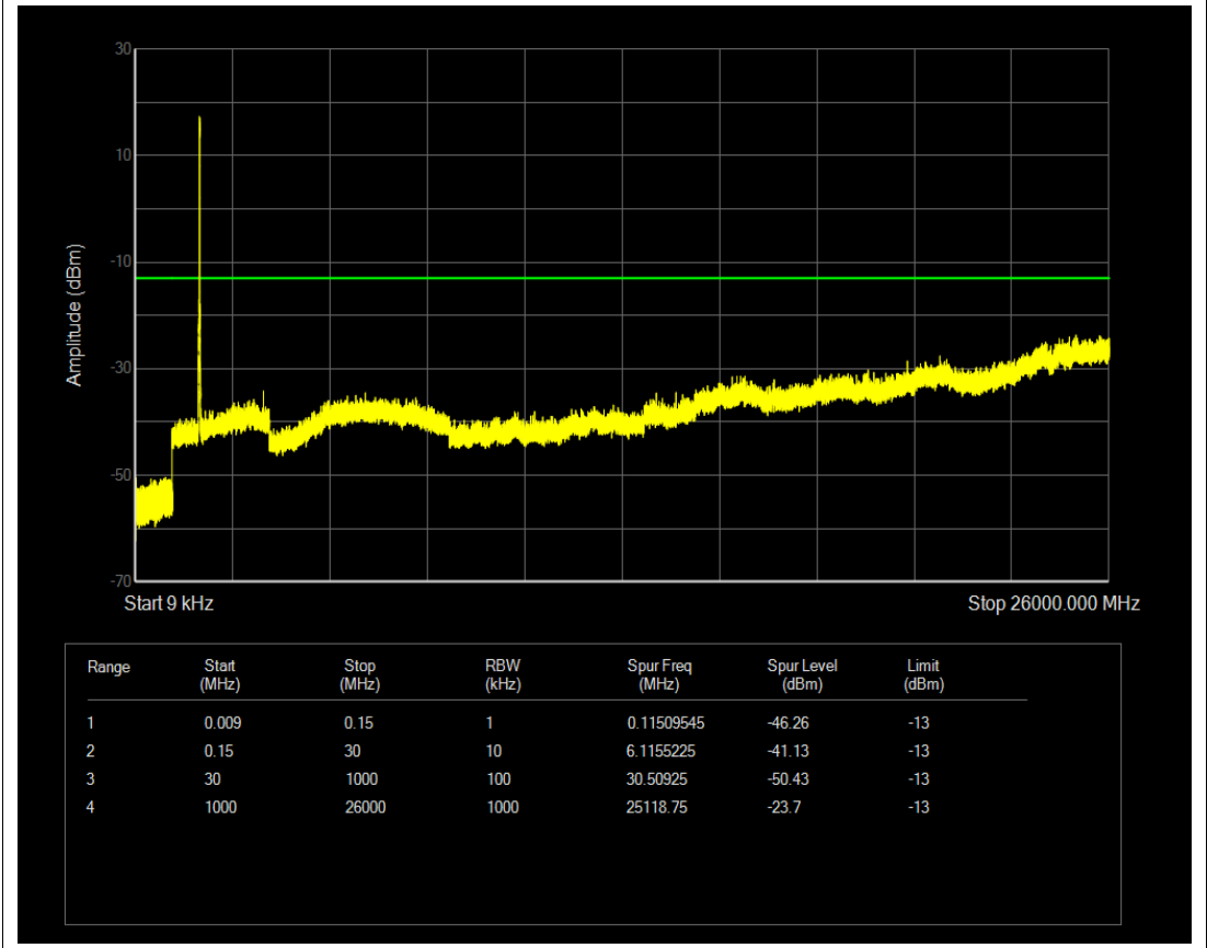
Band4 16QAM BW=15MHz Channel=20175 RB Size=75 Position=#0
