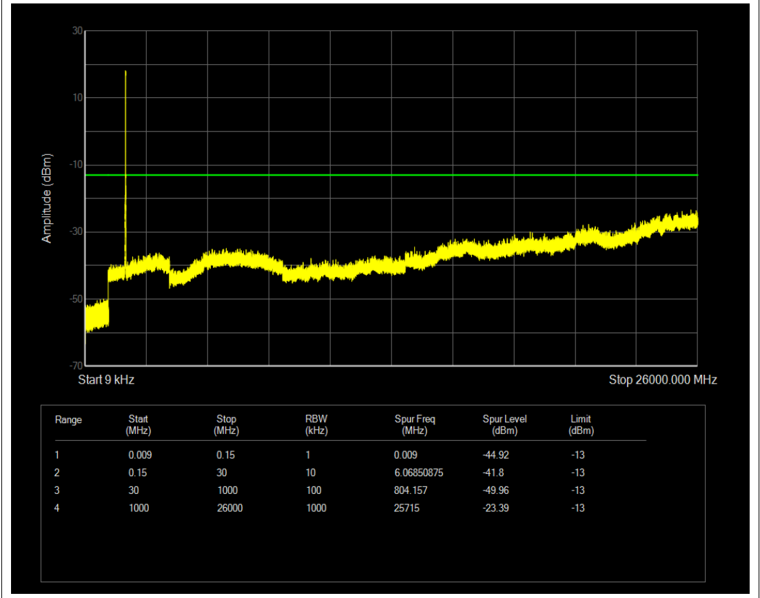
Band4 16QAM BW=10MHz Channel=20175 RB Size=50 Position=#0
