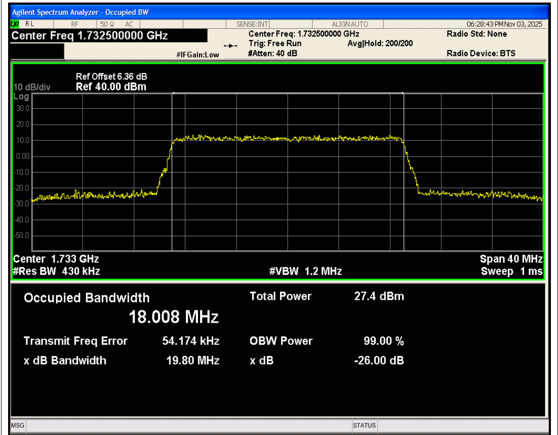
Band4 16QAM BW=20MHz Channel=20175 RB Size=100 Position=#0
