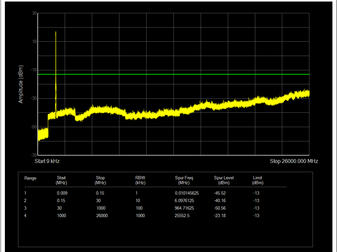
Band4 16QAM BW=20MHz Channel=20300 RB Size=100 Position=#0
