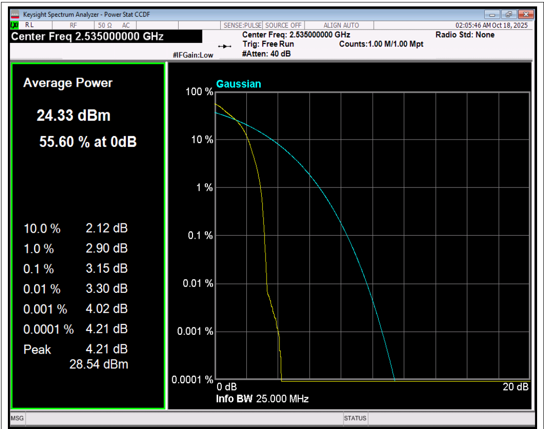
Band7 QPSK BW=20MHz Channel=21100 RB Size=1 Position=#0 NVNT
