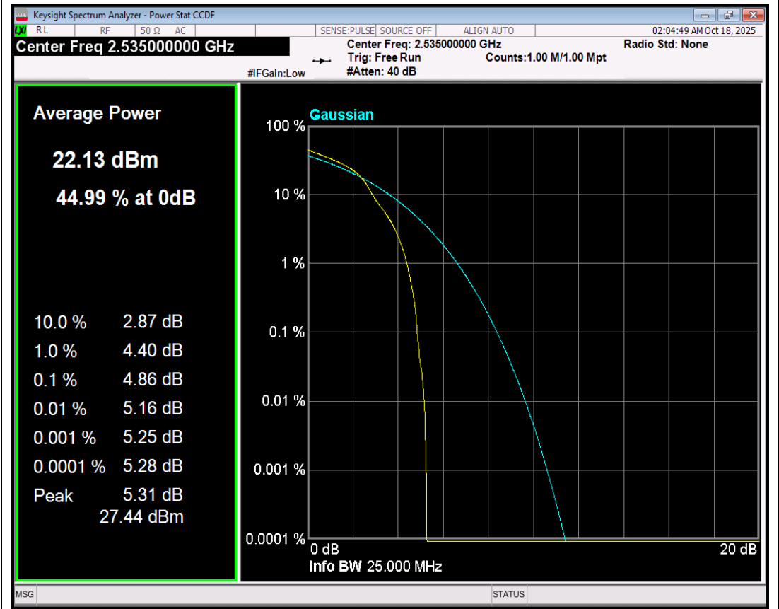
Band7 16QAM BW=5MHz Channel=21100 RB Size=1 Position=#0 NVNT
