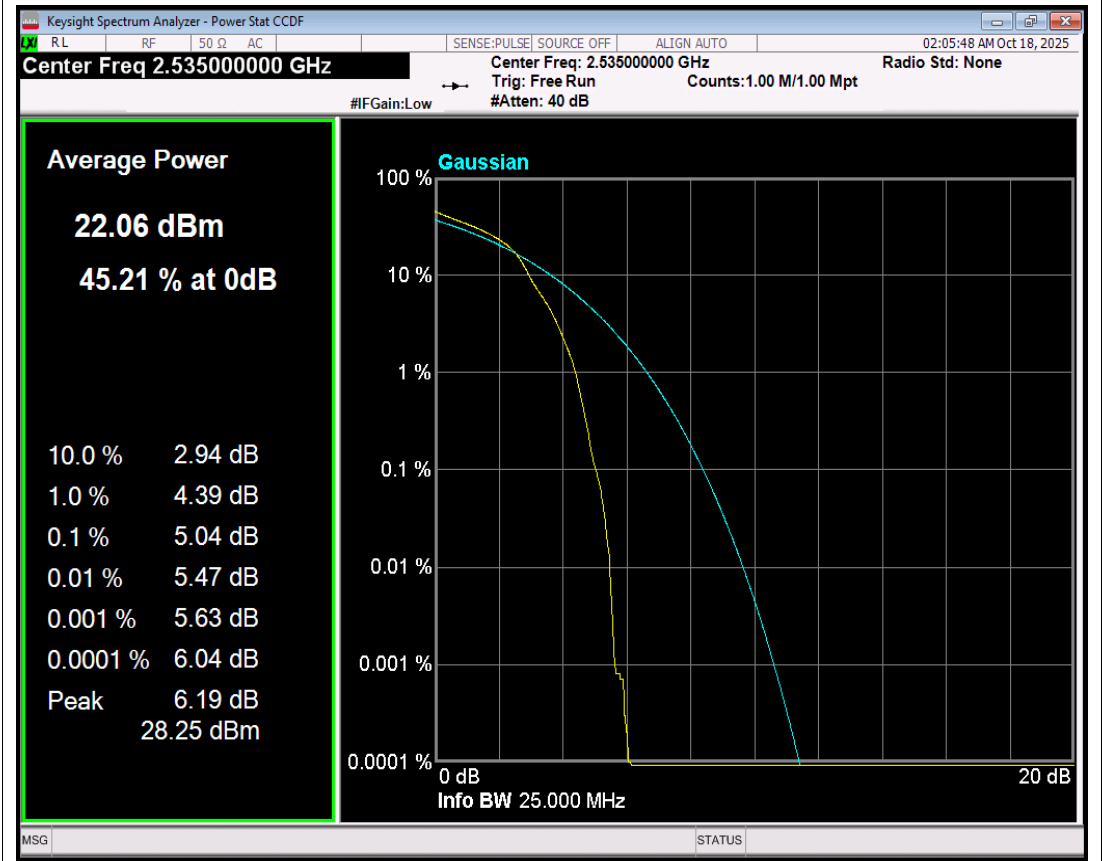
Band7 16QAM BW=20MHz Channel=21100 RB Size=1 Position=#0 NVNT
