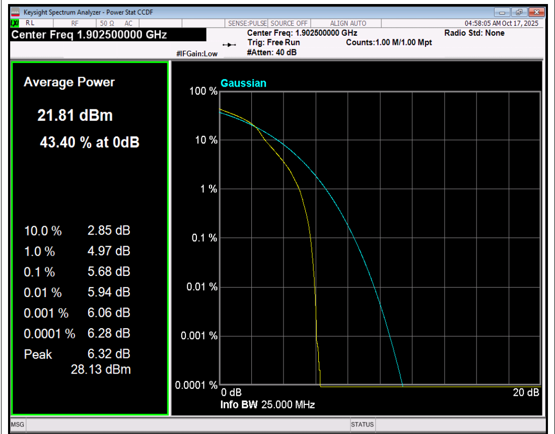
Band2 16QAM BW=15MHz Channel=19125 RB Size=1 Position=#0 NVNT
