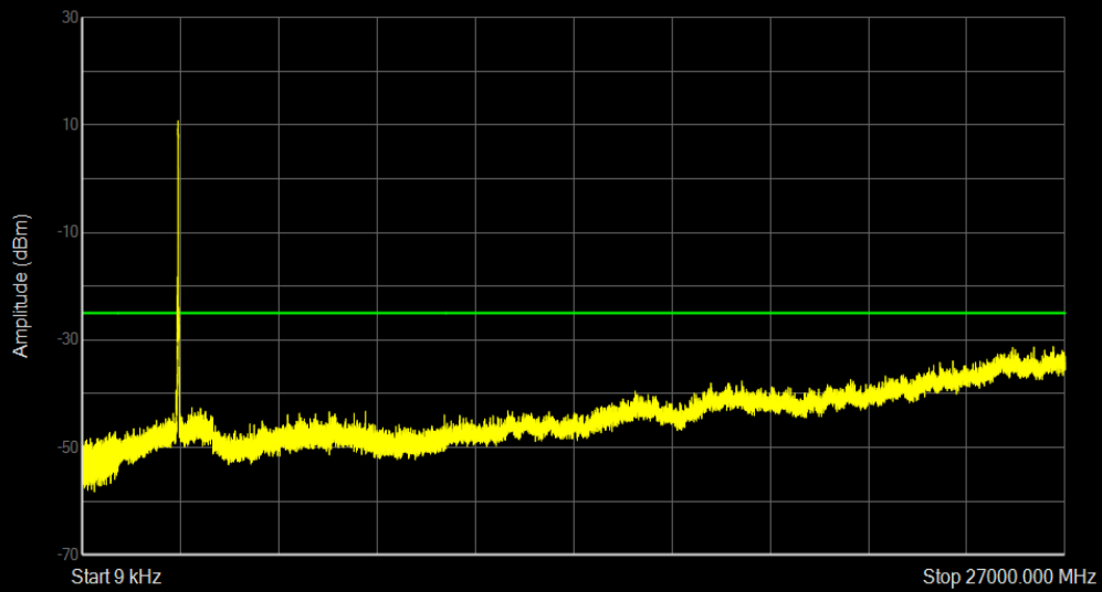
Band41(2535-2655) QPSK BW=15MHz Channel=41165 RB Size=75 Position=#0
