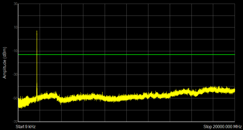
Band66 16QAM BW=15MHz Channel=132322 RB Size=75 Position=#0
