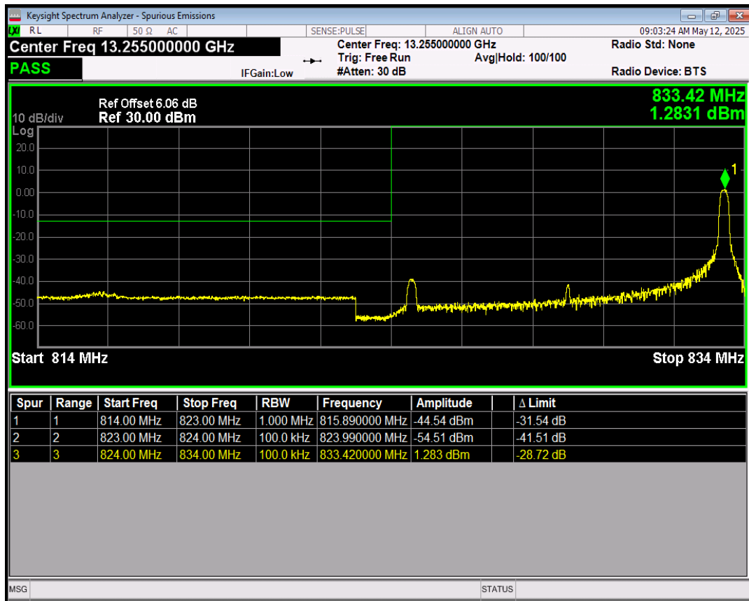
Band5 64QAM BW=10MHz Channel=20450 RB Size=50 Position=#0
