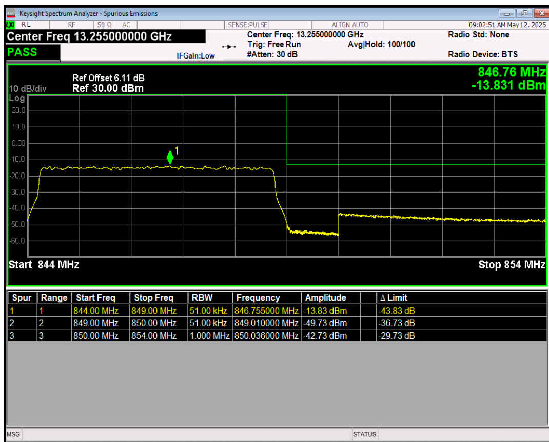
Band5 64QAM BW=5MHz Channel=20625 RB Size=1 Position=#0
