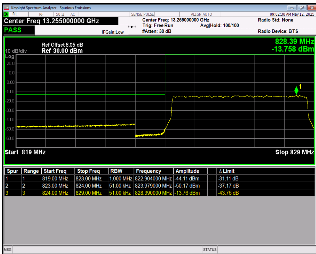
Band5 64QAM BW=5MHz Channel=20425 RB Size=1 Position=#0
