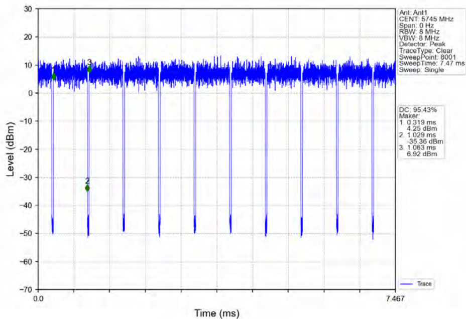
802.11ax(HEW20)_LCH_5745MHz_RU242_Left_Ant1_NTNV
