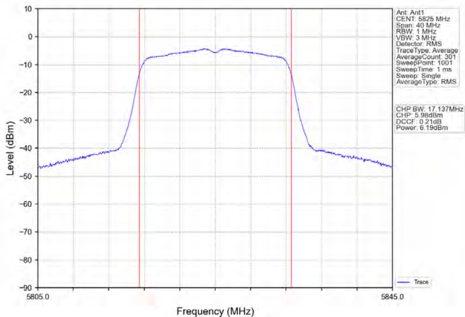
802.11ax(HEW20)_HCH_5825MHz_RU242_Left_Ant1_NTNV
