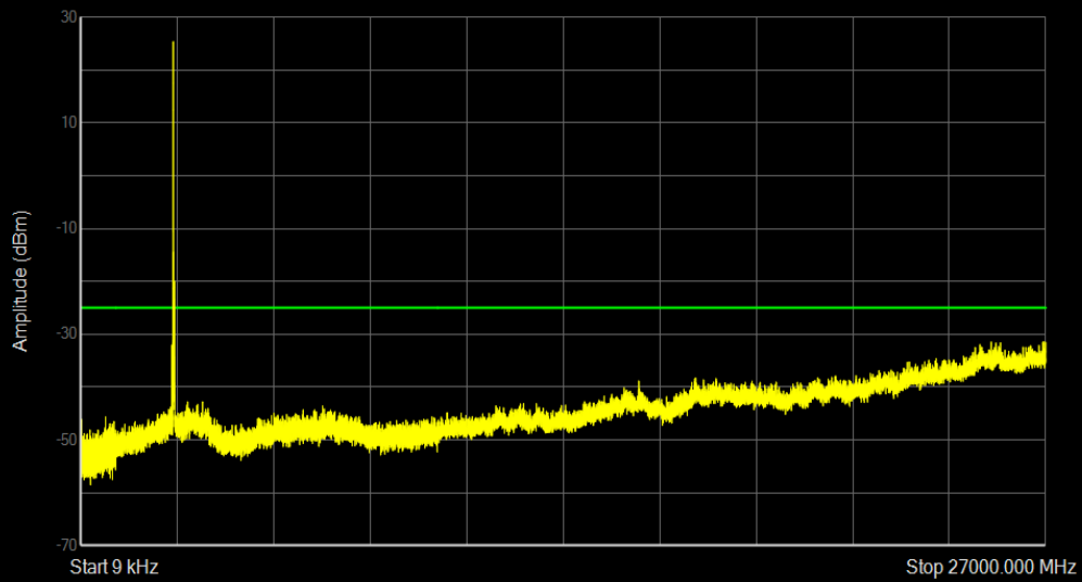
Band38 QPSK BW=20MHz Channel=38150 RB Size=1 Position=#0
