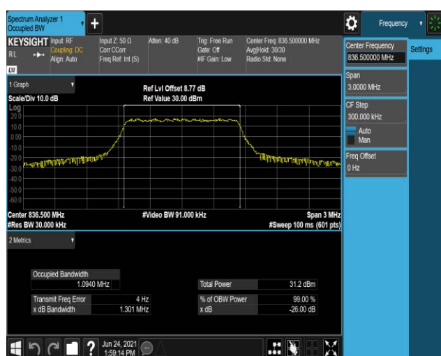
Band26-1.4MHz-QPSK-26915-6RB#0
