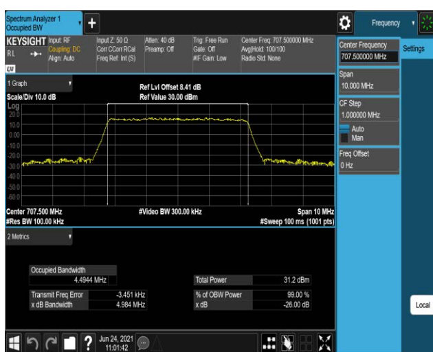
Band12-5MHz-16QAM-23095-25RB#0
