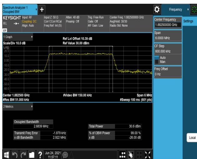
Band25-3MHz-16QAM-26365-15RB#0
