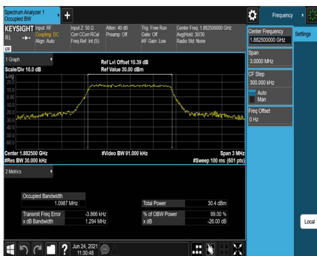
Band25-1.4MHz-16QAM-26365-6RB#0
