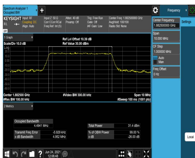
Band25-5MHz-16QAM-26365-25RB#0
