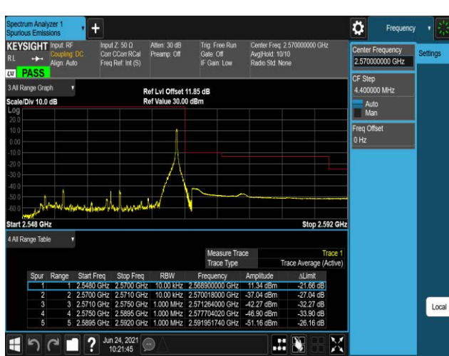
Band7-20MHz-QPSK-21350-1RB#99
