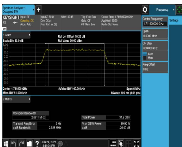
Band66-3MHz-QPSK-131987-15RB#0
