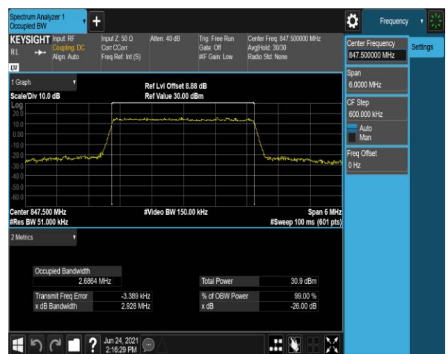
Band26-3MHz-16QAM-27025-15RB#0
