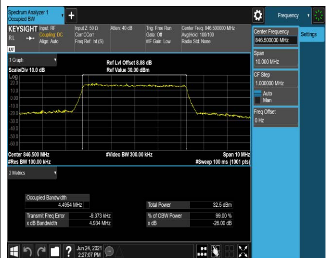
Band26-5MHz-QPSK-27015-25RB#0
