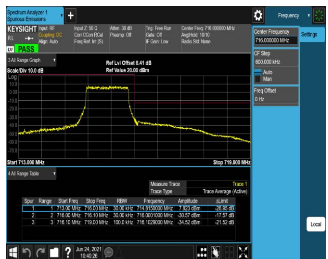
Band12-1.4MHz-QPSK-23173-6RB#0
