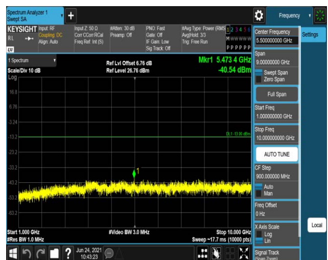
Band12-1.4MHz-QPSK-23173:1000~10000MHz
