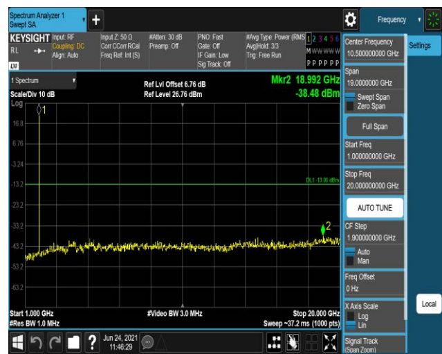
Band25-1.4MHz-16QAM-26365:1000~20000MHz
