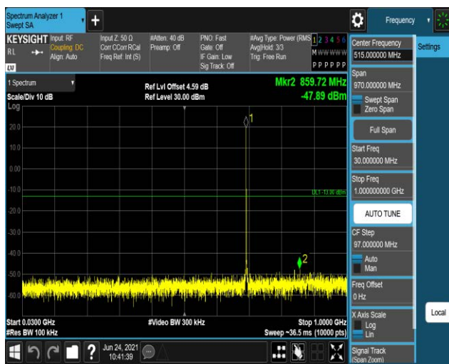
Band12-1.4MHz-16QAM-23095:30~1000MHz
