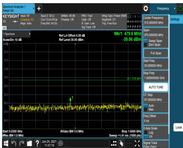
Band25-1.4MHz-16QAM-26683:30~1000MHz
