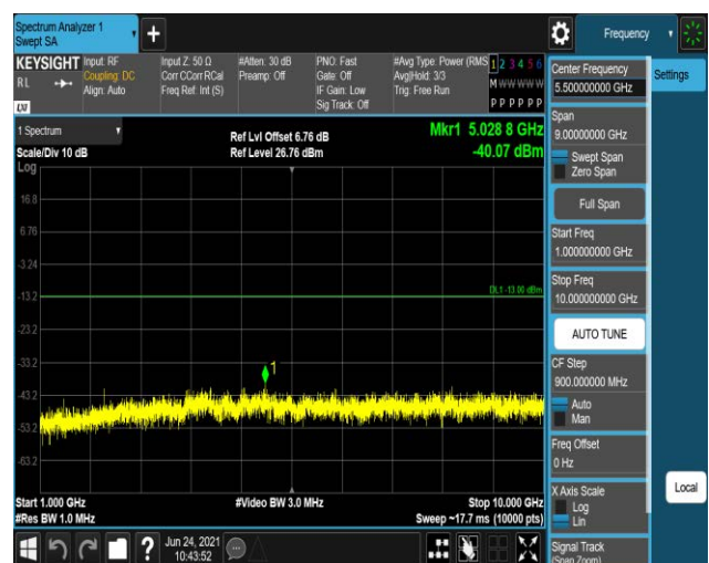
Band12-1.4MHz-16QAM-23173:1000~10000MHz
