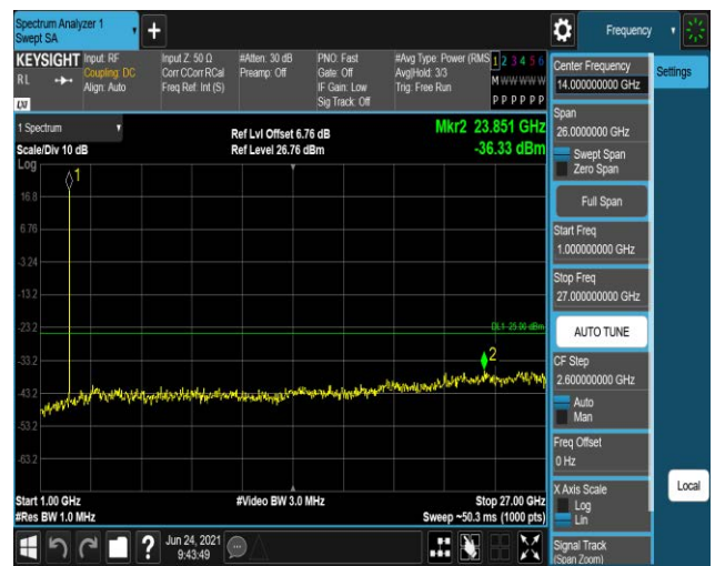
Band7-5MHz-QPSK-21100:1000~27000MHz
