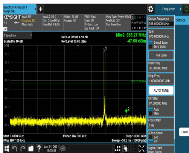
Band12-10MHz-QPSK-23095:30~1000MHz
