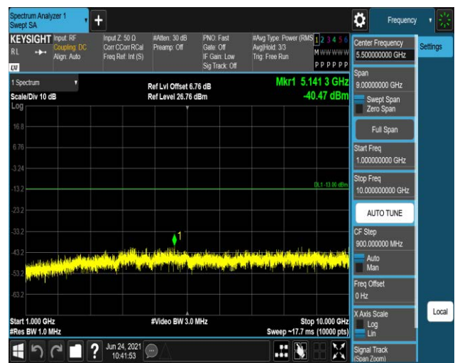
Band12-1.4MHz-16QAM-23095:1000~10000MHz
