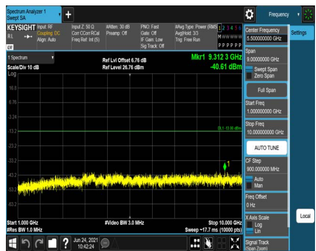
Band12-1.4MHz-QPSK-23173:1000~10000MHz
