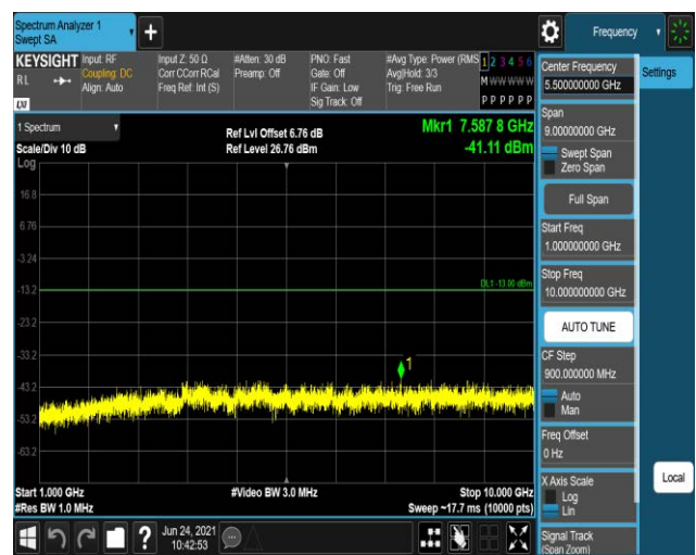
Band12-1.4MHz-16QAM-23173:1000~10000MHz
