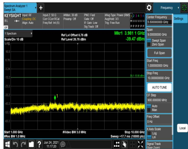
Band12-10MHz-16QAM-23130:1000~10000MHz
