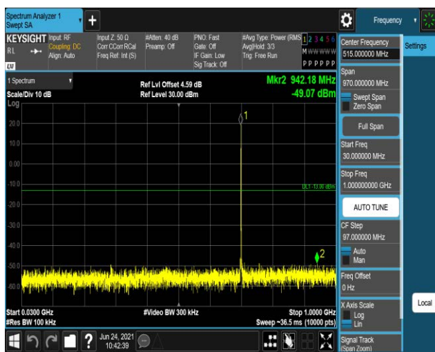
Band12-1.4MHz-16QAM-23173:30~1000MHz
