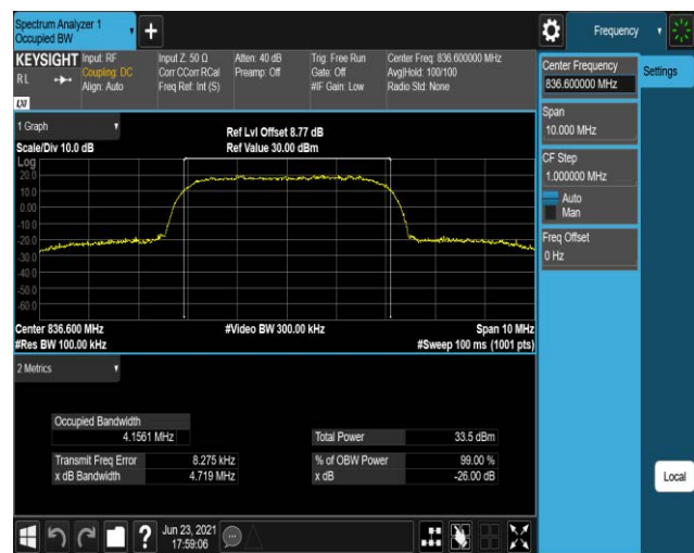
Band5-4183-4.719
