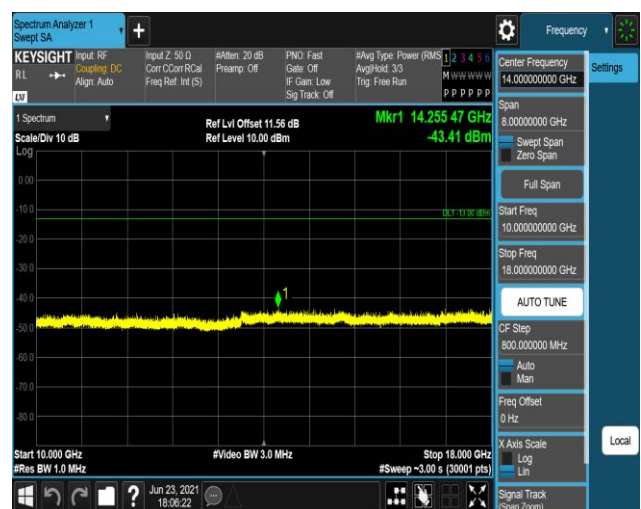
Band5-4233-10000~18000MHz
