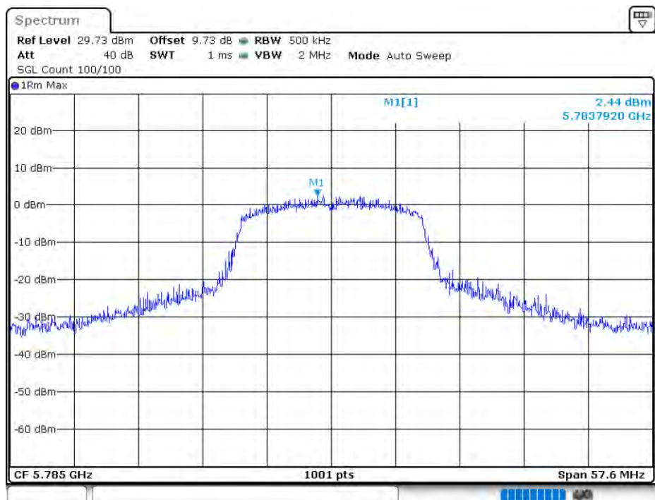
PSD NVNT 802.11a 5785MHz Ant1
