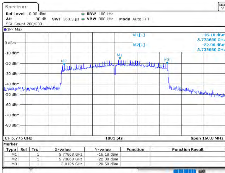
EBW NVNT 802.11ac80 5775MHz Ant1
