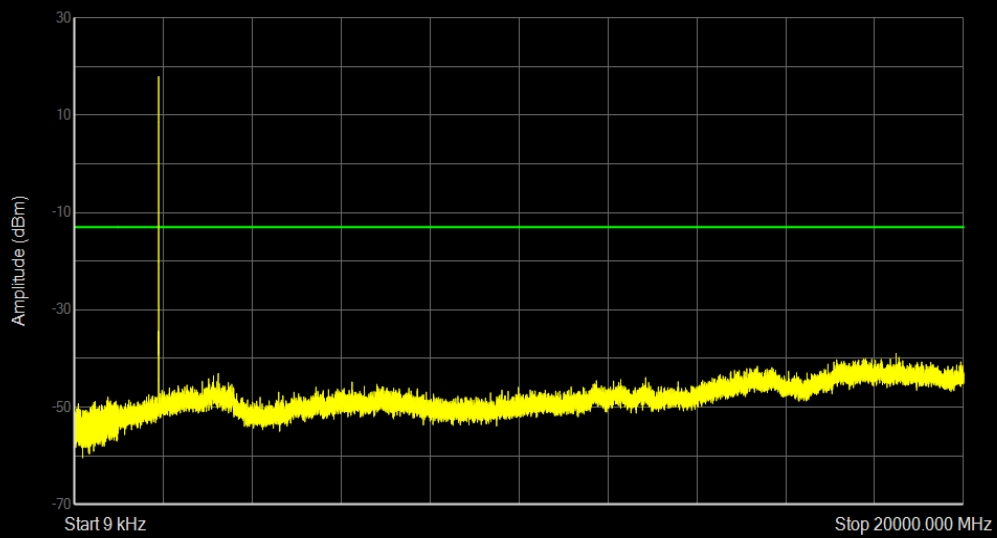
Band25 16QAM BW=3MHz Channel=26675 RB Size=1 Position=#0
