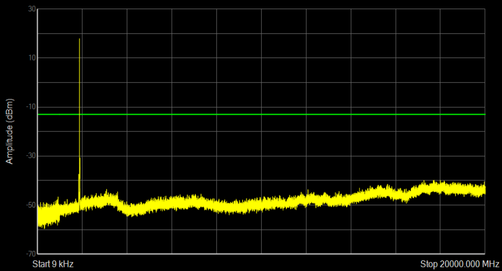
Band25 16QAM BW=20MHz Channel=26590 RB Size=1 Position=#0
