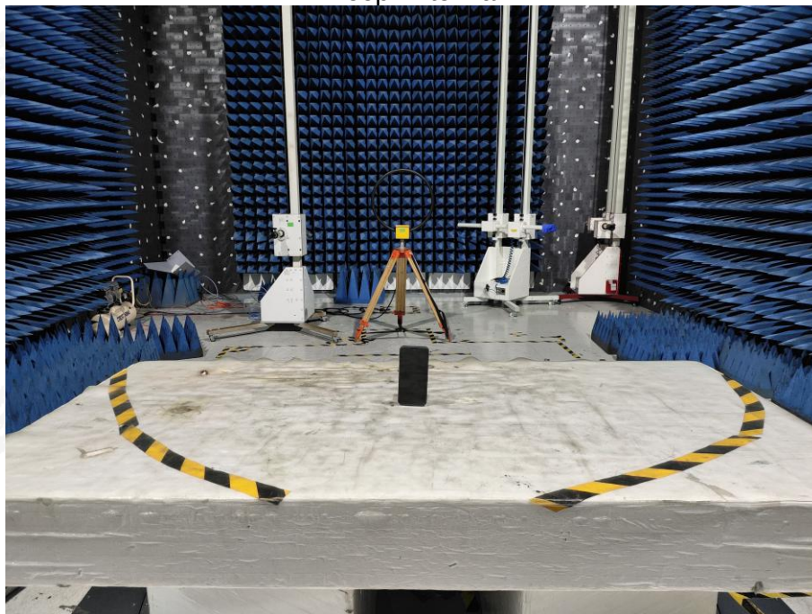
Loop Antenna
