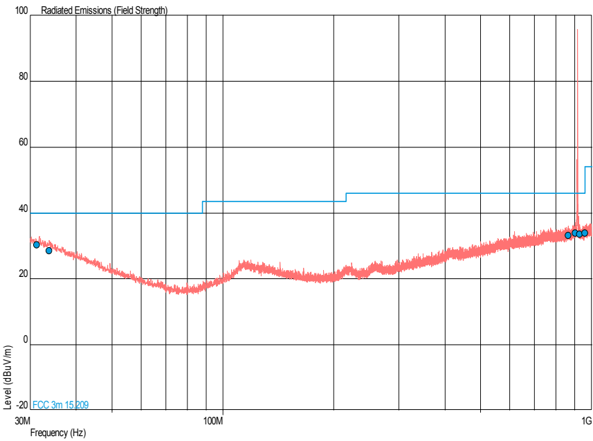
Figure 1 - 915.3 MHz - 30 MHz to 1 GHz
