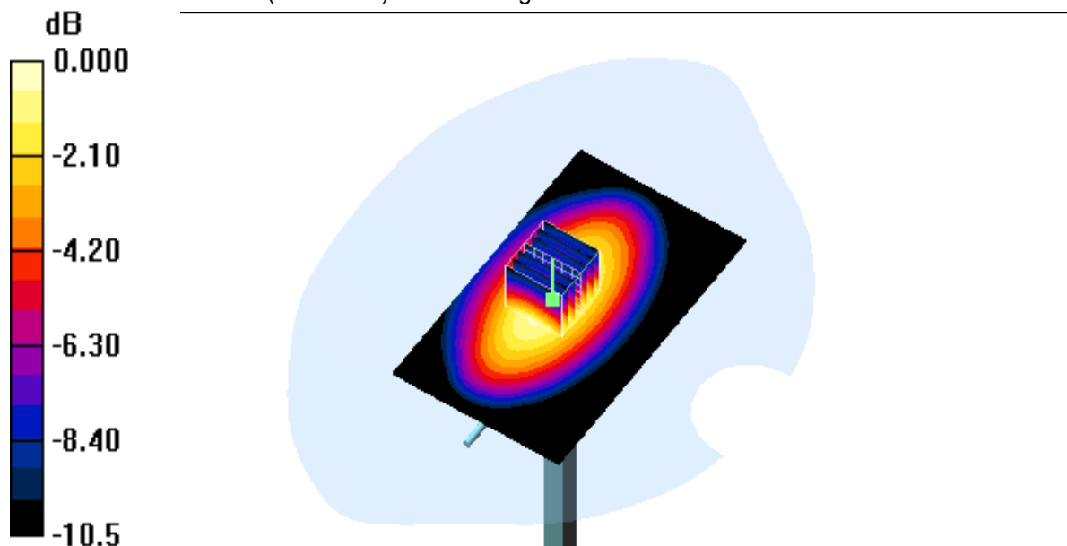
System Performance Check 835MHz Head 250 mW
