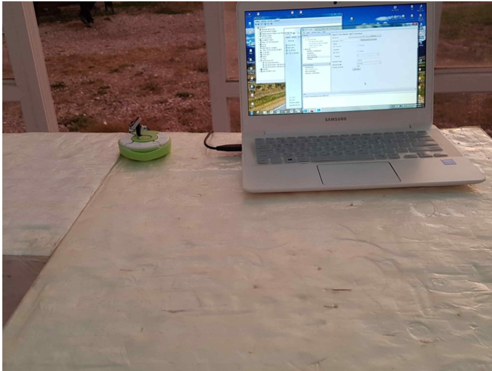
Radiated Emission Test (Above 1 GHz) Close-up of test setup
