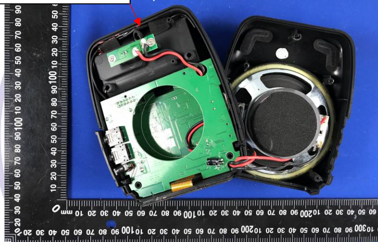
Wireless microphone receiver antenna
