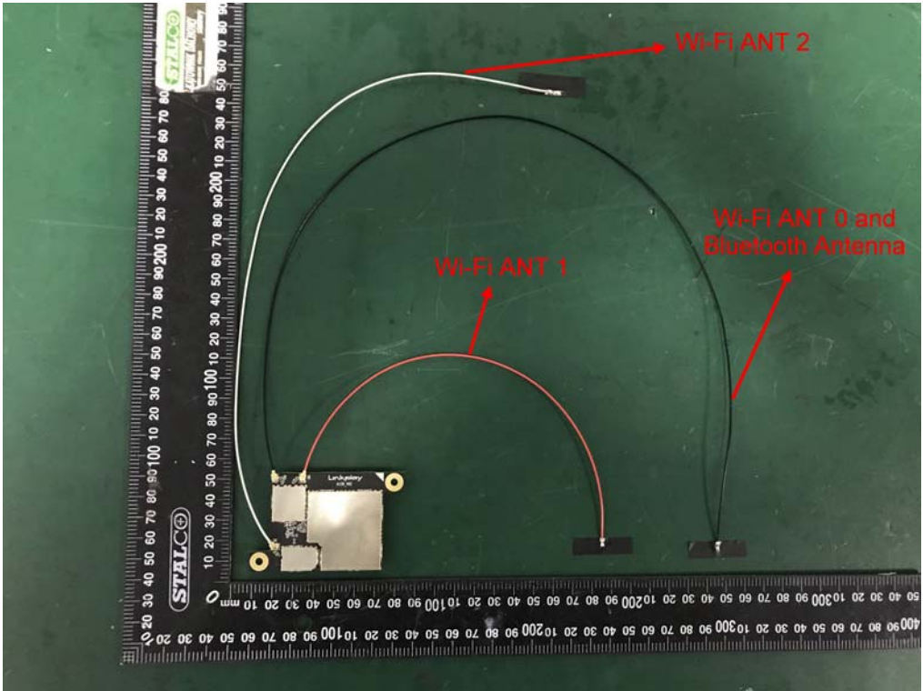
External Photos M/N: A128
