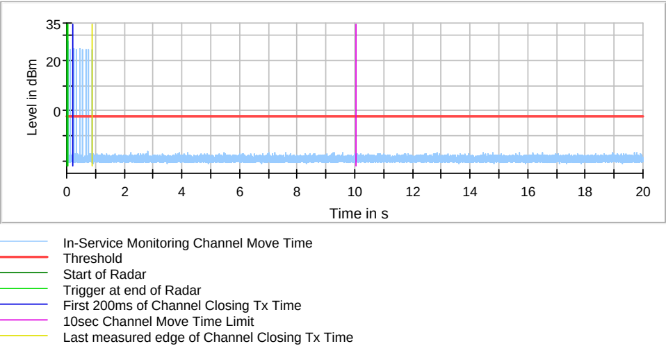
802.11a 5260 MHz_Ant 2
