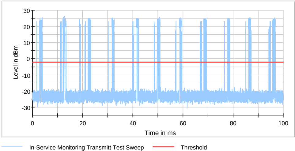
802.11a 5260 MHz_Ant 2
