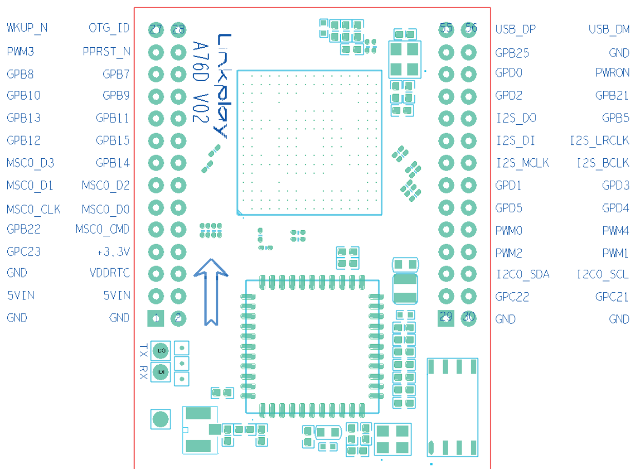
Figure 2-1 A76D interface pins
