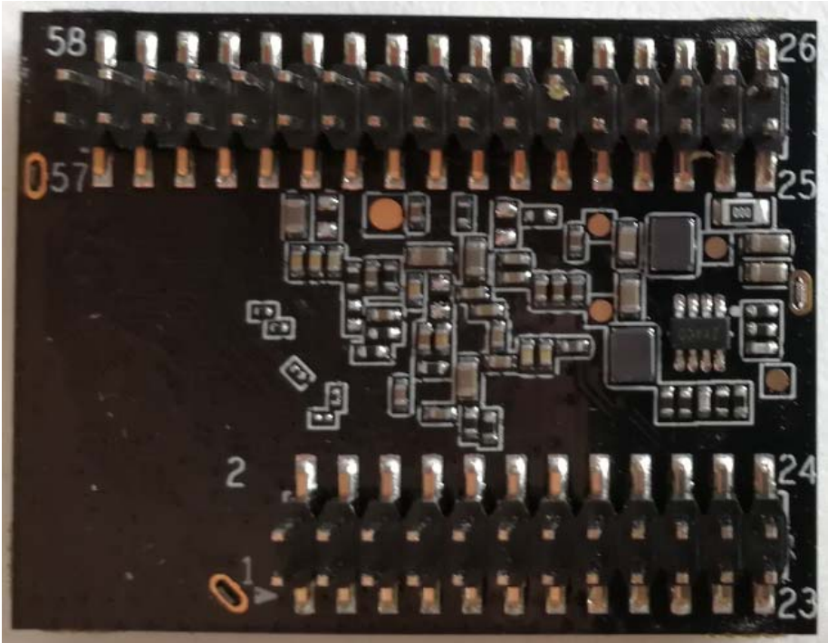
Figure 2- 8 Bottom View
