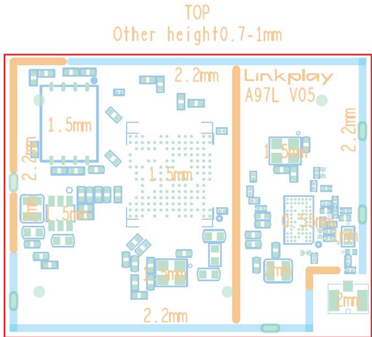
Figure 2-7 TOP Components Height
