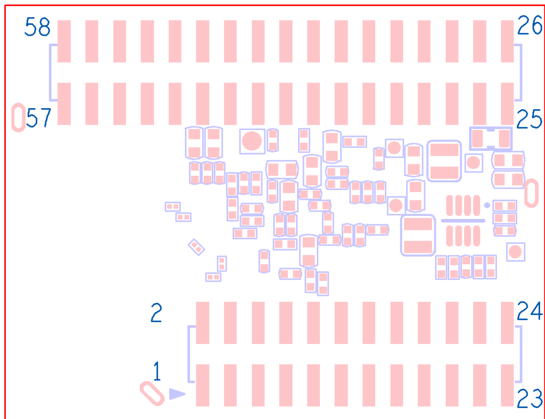
Figure 2-1 A97L interface pins
