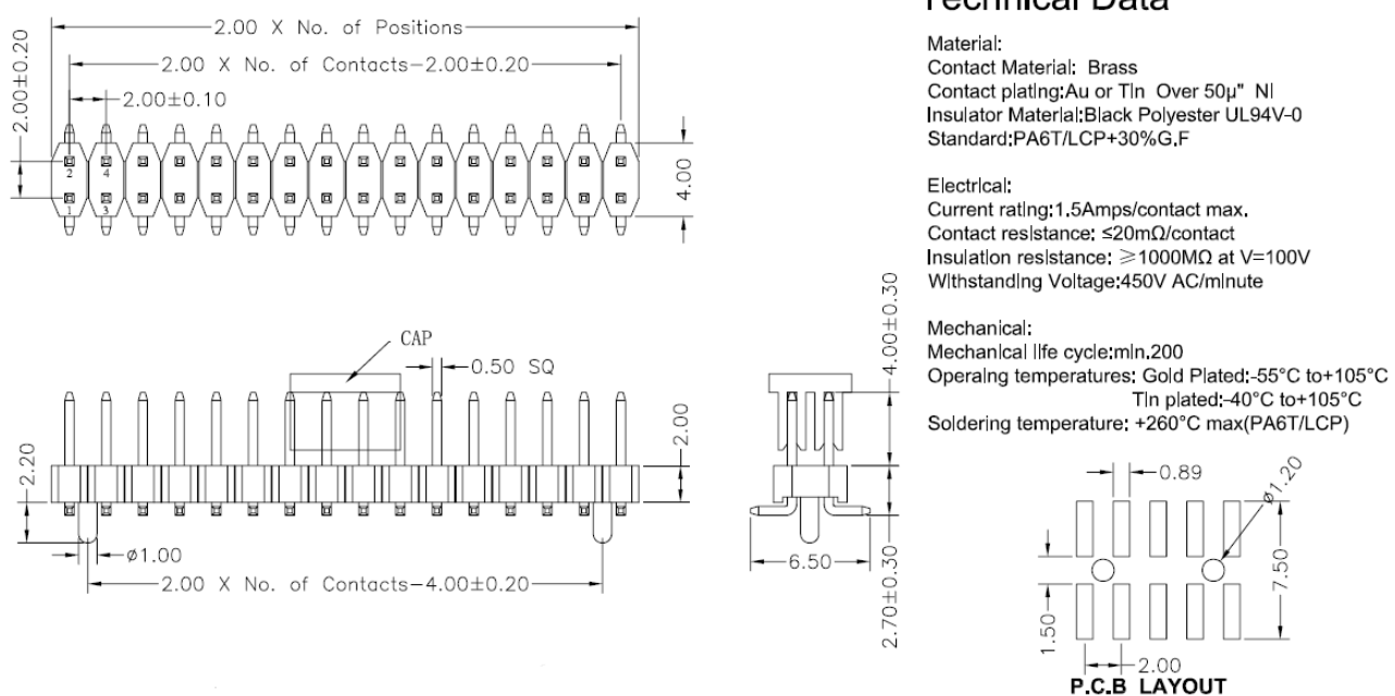
Figure 2-2 male connector dimensions
