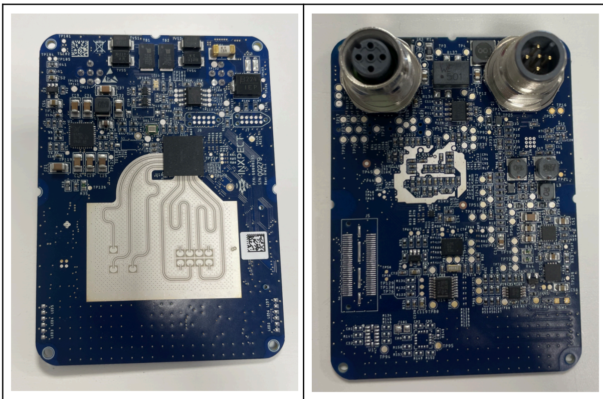
figure 2: top view (on the left) and bottom view (on the right) of the PCB
