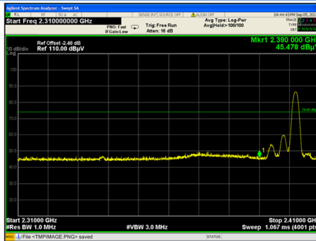
GFSK LOW CHANNEL , PEAK
