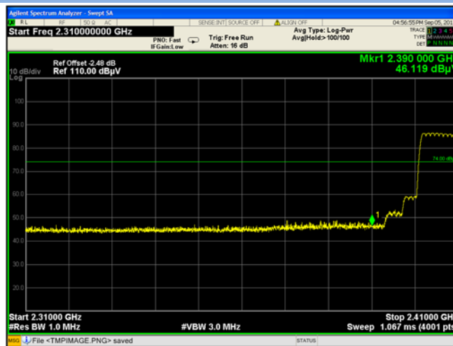
GFSK LOW FREQUENCY BAND, PEAK
