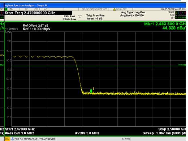
GFSK HIGH FREQUENCY BAND, PEAK
