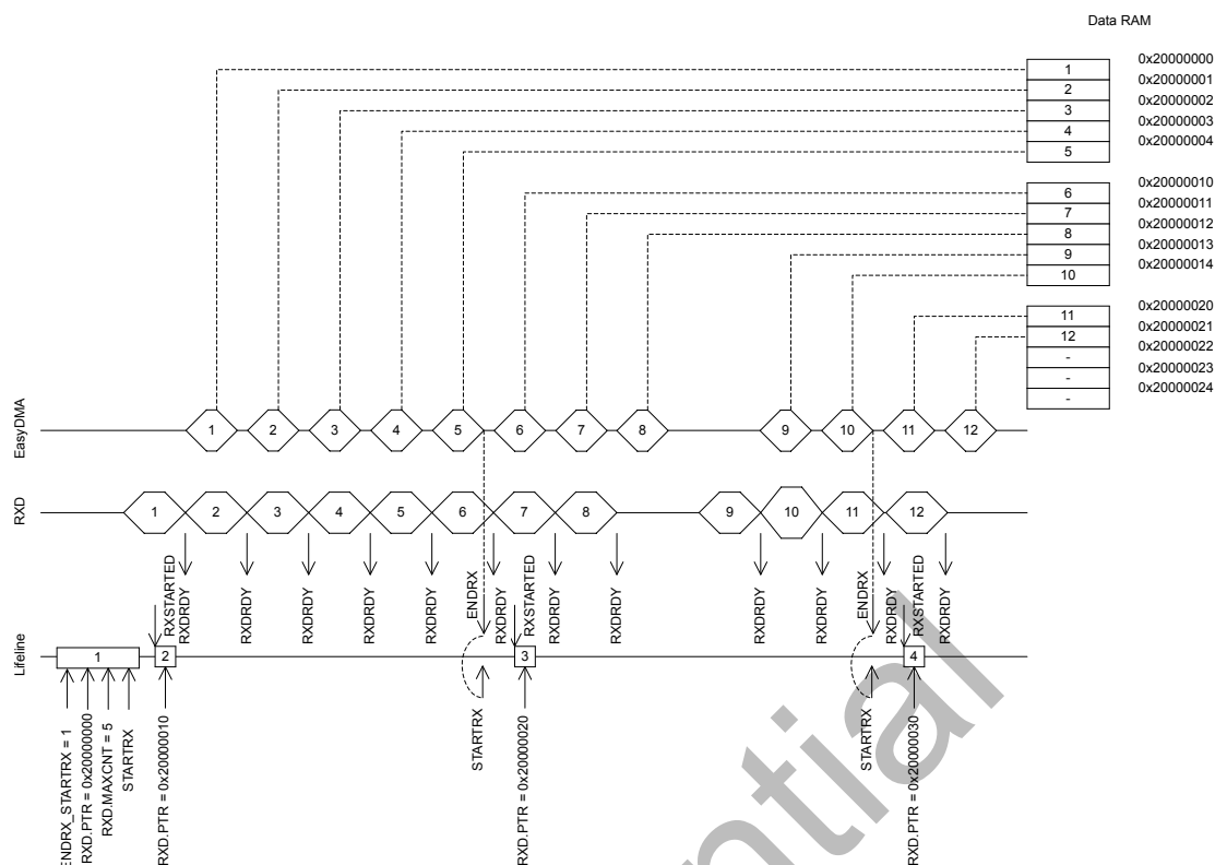
Figure 104: UARTe reception
