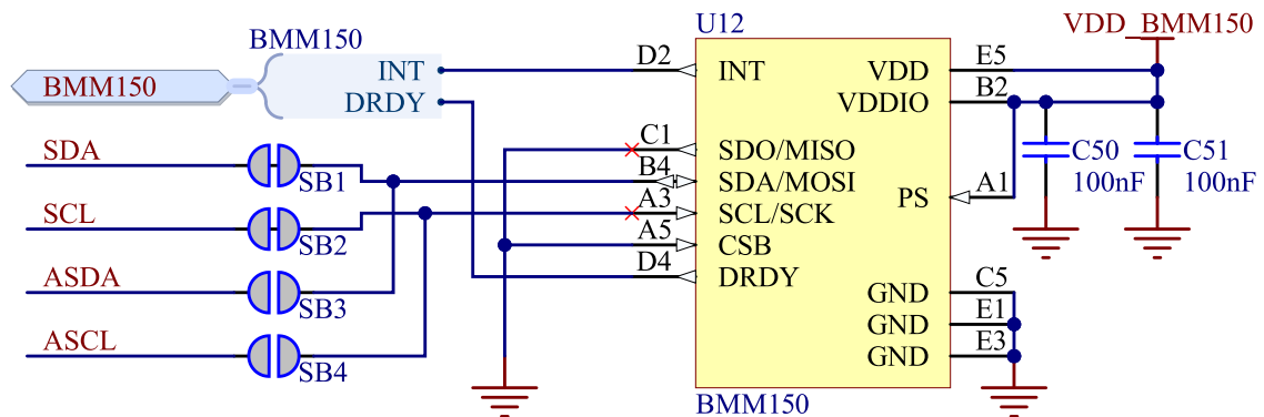
Figure 13: Magnetometer
