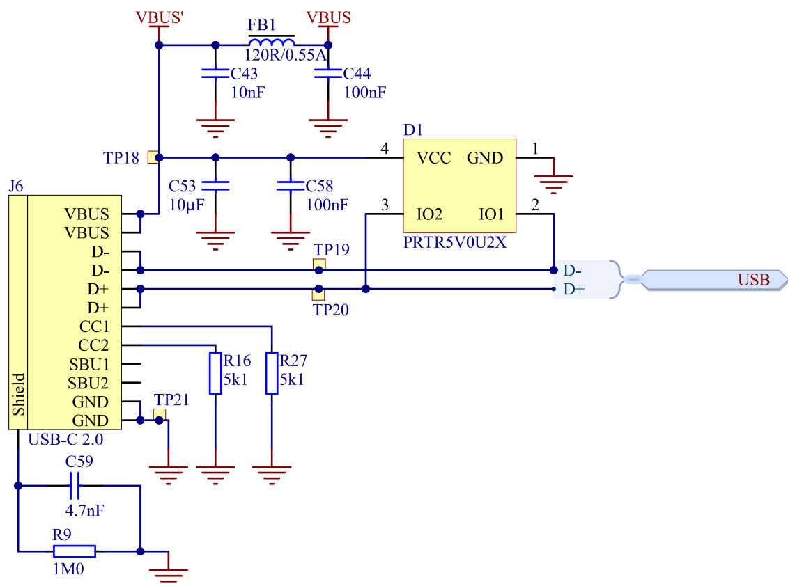
Figure 9: USB-C interface
