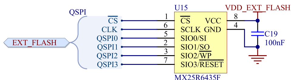
Figure 18: External memory
