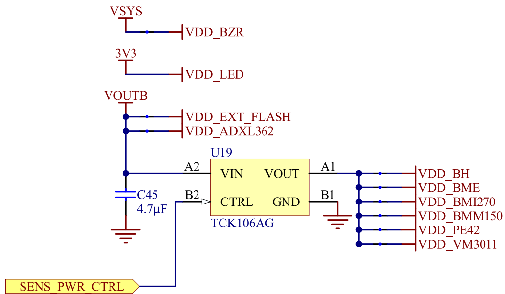
Figure 27: Sensor power control circuit
