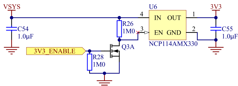
Figure 26: Regulator
