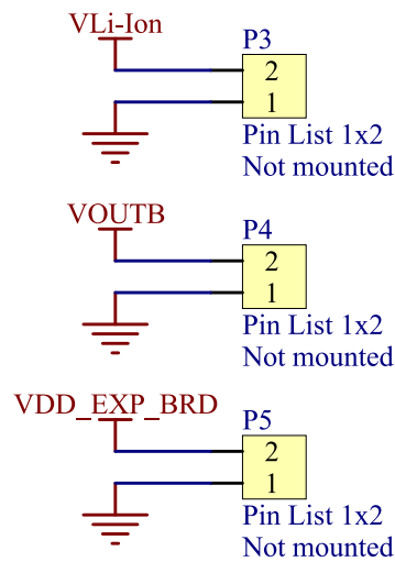
Figure 32: Power connectors
