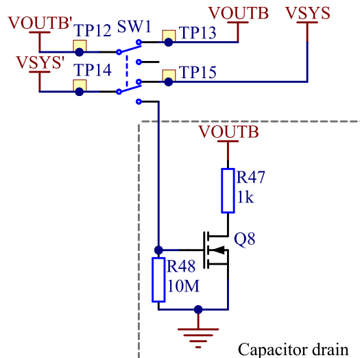
Figure 22: Power switch
