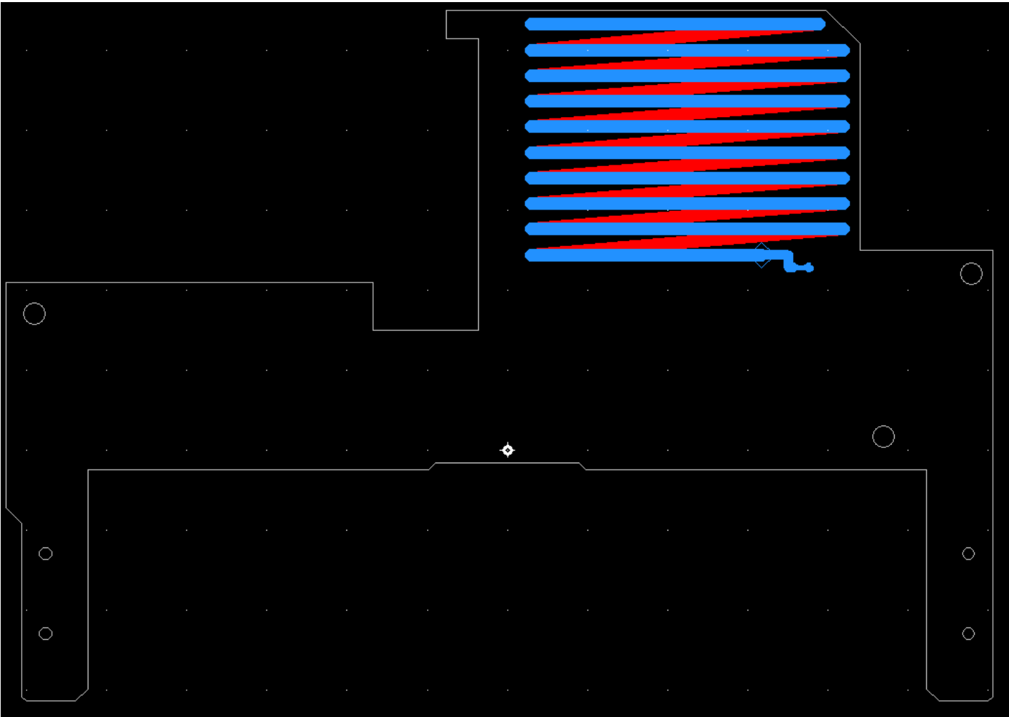
PCBAntenna drawing:
