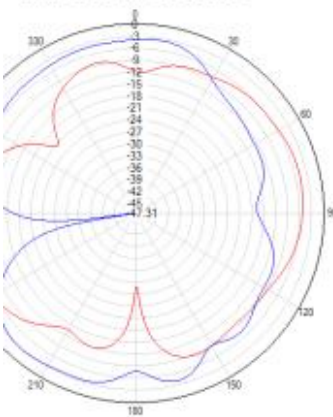
Phi=0 freq=2540MHz
