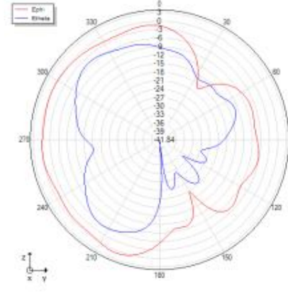
Phi=90 freq=2600MHz
