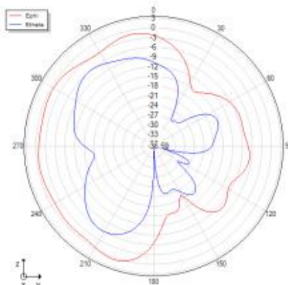
Phi=90 freq=2560MHz
