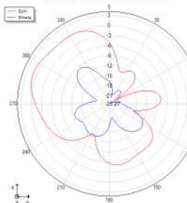
Theta=90 freq=2540MHz
