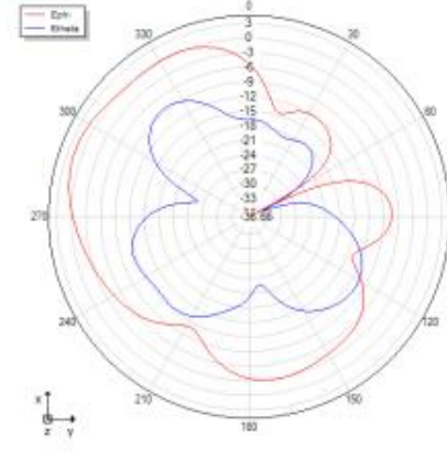
Theta=90 freq=2600MHz
