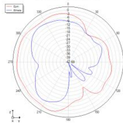
Phi=90 freq=2620MHz
