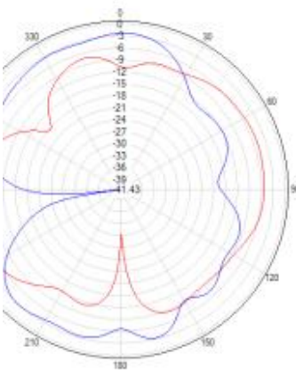
Phi=0 freq=2560MHz
