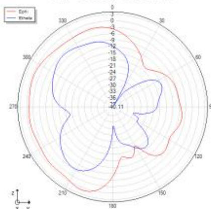
Phi=90 freq=2540MHz
