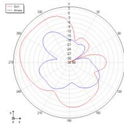
Theta=90 freq=2620MHz
