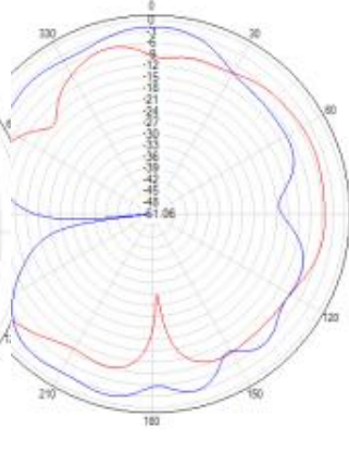
Phi=0 freq=2600MHz
