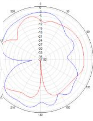
Phi=0 freq=2620MHz
