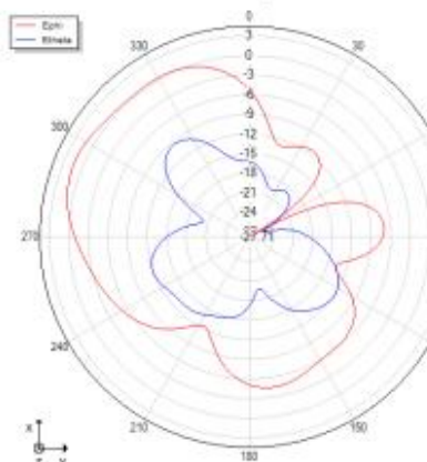
Theta=90 freq=2560MHz
